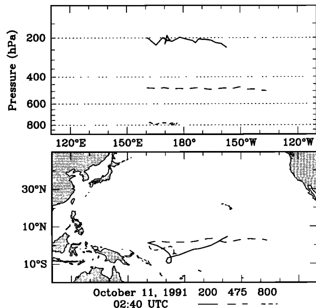
Figure 7. Backtrajectory analysis for 10 days starting from 1.3°N/161°E at 02:40 UT on October 11, 1991 (PWA flight 15), at 200 hPa (~12 km) (solid line), 475 hPa (~6 km) (long-dashed line), and 800 hPa (~2 km) (medium-dashed line).
