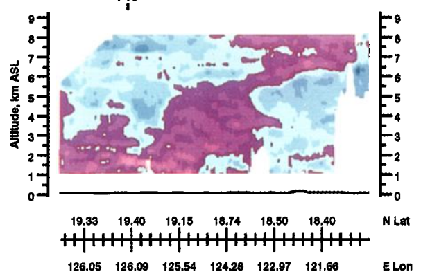
Plate 5. Aerosol and O 3 distributions associated with clean Pacific air and convective outflow observed near Taiwan on October 1, 1991 (PWA flight 10).
