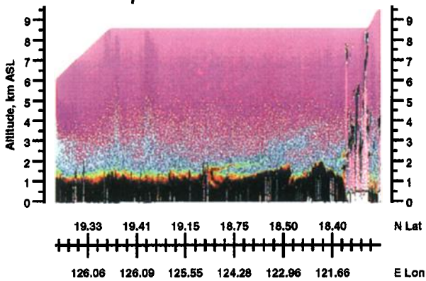
Plate 5. Aerosol and O 3 distributions associated with clean Pacific air and convective outflow observed near Taiwan on October 1, 1991 (PWA flight 10).
