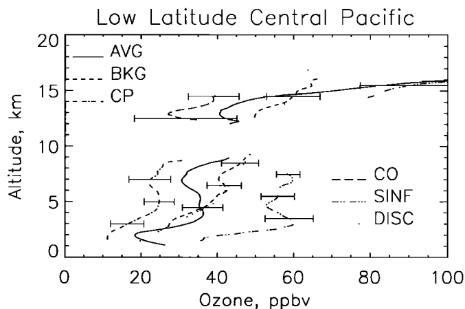
Figure 12. Average O 3 profile for low-latitude central Pacific (0°-20°N/150°E-160°W) region (solid line), and average O 3 profiles for background (medium-dashed line), clean Pacific (long-short-dashed line), and stratospherically influenced (long-short-short-short-dashed line) air masses relative to the reference O 3 profile, or discriminator (short-dashed line).
