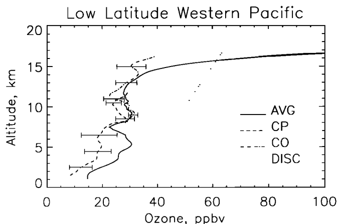
Figure 11. Average O 3 profile for western Pacific low latitude (0°-20°N/110°-150°E) region (solid line), and average O 3 profiles for clean Pacific (long-dashed line) and convective outflow (long-short-dashed line) air masses shown relative to the reference O 3 profile, or discriminator (short-dashed line).
