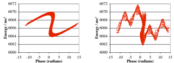
FIG. 7: Longitudinal phase space of a prebunched electron beam after harmonic generation at 50 nm. The low-current limit (left) is compared with the nominal case where the beam is modulated by its own radiation (right).
