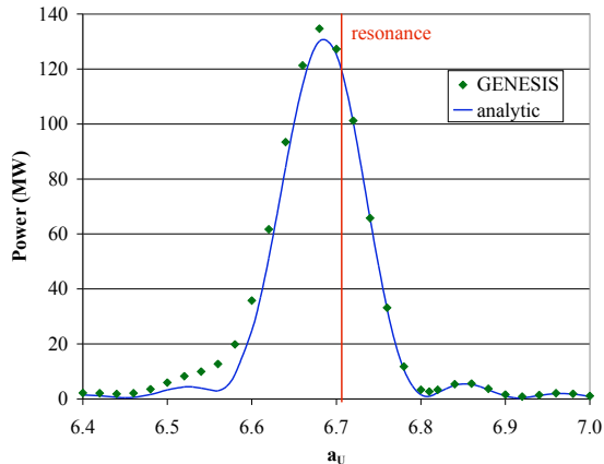
FIG. 5: Comparison of analytic theory with simulations using GENESIS. Results are shown for harmonic generation at 50 nm, as the undulator field strength ( a_u ) is varied.
