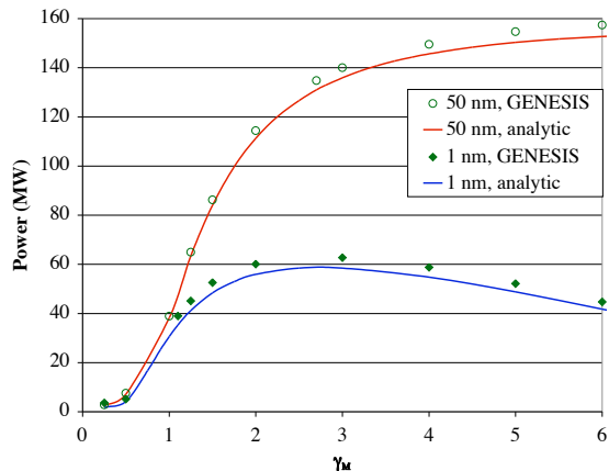
FIG. 2: Comparison of analytic theory with simulations using GENESIS. Results are shown for harmonic generation at 50 nm and 1.04 nm, as the energy modulation \gamma_M is varied.
