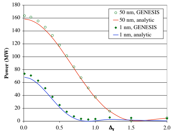
FIG. 3: Comparison of analytic theory with simulations using GENESIS. Results are shown for harmonic generation at 50 nm and 1.04 nm, as the energy spread \Delta_\gamma is varied.
