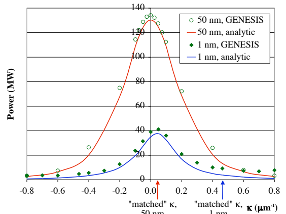
FIG. 4: Comparison of analytic theory with simulations using GENESIS. Results are shown for harmonic generation at 50 nm and 1.04 nm, as the conditioning parameter \kappa is varied. The “matched” values indicated refer to the ideal conditioning parameters for a different geometry, where the FEL output grows from noise, with no chicane.
