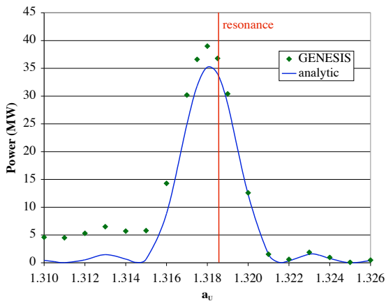
FIG. 6: Comparison of analytic theory with simulations using GENESIS. Results are shown for harmonic generation at 1.04 nm, as the undulator field strength ( a_u ) is varied.
