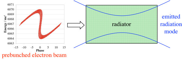
FIG. 1: A schematic of the FEL configuration chosen here, where a beam, which has a longitudinal distribution that is modulated at one wavelength, then passes through an undulator where it radiates into a harmonic wavelength.
