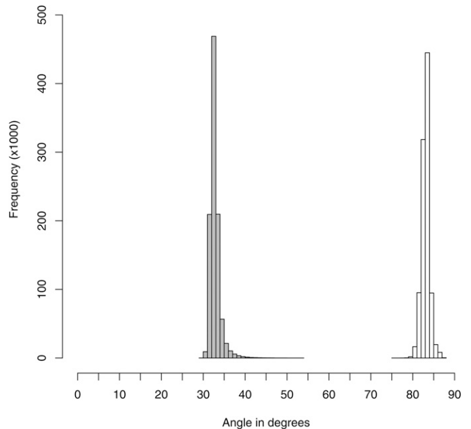
Figure 5 Angles between random selection gradients and the corresponding evolutionary response predicted by \mathbf{M} . The evolutionary responses predicted by the posterior samples of the observed data (open) and the randomized data sets (gray) are each plotted.
