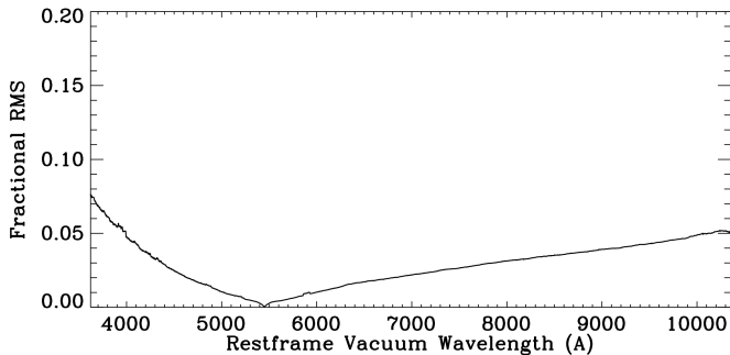
Figure 6. Fractional uncertainty in the spectra due to flux-calibration systematics, relative to 5450Å. This is derived using repeated observations of the same star. See the text for how it is produced.
