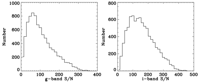
Figure 4. Distributions of median S/N per pixel for all the good per-visit spectra in the g -band (left) and the i -band (right).
