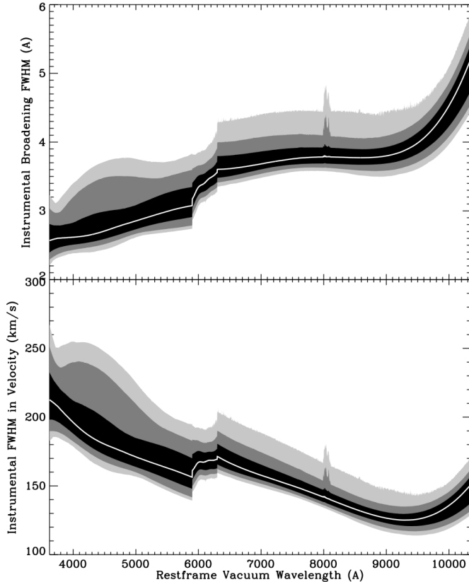
Figure 10. Distribution of the spectral resolution as a function of wavelength among all good per-visit spectra, in units of \text{\AA} (top panel) or \text{km/s} (bottom panel). The white lines indicate the median resolution, while the three different gray scales, from black to light grey, indicate zones of 68.3-, 95-, and 99.7-percentiles around the median, respectively
