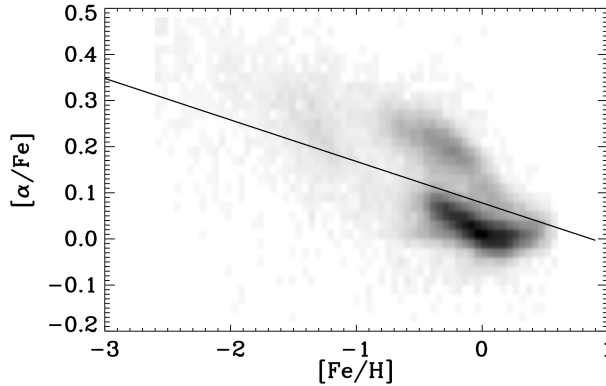
Figure 15. Distribution of APOGEE stars in [\alpha/\text{Fe}] vs. [\text{Fe}/\text{H}] space. One can see two sequences which merge at high [\text{Fe}/\text{H}] . These parameters have been adjusted according to the prescription in Section D.2. The solid line indicates our fiducial demarcation. We try to balance the sampling of stars above and below this demarcation.
