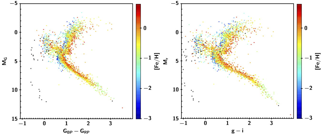
Figure 11. Extinction-corrected color-luminosity diagrams for a subset of the good stars in our library in the Gaia bandpasses (left) and the SDSS bandpasses (right). The subset is selected to be those with unique matches in Gaia DR2, and with either moderate extinction, with significant height above or below the plane of the Milky Way, or with a small distance from the Sun. The color-coding of points indicate metallicity estimates. Those with unknown metallicities are plotted in black.
