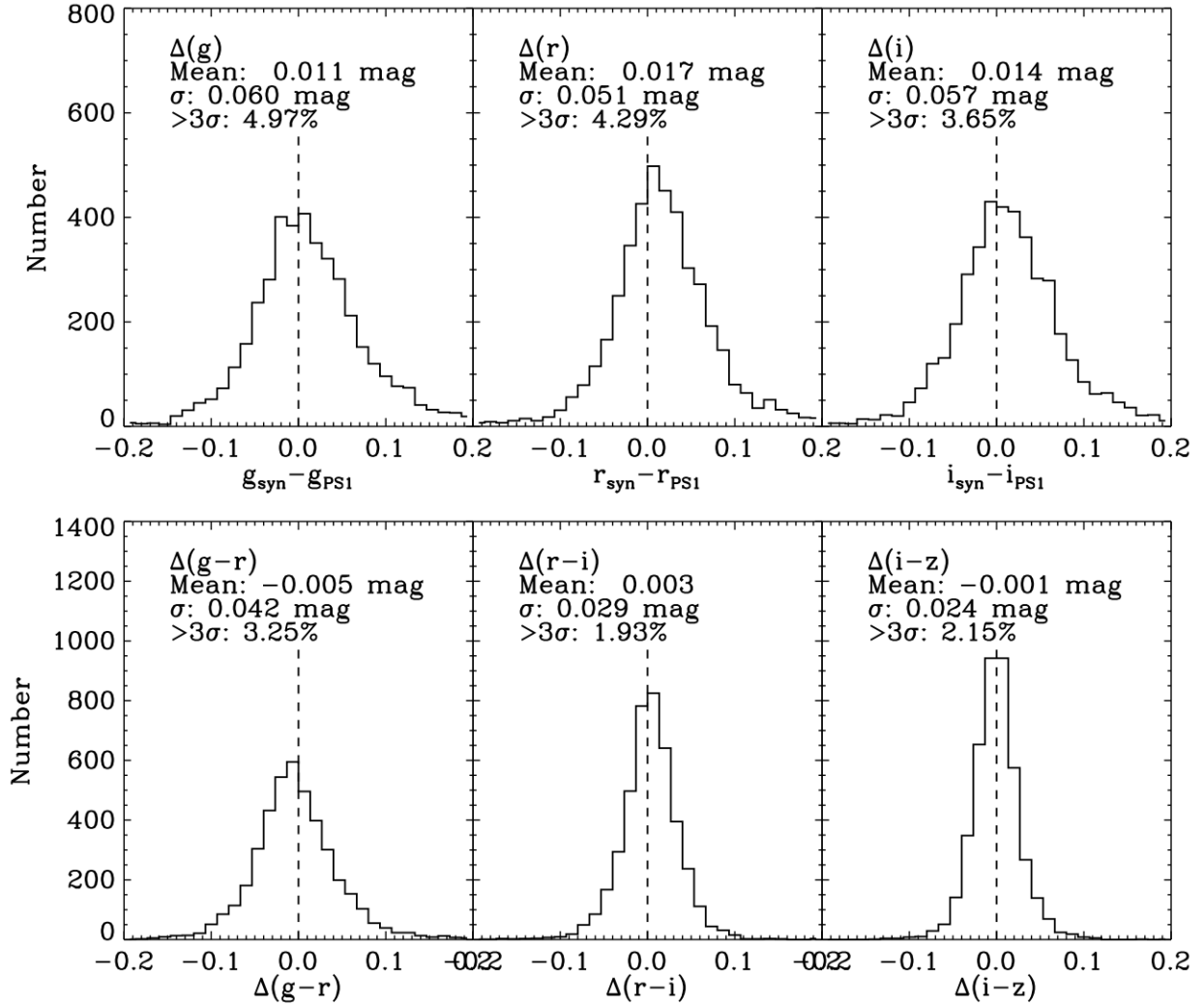
Figure 5. Top: histogram showing the difference in the g -, r -, and i -bands between synthetic magnitudes from MaStar and observed magnitudes from PS1 for our per-visit spectra. This shows our absolute calibration is 0.051 mag (4.7%) in the r -band. Bottom: histograms showing the difference in g-r , r-i , and i-z between synthetic color and the observed color in PS1, also for per-visit spectra. This shows that our relative calibration is 0.42 mag (3.9%) in g-r , 0.029 mag (2.7%) in r-i , and 0.024 mag (2.2%) in i-z . The fraction of outliers beyond 3\sigma are also given in the legend, which are generally around 2-3% for colors.
