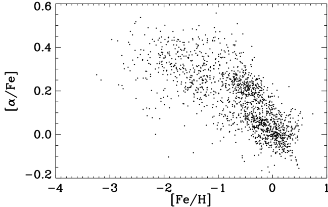
Figure 13. Distribution of half of the MaStar sample in the [\alpha/\text{Fe}] vs. [\text{Fe}/\text{H}] space. This only shows those stars with known [\alpha/\text{Fe}] and [\text{Fe}/\text{H}] values from input catalogs. The distribution here is much more uniform than shown in Figure 15.
