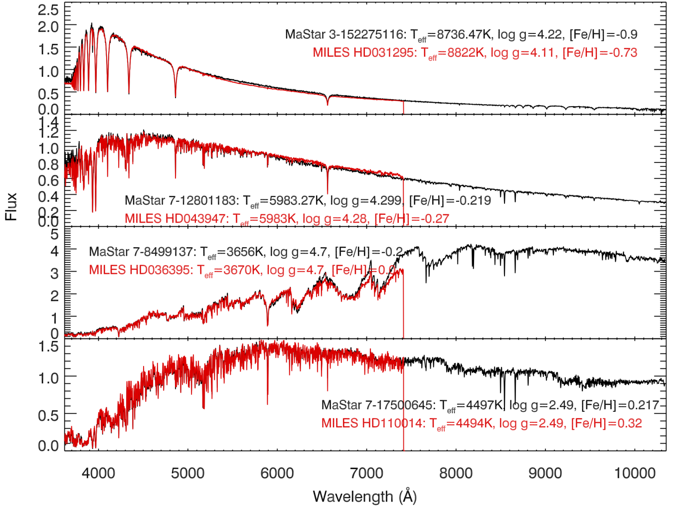
Figure 14. Comparison between MaStar spectra and MILES spectra for stars with similar parameters. From top to bottom, we show one hot main sequence star, one warm main sequence star, one cool main sequence star, and one red giant star. Both MaStar and MILES spectra are normalized by the median value between 5000Å and 5050Å. The wavelength are converted from vacuum to air to match MILES. The spectra agree well in general, with small differences in flux calibration.
