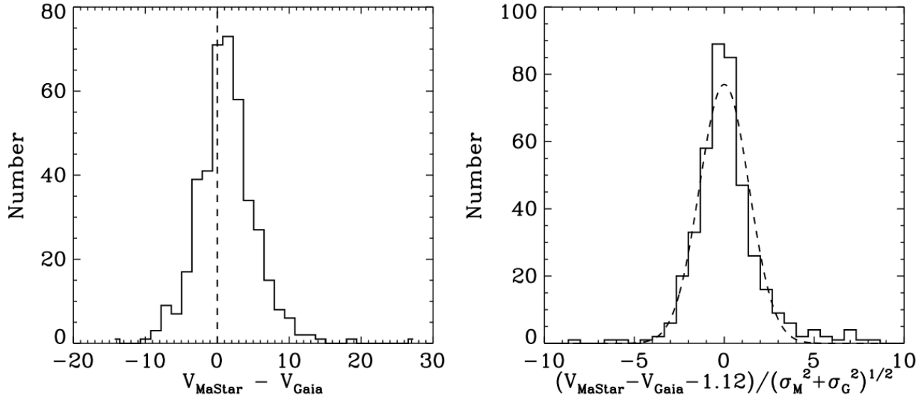
Figure 9. Left: Distribution of heliocentric radial velocity differences between MaStar and Gaia measurements for 417 stars that have good velocities from both sources. There is a 1.12 km/s systematic offset. The standard deviation is 3.68 km/s. Right: Distribution of the velocity difference (after removing the systematic difference) divided by the reported uncertainty. The Gaussian curve has a \sigma = 1.375 . This shows our velocity errors are slightly underestimated. The outliers beyond 3\sigma could be stars with genuine radial velocity variations.
