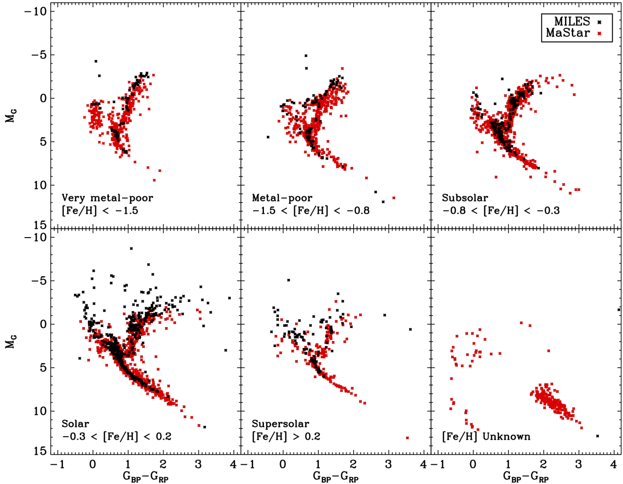
Figure 12. Comparison of the coverage in extinction-corrected color-luminosity diagrams between MILES (black) and MaStar (red) in 5 metallicity bins. The last panel is for stars with no or unreliable metallicity measurements. MaStar has much more extensive and more contiguous coverage for cool dwarfs, red giants, and low metallicity stars. The coverages of the two libraries in the super-Solar metallicity bin are very complementary to each other.
