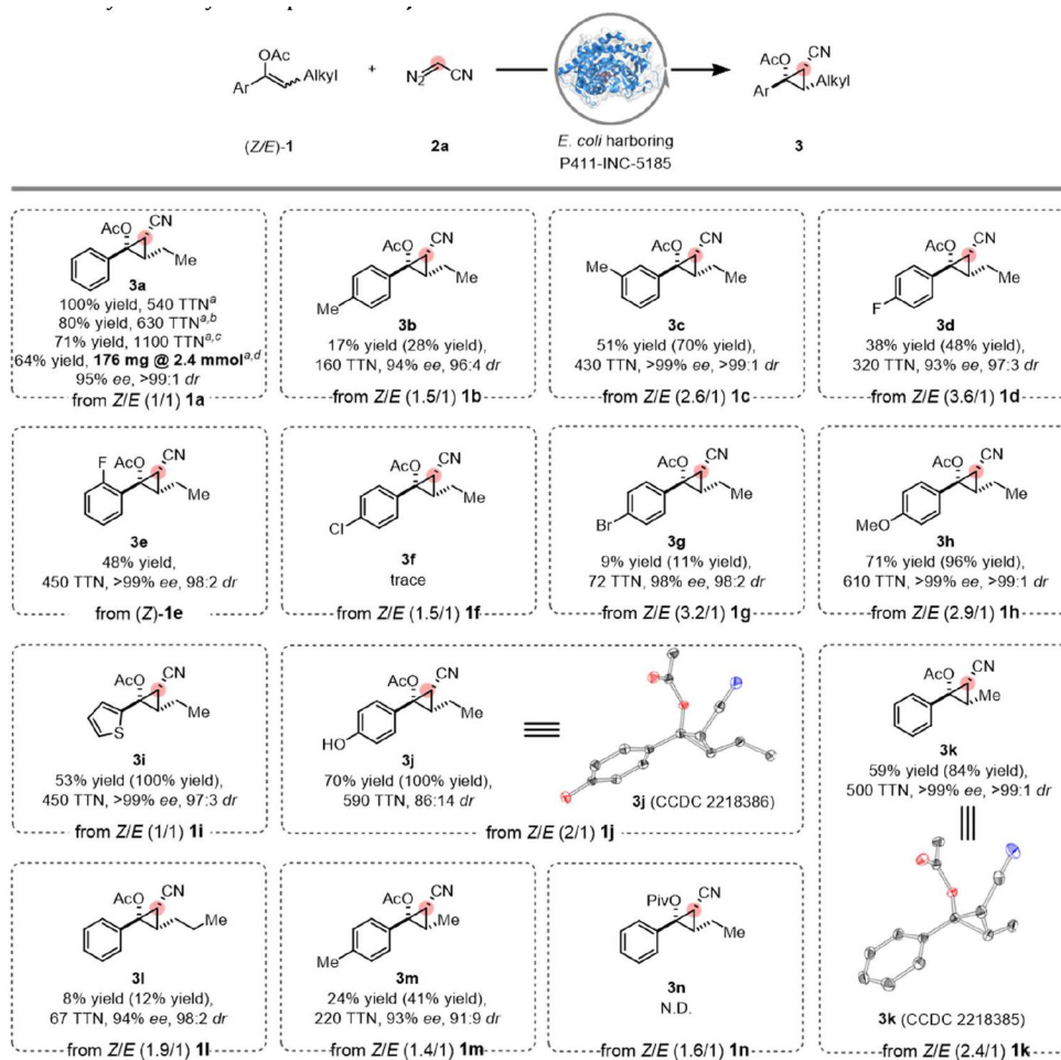
Figure 3. Substrate scope study.
