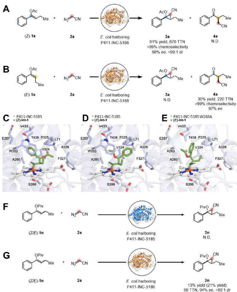
Figure 4. Discovery of the diastereomer-differentiating alkyl transferase P411-INC-5186 and its activity toward divergent alkyl transfer reactions.
