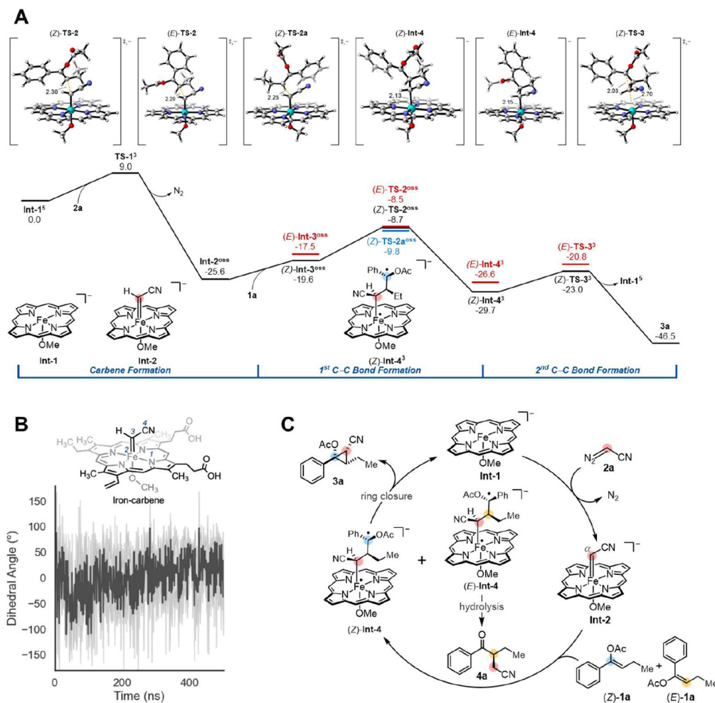
Figure 5. Proposed stepwise pathway for enantio- and diastereoenriched enzymatic cyclopropanation.
