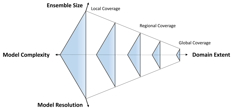
Fig. 3. A depiction of the allowed state space for modeling experiments given a prescribed limit on computational resources. Reducing the domain extent allows for more options for model resolution, ensemble size, and model complexity.
