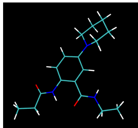
Figure S7. Model of Aa with truncated aliphatic chains used for the calculations described here.
