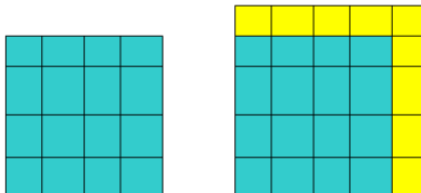
Figure 5: On the left is a domain without ghost elements. On the right is the same domain with ghost elements added (drawn in yellow). VisIt combines the ghost elements with the domain's real elements into one large domain for efficiency purposes for the filters downstream as well as simplicity of coding.
