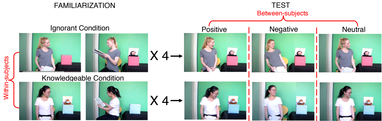
Figure 1 Experimental design
