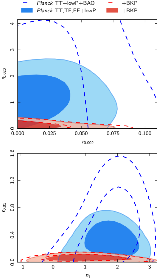
Fig. 57. 68% and 95% CL constraints on tensors when the inflationary consistency relation is relaxed, with Planck TT+lowP+BAO (blue dashed contours) and TT,TE,EE+lowP (blue shaded regions). The red colours are for the same data plus the BKP joint likelihood. The upper panel shows our independent primary parameters r_{0,002} and r_{0,020} . The lower panel shows the derived parameters n_t and r_{0,01} . The scale k = 0.01 \text{ Mpc}^{-1} is near the decorrelation scale of (n_t, r) for the Planck +BKP data.
