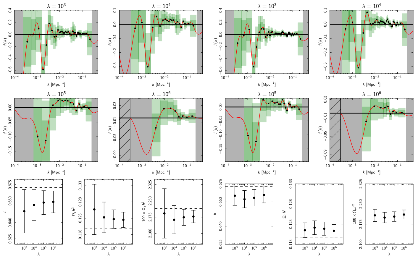
Fig. 21. Planck TT likelihood primordial power spectrum (PPS) reconstruction results. Top four panels: Reconstruction of the deviation f(k) using four different roughness penalties. The red curves represent the best-fit deviation f(k) using the Planck TT likelihood. f(k) = 0 would represent a perfectly featureless spectrum with respect to the fiducial PPS model, which is obtained from the best-fit base \Lambda CDM model with a power-law PPS. The vertical extent of the dark and light green error bars indicates the \pm 1\sigma and \pm 2\sigma errors, respectively. The width of the error bars represents the minimum reconstructible width (the minimum width for a Gaussian feature so that the mean square deviation of the reconstruction is less than 10%). The grey regions indicate where the minimum reconstructible width is undefined, indicating that the reconstruction in these regions is untrustworthy. The hatched region in the \lambda = 10^6 plot shows where the fixing penalty has been applied. These hashed regions are not visible in the other three reconstructions, for which \kappa_{\min} lies outside the range shown in the plots. For all values of the roughness penalty, all data points are within 2\sigma of the fiducial PPS except for the deviations around k \approx 0.002 \text{ Mpc}^{-1} in the \lambda = 10^3 and \lambda = 10^4 reconstructions. Lower three panels: \pm 1\sigma error bars of the three non-PPS cosmological parameters included in the maximum likelihood reconstruction. All values are consistent with their respective best-fit fiducial model values indicated by the dashed lines.
