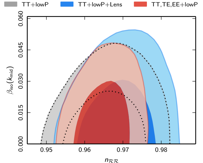
Fig. 50. Uncorrelated ADI+CDI with n_{\mathcal{I}\mathcal{I}} = 1 (“axion”).
