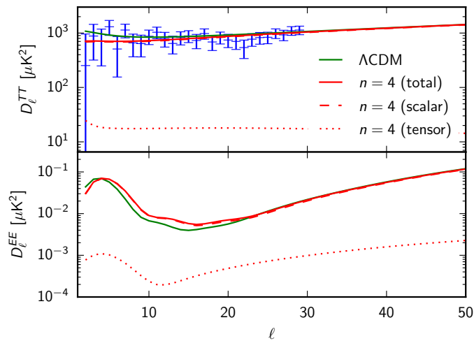
Fig. 18. Temperature spectrum (total, scalar contribution, tensor contribution) of the best-fit V(\phi) model with n = 4 , for the Planck TT,TE,EE+lowP data set, compared to the temperature spectrum (scalar contribution only) of the best-fit base model. We also show the Planck low- \ell temperature data, which is driving the small differences between the two best-fit models.
