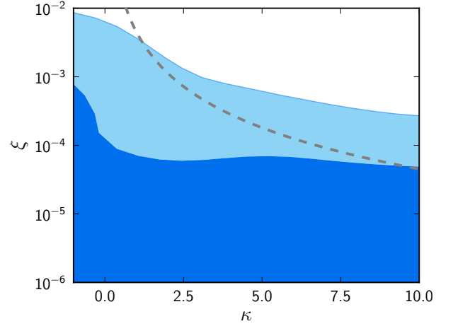
Fig. 53. 68 % and 95 % CL regions in the modulated isocurvature model parameter space using the Planck temperature data up to \ell_{\text{max}} = 1000 (contours). The region above the dashed curve is ruled out by the Planck constraint on an uncorrelated, scale-invariant isocurvature component.
