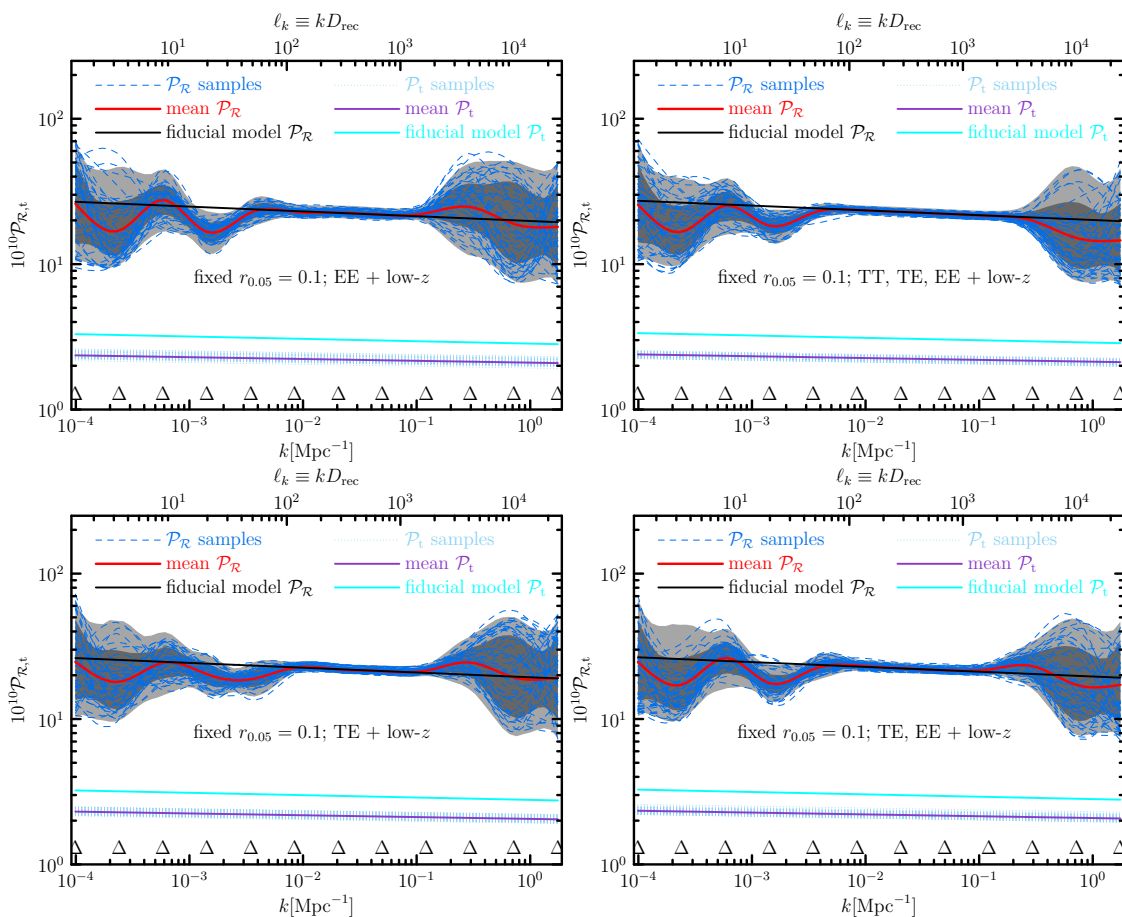
Fig. 28. Reconstructed 12-knot power spectra with polarization included. Data sets in common: lowP+BAO+SN+HST+ z_{re}>6 prior.
