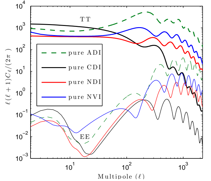
Fig. 42. Angular power spectra for the scale invariant (i.e., n_{RR} = 1 ) pure adiabatic mode (ADI, green dashed curves) and for the scale invariant ( n_{II} = 1 ) pure isocurvature (CDI, NDI, or NVI) modes, with equal primordial perturbation amplitudes. The thick lines represent the temperature auto-correlation ( TT ), and the thin lines the E mode polarization auto-correlation ( EE ).
