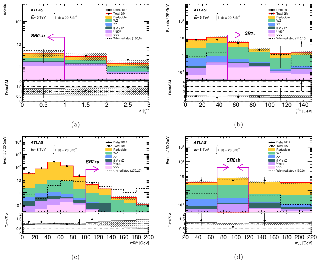
Figure 6. Expected distributions of SM background events and observed data distributions for (a) \Delta\phi_{\ell\ell'}^{\min} , (b) E_T^{\text{miss}} , (c) m_{T2}^{\max} and (d) m_{\tau\tau} variables in the SR0 \tau b, SR1 \tau , SR2 \tau a and SR2 \tau b regions respectively, prior to the requirements on these variables. Arrows indicate the limits on the values of the variables used to define the signal regions. Also shown are the respective contributions of the various background processes as described in the legend. Both the statistical and systematic uncertainties are shown. The last bin in each distribution includes the overflow. The plots also show the distribution for signal hypotheses, where the parentheses following the simplified model denote the mass parameters in GeV as (m(\tilde{\chi}_1^\pm, \tilde{\chi}_2^0), m(\tilde{\chi}_1^0)) .
