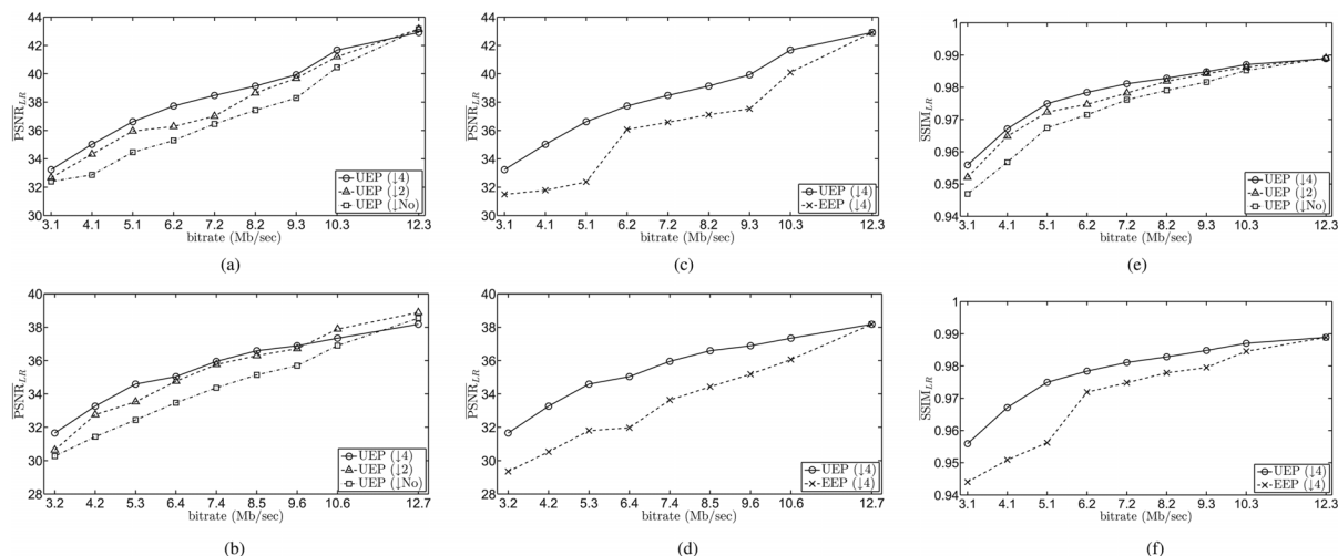
Fig. 5. (a)-(b) \overline{\text{PSNR}}_{LR} for scenarios \downarrow \text{No} , \downarrow 2 , and \downarrow 4 , (c)-(d) \overline{\text{PSNR}}_{LR} of UEP and EEP for scenario \downarrow 4 , (e) \overline{\text{SSIM}}_{LR} for scenarios \downarrow \text{No} , \downarrow 2 and \downarrow 4 , and (f) \overline{\text{SSIM}}_{LR} of UEP and EEP for scenario \downarrow 4 .
