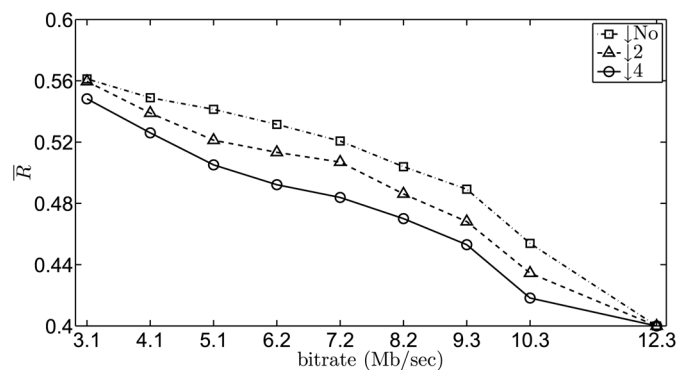
Fig. 4. \bar{R} for \downarrow No, \downarrow 2, and \downarrow 4 scenarios for a flat Rayleigh fading channel with SNR = 8 dB and T_c = 4000 .
