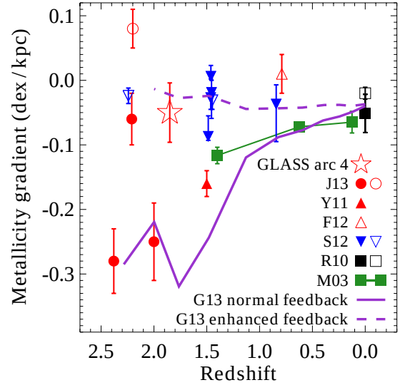
FIG. 7.— Evolution of metallicity gradients with redshift. We compare the gradient of arc 4 from this work with published measurements at high redshift including other lensed galaxies (Jones et al. 2013, J13; Yuan et al. 2011, Y11; Frye et al. 2012, F12), non-lensed galaxies observed with adaptive optics (Swinbank et al. 2012, S12), an average of local gradients reported by Rupke et al. (2010b, R10), and the Milky Way’s metallicity gradient evolution measured from planetary nebulae (Maciel et al. 2003, M03). Solid and hollow symbols denote isolated disks and interacting (or merging) galaxies, respectively, to show that interacting galaxies have flatter gradients (closer to zero) on average in the lensed and z = 0 samples. We additionally show results of two different feedback schemes in otherwise identical simulations, described in (Gibson et al. 2013, G13; the galaxy shown is g15784). The standard feedback results are similar to the Milky Way and isolated lensed galaxies, while enhanced feedback leads to shallower gradients at high redshifts and is good agreement with the measurement of arc 4 in this work.
