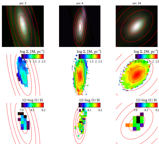
FIG. 4.— Source plane morphologies of arcs 3, 4, and 14 (from left to right). Each panel shows contours of constant de-projected galactocentric radii at intervals of 1 kpc, derived in Section 5. Top row : HST image (RGB: WFC3/F160W, WFC3/F110W, ACS/F814W). Middle : stellar mass maps derived from spatially resolved HST photometry. All galaxies have smooth, centrally peaked stellar mass profiles with no significant secondary peaks. Bottom : gas-phase metallicity maps.
