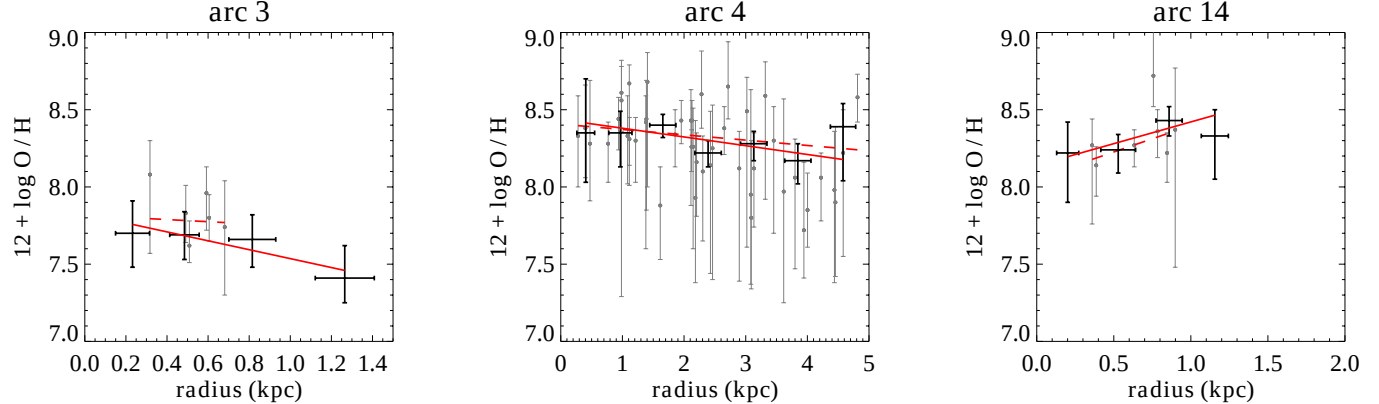
FIG. 5.— Radial metallicity gradients in each galaxy. Grey points are measured from individual source plane pixels shown in Figure 4, and thick black points show the results for flux summed within radial annuli. Linear gradient fits to the individual pixels and radial bins are shown as dashed and solid lines, respectively. Both methods give consistent results.
