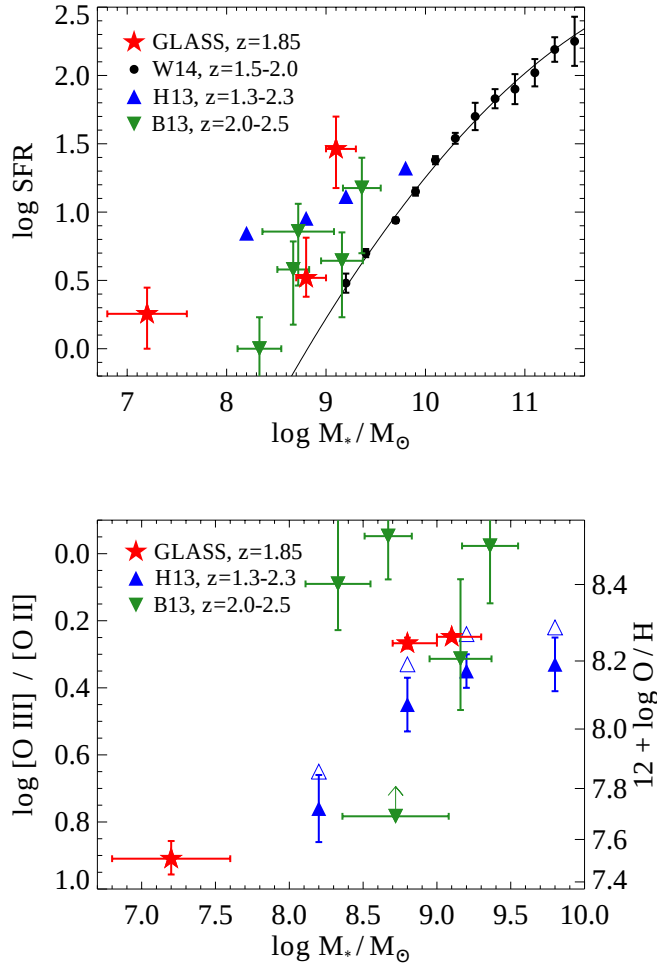
FIG. 6.— Global demographic properties of the GLASS arcs. For comparison we also show average values of larger samples at similar redshift from WISP (Henry et al. 2013, H13) and 3D-HST (Whitaker et al. 2014, W14) data as well as individual lensed galaxies reported by Belli et al. (2013, B13). Top : SFR versus stellar mass. The arcs studied here have significantly higher specific SFR compared to the “main sequence” at z \simeq 1.8 (shown by the W14 data), consistent with expectations for excess star formation triggered by gravitational interactions among these systems. Bottom : comparison of emission line ratios versus stellar mass. Open symbols show the effect of dust attenuation measured by Henry et al. (2013); all other data are uncorrected for reddening. The arcs studied here have typical [\text{O III}]/[\text{O II}] ratios for their redshift, stellar mass, and SFR. The right axis shows equivalent metallicity corresponding to [\text{O III}]/[\text{O II}] for the Maiolino et al. (2008) calibration used in this work. The GLASS data are consistent with a steep mass-metallicity relation as found by Henry et al. (2013), and notably extend to an order of magnitude lower in stellar mass compared to previous studies at z \simeq 2 .
