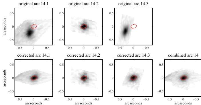
FIG. 3.— Demonstration of the lens model corrections. The panels in the top row are source plane reconstructions given by the original Sharon version 2 model, whereas those in the bottom row show the improved reconstructions after our correction is applied. Note that the original and corrected arc 14.2 is identical since it is used as a reference. In all panels, the gray scale represents the surface brightness contrast and the red contour shows an isophotal radius measured for the combined arc. Here we show the process for arc 14 as an illustration. The corrections for arcs 3 and 4 give similar results.
