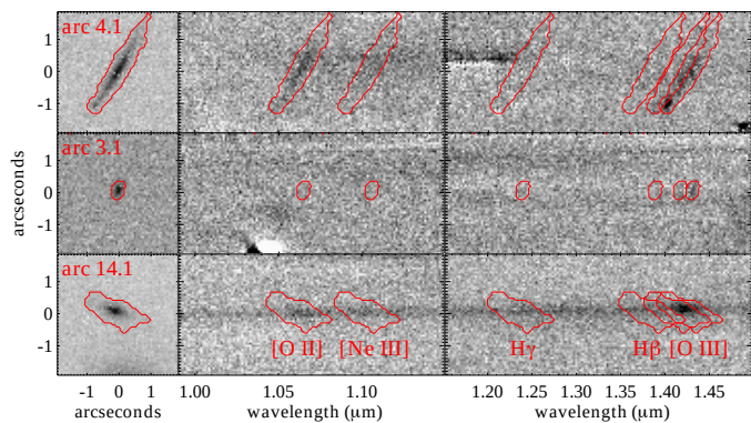
FIG. 1.— Grism spectra for the arcs of interest show multiple spatially extended emission lines which can be used to derive metallicity maps. From left to right, each row shows the F140W direct image, G102 grism spectrum, and G141 grism spectrum. In all cases the estimated contamination has been subtracted from the spectra. Strong source continuum is apparent for arc 14.1. Red contours show the object segmentation maps derived using the direct images, and mapped to emission lines of interest in the grism spectra using the redshift of each source (left to right: [O II] \lambda\lambda 3727 , [Ne III] \lambda 3869 , H\gamma , H\beta , [O III] \lambda 4959 , [O III] \lambda 5007 ). The redshift is z = 1.855 for all cases shown here.
