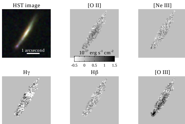
FIG. 2.— HST image (top left; RGB: WFC3/F160W, WFC3/F110W, ACS/F814W) and emission line maps of arc 4.1. The typical flux uncertainty in each pixel is 2 \times 10^{-18} \text{ ergs s}^{-1} \text{ cm}^{-2} ( 1\sigma ).
