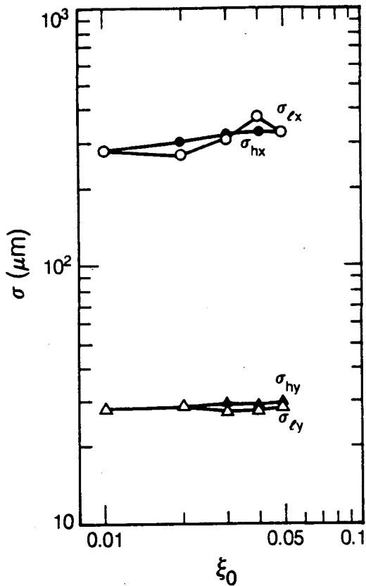
Fig. 5 RMS beam sizes when all four criteria are satisfied.
