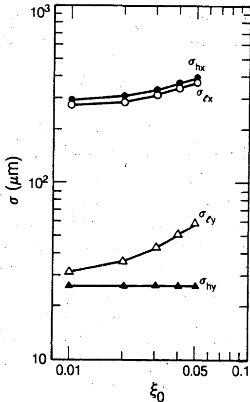
Fig. 3 RMS beam sizes when the two rings have the same damping decrement.
