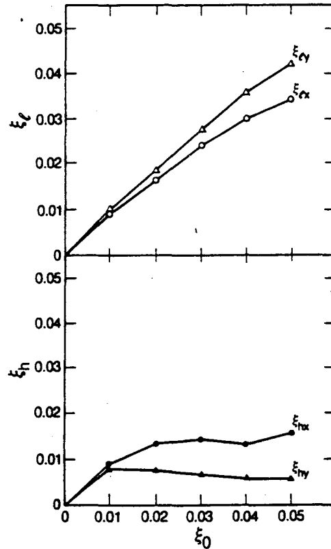
Fig. 2 Dynamic beam-beam parameters, \xi , as a function of \xi_0 for the original APIARY-I lattice.
