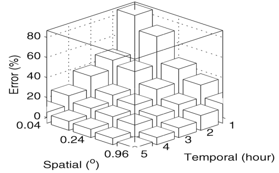
Figure 3. Satellite-based rainfall estimation error distribution as a function of spatial and temporal resolution without consideration of rain intensity.
