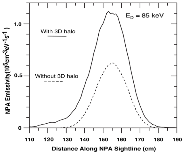
Figure 9. Comparison of the charge exchange neutral emissivity for the E||B NPA sightline with and without 3D halo neutrals.
