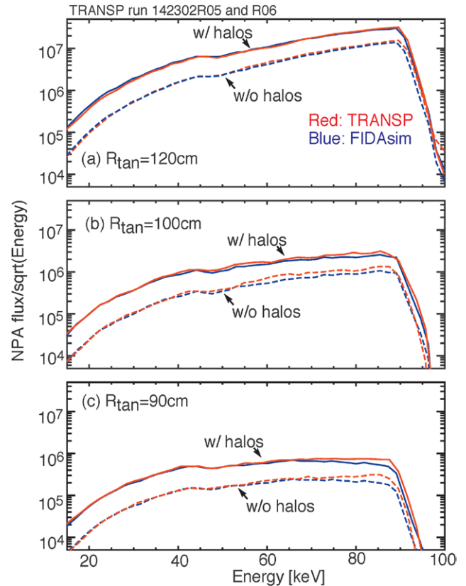
Figure 19. Comparison of NPA energy spectrum at t = 2.5 s with and without halo neutrals for the NPA sightlines captioned in (a), (b) and (c). The TRANSP simulation results are shown in red and the FIDASim simulation results are plotted in blue. The TRANSP and FIDASim simulation results overlap with each other.
