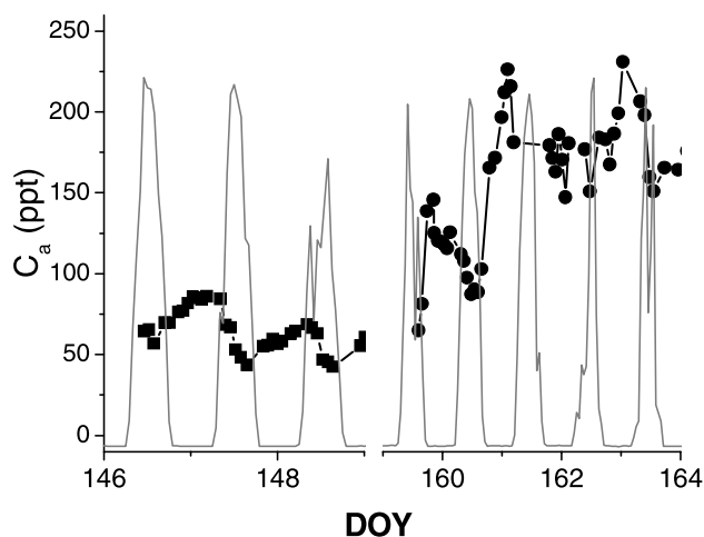
Figure 11. Atmospheric mixing ratios of DMS (solid squares and circles) shown with measured solar irradiation (shaded line) used to calculate air/sea flux of DMS from the nighttime buildup of DMS.
