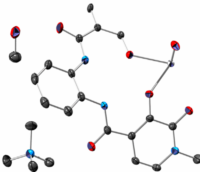
Figure A3-2. Asymmetric unit in the crystal structure of \text{UO}_2[\text{TAM}(o\text{-phen-Me-3,2-HOPO})_2] , \text{UO}_2(\mathbf{3-5}) . Tetramethylammonium cation and methanol inclusion included. Hydrogen atoms have been omitted for clarity. Thermal ellipsoids are drawn at the 50% level. Carbons are gray, oxygens red, nitrogens blue, and uranium silver.
