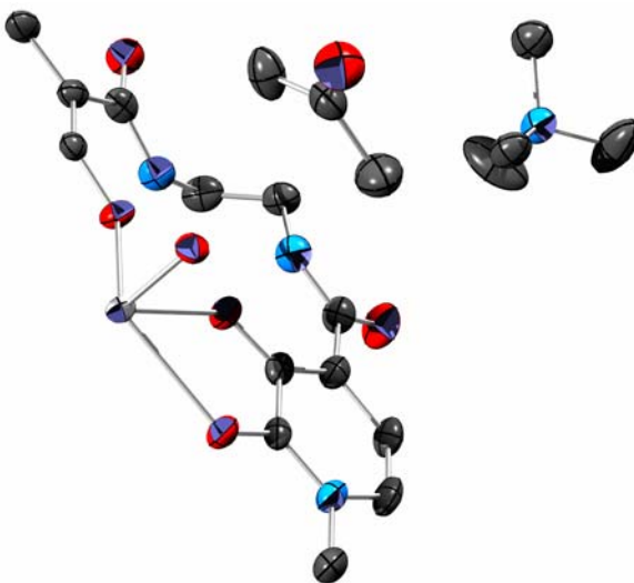
Figure A3-1. Asymmetric unit in the crystal structure of \text{UO}_2[\text{TAM}(2\text{Li-Me-3,2-HOPO})_2] , \text{UO}_2(\mathbf{3-2}) . Tetramethylammonium cation and acetone inclusion are included. Hydrogen atoms have been omitted for clarity. Thermal ellipsoids are drawn at the 50% level. Carbons are gray, oxygens red, nitrogens blue, and uranium silver.
