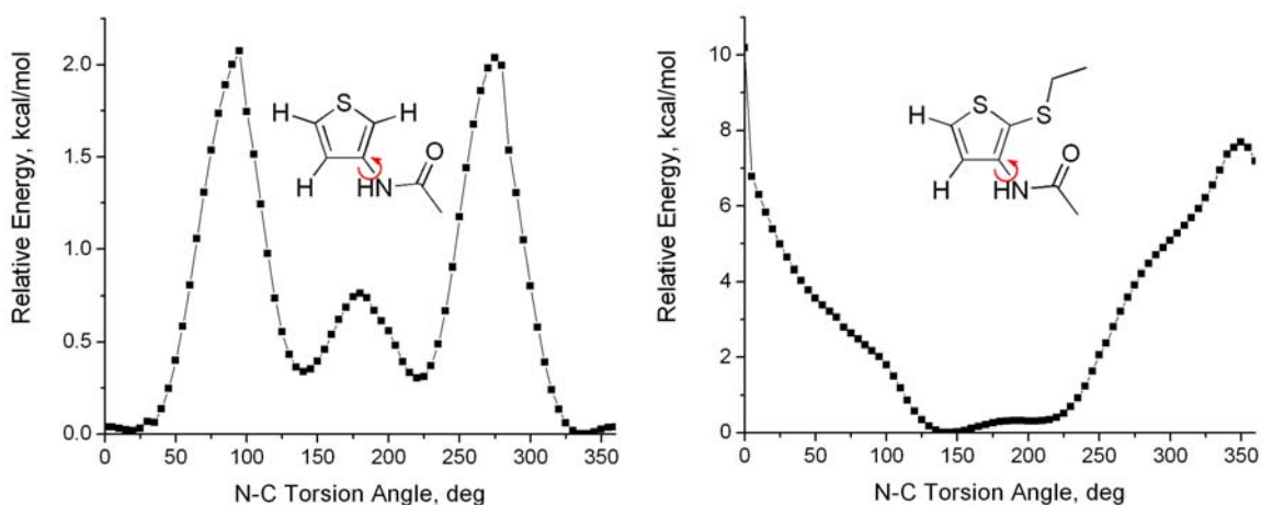
Figure 2-12. Relative energy calculations for rotation of an acetamide substituent about the N_{\text{amide}}-C_{\text{thiophene}} bond without (left) and with (right) ortho thioethyl substitution.
