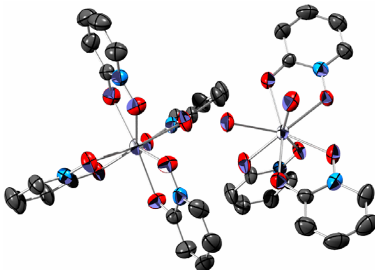
Figure 4-4. X-ray diffraction structure of the Pu(IV)-1,2-HOPO mixed salt complex Pu( 4-1 ) 4 ·Pu( 4-1 ) 3 (H 2 O) 2 ·ClO 4 . Hydrogen atoms and the perchlorate counterion have been omitted for clarity. Thermal ellipsoids are drawn at the 50% level. Carbons are gray, oxygens red, and plutonium silver.
