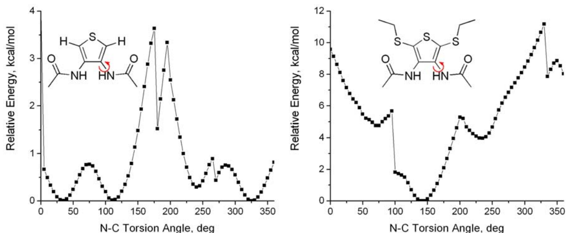
Figure 2-13. Relative energy calculations for rotation of an acetamide substituent about the N_{\text{amide}}-C_{\text{thiophene}} bond in the presence of an ortho acetamide in the absence (left) and presence (right) of 2,5-dithioethyl substitution.
