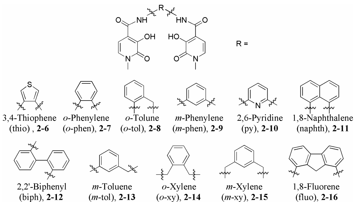
Figure 2-3. Rigidly-linked bis-Me-3,2-HOPO ligands synthesized for structural studies with the uranyl cation. Backbone abbreviations are indicated and amide attachment points are indicated by wavy lines.
