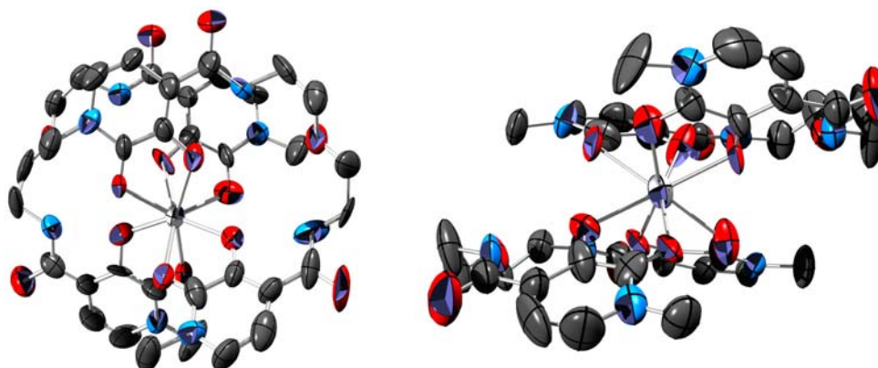
Figure 4-2. Crystal structure of Pu(5LiO-Me-3,2-HOPO) 2 . 15
