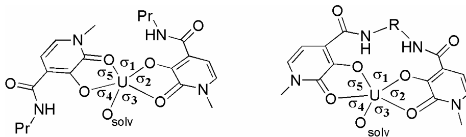
Figure 2-6. Equatorial O-U-O bond angle designations for \text{UO}_2(\mathbf{2-1})_2(\text{DMF}) (left) and \text{UO}_2(\text{bis-Me-3,2-HOPO})(\text{solv}) (right), tabulated in Table 2-3. Uranyl oxo atoms are removed for clarity.
