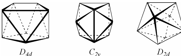
Figure 4-6. Ideal coordination polyhedra: Square antiprism ( D_{4d} ), bicapped trigonal prism ( C_{2v} ), and trigonal dodecahedron ( D_{2d} ).
