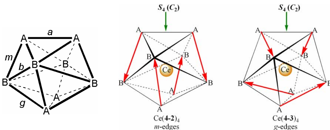
Figure 4-11. Hoard and Silverton 27 edge notation of trigonal dodecahedral geometry (left) and coordination polyhedra of the Ce(4-2) 4 (middle) and Ce(4-3) 4 (right) complexes. Ligand-spanned edges are indicated by arrows whose heads point towards the methyl substituents, with primary molecular symmetry axes indicated.
