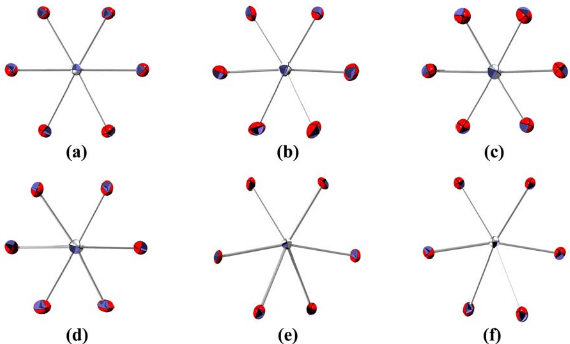
Figure 3-10. Uranyl binding pockets in the \text{UO}_2[\text{TAM}(\text{HOPO})_2] crystal structures: (a) \text{TAM}(2\text{Li-Me-3,2-HOPO})_2 , 3-2 ; (b)-(e) \text{TAM}(o\text{-phen-1,2-HOPO})_2 , 3-4 , #1-#4 respectively; (f) \text{TAM}(o\text{-phen-Me-3,2-HOPO})_2 , 3-5 . Structures are viewed down the uranyl \text{O}=\text{U}=\text{O} vector, although uranyl oxo atoms have been removed for clarity, and oxygens are oriented as illustrated in Figure 3-9. Thermal ellipsoids are drawn at the 50% probability level. Oxygen atoms are red and uranium is silver.
