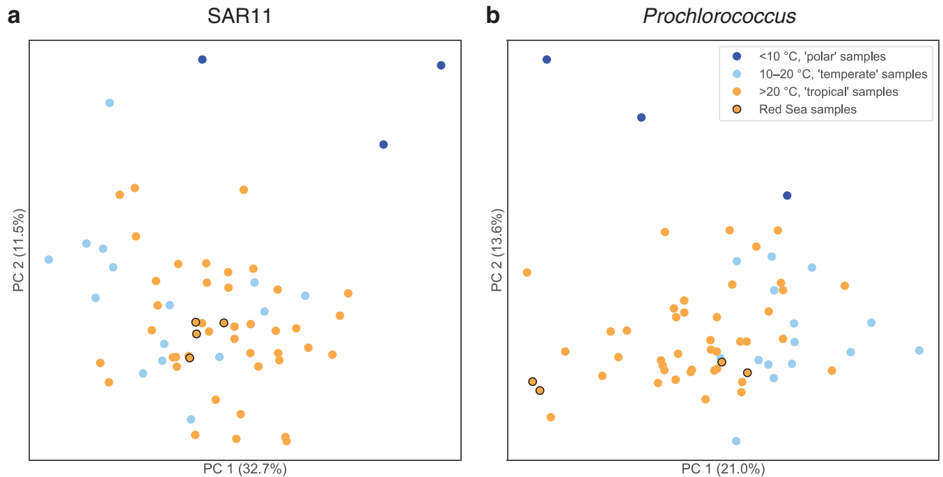
FIG 5 Principal component analysis of Tara Oceans surface samples by the abundance of SAR11 (a) and Prochlorococcus (b) OGs. The ordination shows the similarity of Tara Oceans samples to each other along the first two principal components. Samples are colored by Tara temperature categories: polar samples (<10°C) are dark blue, temperate samples (10 to 20°C) are light blue, tropical samples (>20°C) are orange, and Red Sea tropical samples are orange with black edges. Red Sea samples and Tara samples generally show more separation based on temperature when ordinated by Prochlorococcus OG composition than by SAR11 OG composition.
