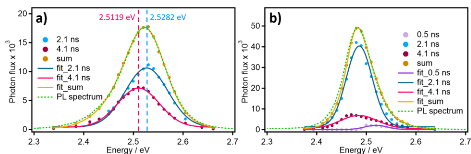
Figure 6 Energy-dependent time-resolved PL spectra at a) 260 K and b) 15 K. Tetradecane PQD suspensions are frozen from 15-260 K to ensure QD aggregation is minimized. PL and TRPL measurements were conducted under the same conditions as Figure 3a.
