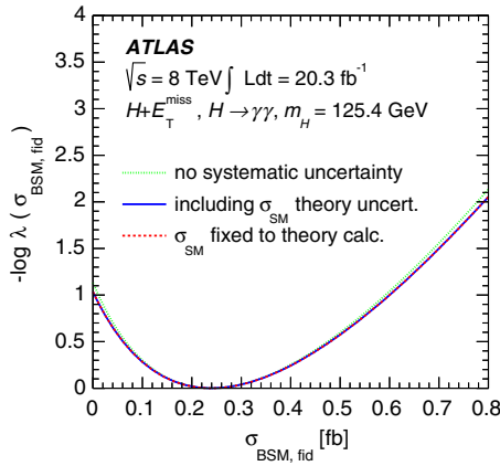
FIG. 3 (color online). Profile likelihood ratio ( \lambda ) as a function of \sigma_{\text{BSM, fid}} , the fiducial cross section for production of a BSM H + \text{DM} process in the \gamma\gamma + E_{\text{T}}^{\text{miss}} channel taking into account the contribution of the SM component. The solid blue likelihood curve shows that the number of events observed in the data corresponds to a 1.4\sigma deviation using the asymptotic formulas in Ref. [47]. The dotted green likelihood curve only includes statistical uncertainties. The dashed red likelihood curve allows for modifications of the central value and uncertainty on the SM component as described in the text.
