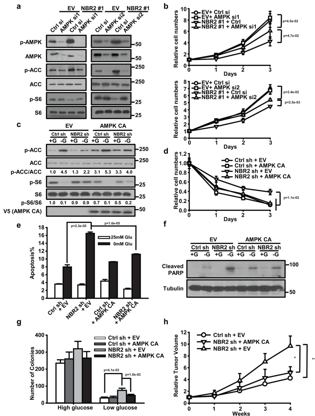
Figure 7. The functional effects of NBR2 are partially mediated by AMPK (A and B) UMRC2 cells stably expressing EV or NBR2 expression vectors were transfected with AMPK siRNA ( AMPK si1 or si2) or control siRNA (Ctrl si). Protein lysates were prepared and analyzed by Western blotting (a) , or cells were cultured in 25 mM glucose-containing medium for different days as indicated, and then subjected to cell proliferation analysis (b) (Mean \pm s.d., n=3 biologically independent extracts, two-tailed paired Student's t-test). (c–g) MDA-MB-231 cells with stable expression of control shRNA (Ctrl sh) or NBR2 shRNA ( NBR2 sh) were infected with empty vector (EV) or constitutively active
