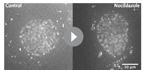
Video 1. CSV decreases after NEBD even in the absence of MTs. Video of representative cells (Control and Nocodazole-treated) shown in Figure 1C (SiR-DNA staining). Frame intervals are 2 min. Video is shown at 600x speed.
