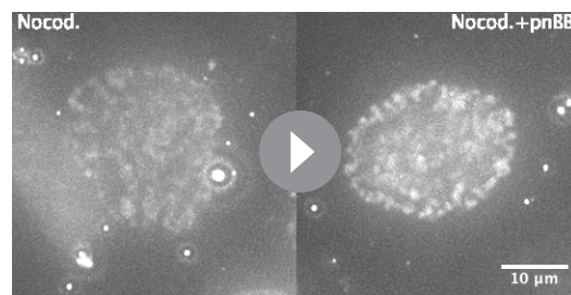
Video 6. CSV reduction is almost completely alleviated when myosin II activity is inhibited in the absence of MTs. Video of representative cells (Nocodazole and Nocodazole +pnBB treated) shown in Figure 3B (SiR-DNA staining). Frame intervals are 2 min. Video is shown at 600x speed.
