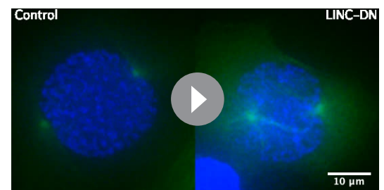
Video 7. Evidence that removal of actin network delays chromosome congression and anaphase onset. Video of representative cells (Control and LINC-DN expressing) shown in Figure 5A (expressing GFP-tubulin and H2B-cerulean). Frame intervals are 2 min. Video is shown at 600x speed.
