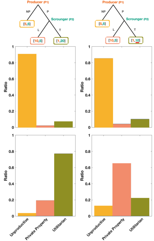
Figure 3: Action vs. Strategy Learning conditions in two different versions of the Producer-Scrounger Game. (a) An Action Learner learns q-values for each action, whereas a Strategy Learner assigns q-values for each strategy profile. (b) Outcome ratios in selfish agents using Action Learning (top) vs. Strategy Learning (bottom).
