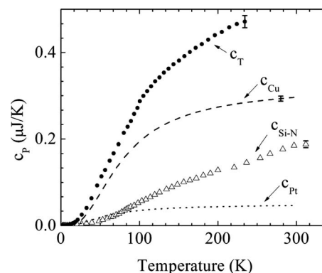
FIG. 3. Total measured heat capacity c_T of a 50 nm thick device with 86.4 nm of Cu [contributions from: Cu conduction layer; Si–N membrane; Pt heater, thermometer, and leads; and a\text{-Nb}_y\text{Si}_{1-y} thermometers (small and not shown)]. c_{\text{Cu}} and c_{\text{Pt}} are calculated from bulk data. (Ref. 19) c_{\text{Si-N}} is calculated from c_T - c_{\text{Cu}} - c_{\text{Pt}} . (Ref. 12).
