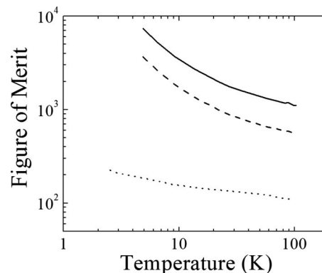
FIG. 2. Low temperature sensitivity \text{FOM} = (t/t_{\text{th}})^{1/2} T^{3/2} / \rho^{1/2} d\rho/dT of the nanocalorimeter using a\text{-Nb}_y\text{Si}_{1-y} thermometers. The predicted nanocalorimeter FOM (solid line) which is the same as the microcalorimeter, FOM for t/t_{\text{th}} = 1/6 and \rho = \text{constant} (dashed line), and the measured FOM with t/t_{\text{th}} = \text{constant} and \rho decreased to reduce the thermometer resistance below 1 M \Omega .
