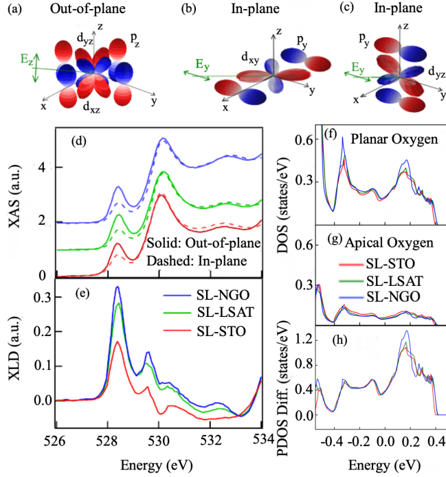
FIG. 3. Schematic diagram of linearly dependent XAS measurement at O K-edge. (a) Out-of-plane channel. (b) and (c) In-plane channel. (d) Polarization dependent O K-edge x-ray absorption (XAS) spectra of SL-STO (red), SL-LSAT (green) and SL-NGO (blue). The solid/dashed line denotes XAS from out-of-plane/in-plane measurement. The absorption is shifted vertically for clarity. (e) X-ray linear dichroism extracted from (d). Density of states (DOS) of the planar oxygen ions (f) and apical oxygen ions (g). (h) The projected DOS difference (PDOS Diff.) extracted from (f) and (g).
