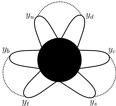
Figure 3: Instanton vacuum diagram arising from closing the SM fermion legs with Higgs loops.
