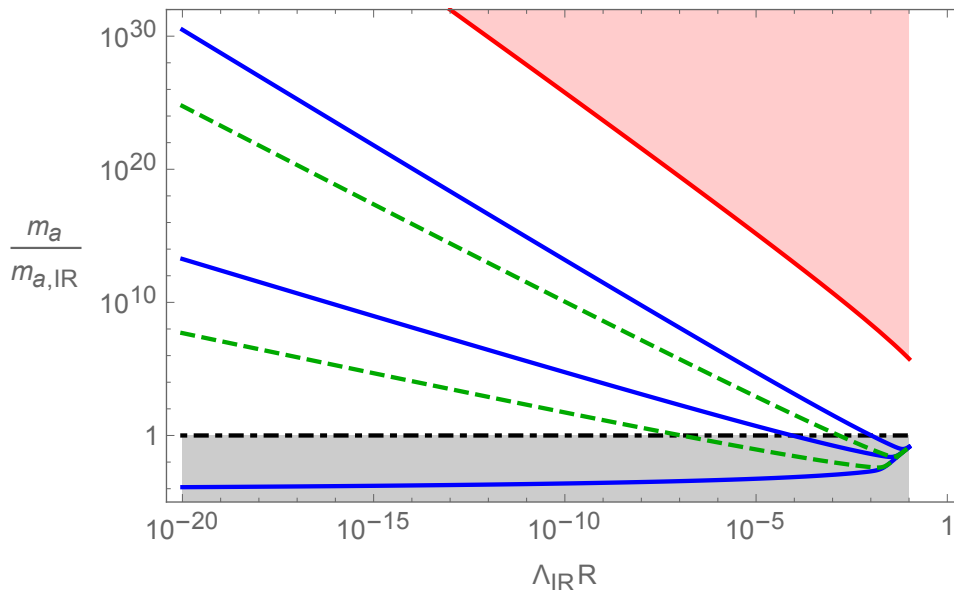
Figure 2: The axion mass ratio for the pure YM case as a function of \Lambda_{\text{IR}}R for various contours of \epsilon = (0.3, 0.25, 0.2) (top to bottom). The solid blue lines are the exact numerical integration results using (8) with no higher dimension terms ( c_6 = 0 ). The green dashed line represents the addition of the higher dimension term (11) with c_6 = 0.5 and \epsilon = 0.52(0.47) for the upper (lower) line. The red line represents the maximum enhancement using m_{a,5} that would occur at the 5D strong-coupling limit.
