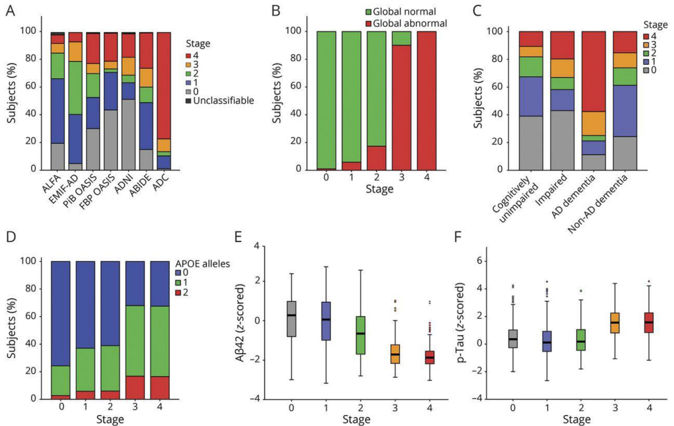
FIGURE 2 (A) Baseline distribution of staging classification per cohort. Stages refer to a model developed in CU individuals based on the sequential addition of four clusters of regional A\beta : Stage 0: no tracer uptake; Stage 1: cingulate regions; Stage 2: precuneus, paracentral gyrus, lateral orbital cortex, and insula; Stage 3: basal temporal, frontal, and additional associative cortices; Stage 4: other temporal and occipital regions. Classification based on A\beta staging model vs (B) global A\beta PET classification. (C) syndromic diagnosis, (D) genetic risk, (E) z-scored CSF A\beta_{42} levels, and (F) log-transformed z-scored phosphorylated tau (p-tau) values. A\beta , amyloid beta; ABIDE, Alzheimer's Biomarkers in Daily Practice; ADC, Amsterdam Dementia Cohort; ALFA, Alzheimer's and Family cohort; EMIF-AD, European Medical Information Framework for AD; FBP, florbetapir; PIB, Pittsburgh compound B. Reproduced with permission from Collij et al. 36
