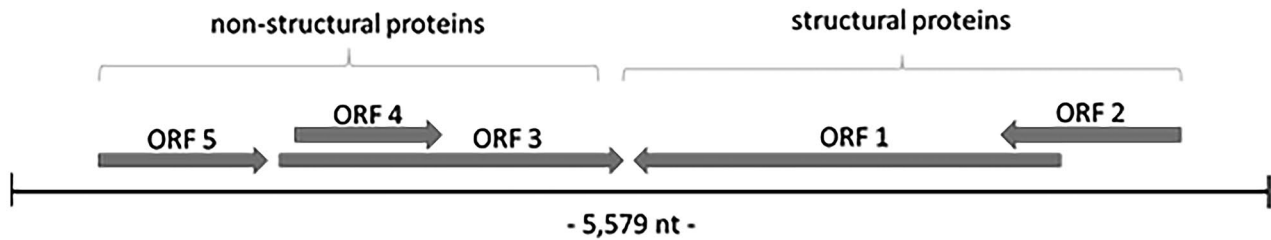
Figure 9. Genomic organization of Tenebrio molitor densovirus ( TmDNV ) indicating the location and direction of transcription for each of the 5 open reading frames (ORFs).
