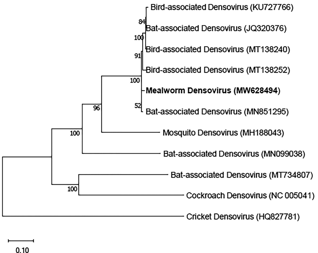
Figure 10. Phylogenetic analysis of the mealworm densovirus ( TmDNV ) whole-genome sequence in relation to other insect densoviruses. The numbers at the nodes represent bootstrap confidence values for 1000 replicates based on maximum likelihood analysis.
