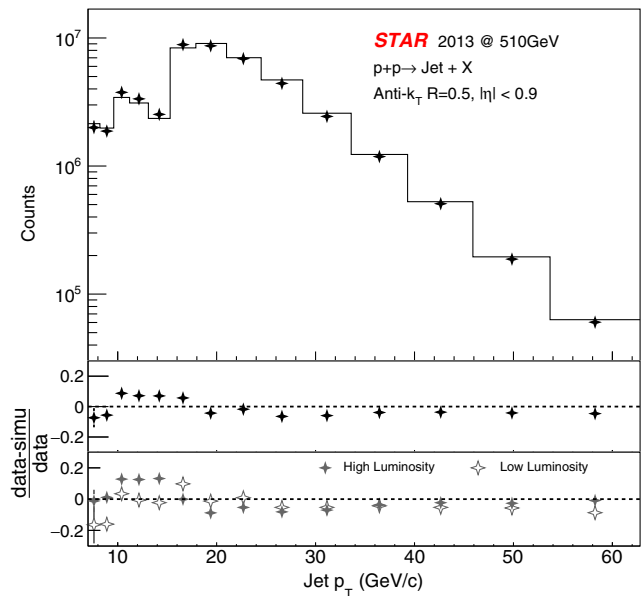
FIG. 1. Comparison between data (points) and embedded simulation (histogram) of the inclusive jet yield versus p_T at detector level. The central panel shows the ratio of the relative differences between all data runs used in the analysis and the simulation, and the lower panel shows the ratio for data separated into high and low luminosity runs. Statistical uncertainties are smaller than most of the points.
