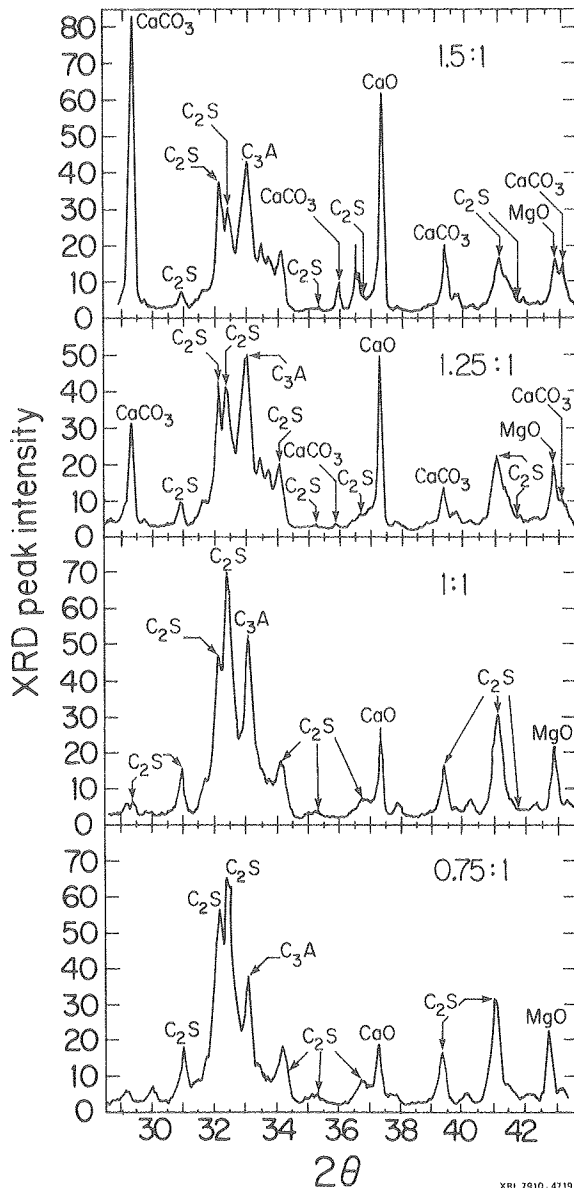
Figure 2. X-ray diffraction patterns of cements produced by heating limestone and Lurgi spent shale at 1000°C for 1 hr. Limestone-spent shale ratios range from 0.75:1 to 1.5:1.
