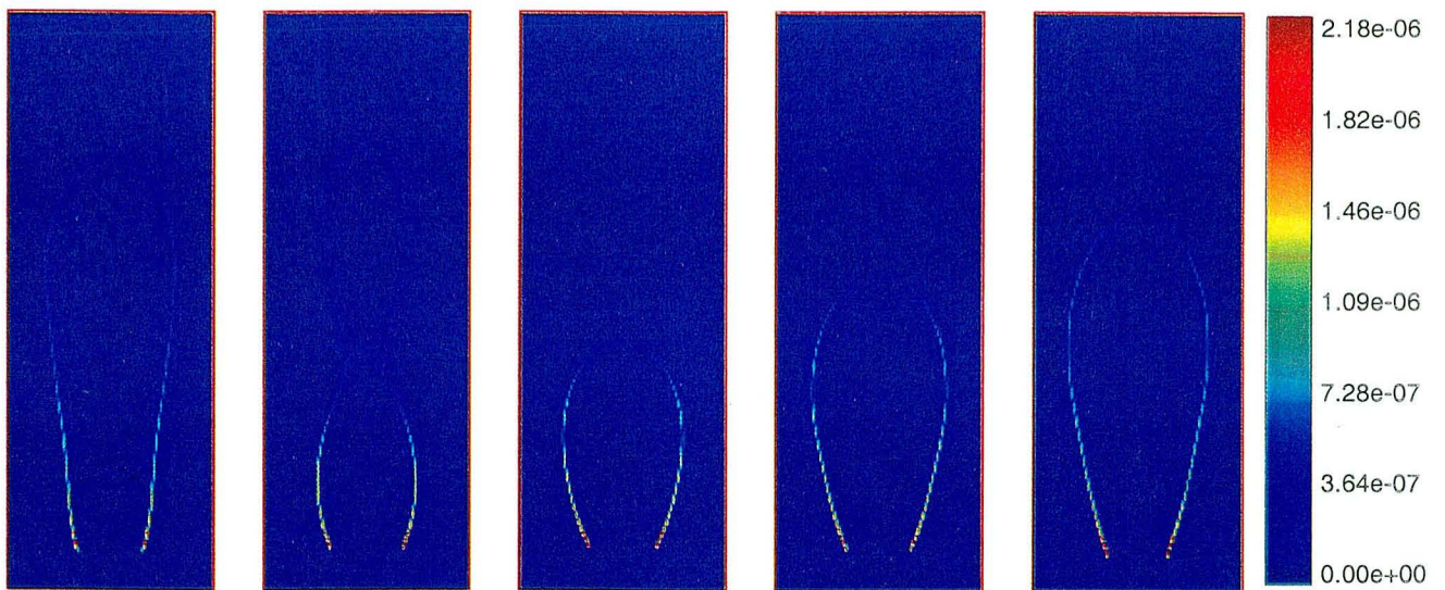
Figure 11. X_{CH} for \epsilon = 0.50 , at 0.01, 0.02, 0.03, 0.04, and 0.05 s, reflected about the origin. The region shown spans \pm 0.88 \times 4.88 cm.
