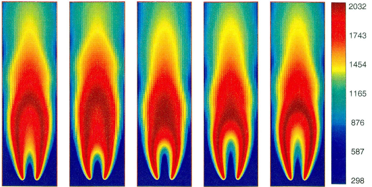
Figure 8. Temperature (in K) for \epsilon = 0.25 , at 0.01, 0.02, 0.03, 0.04, and 0.05 s, reflected about the origin. The region shown spans \pm 1.12 \times 7.52 cm.
