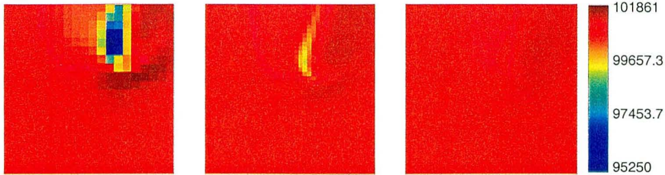
Figure 7. Computed thermodynamic pressure in Pa at the flame tip. Maximum error values with respect to atmospheric pressure, from left to right are 6075, 2107 and 556 Pa, for respective grid spacings, \Delta x = 0.02, 0.01, 0.005 cm.
