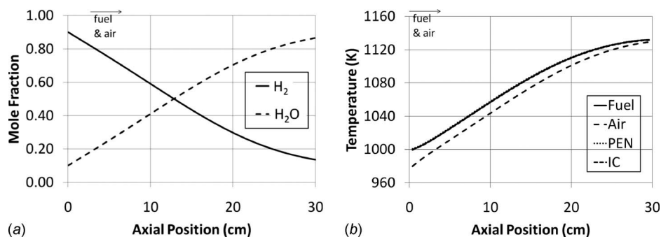
Fig. 4 Fuel channel species mole fractions (a) and temperature distributions (b) along the cell length for humidified H 2 , coflow operation
