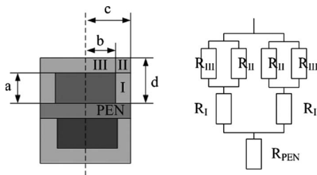
Fig. 3 Electrical resistance of ceramic interconnects
