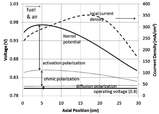
Fig. 7 Predicted working voltage, current density and contribution of all the various polarization terms along the cell length for CH 4 containing syngas, coflow operation
