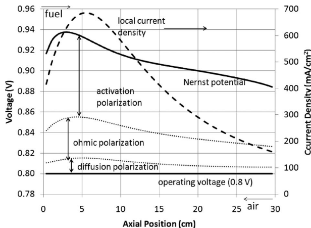
Fig. 9 Predicted working voltage, current density and contribution of all the various polarization terms along the cell length for CH 4 containing syngas, counterflow operation
