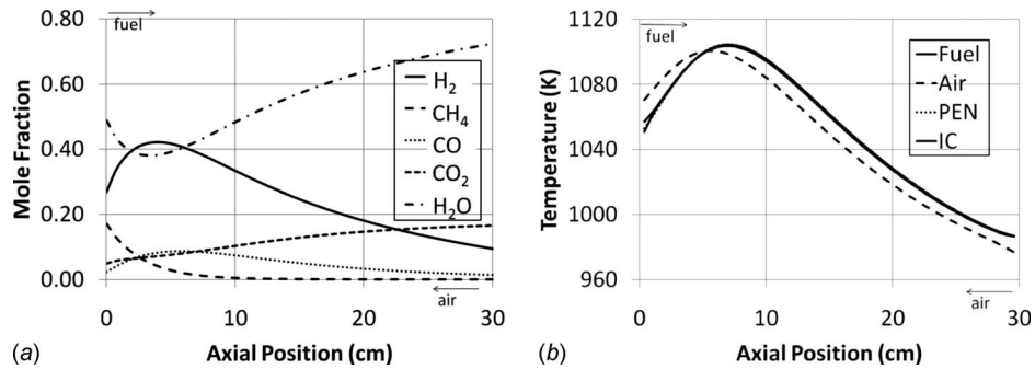
Fig. 8 Fuel channel species mole fractions (a) and temperature distributions (b) along the cell length for CH 4 containing fuel with internal reformation, counterflow operation
