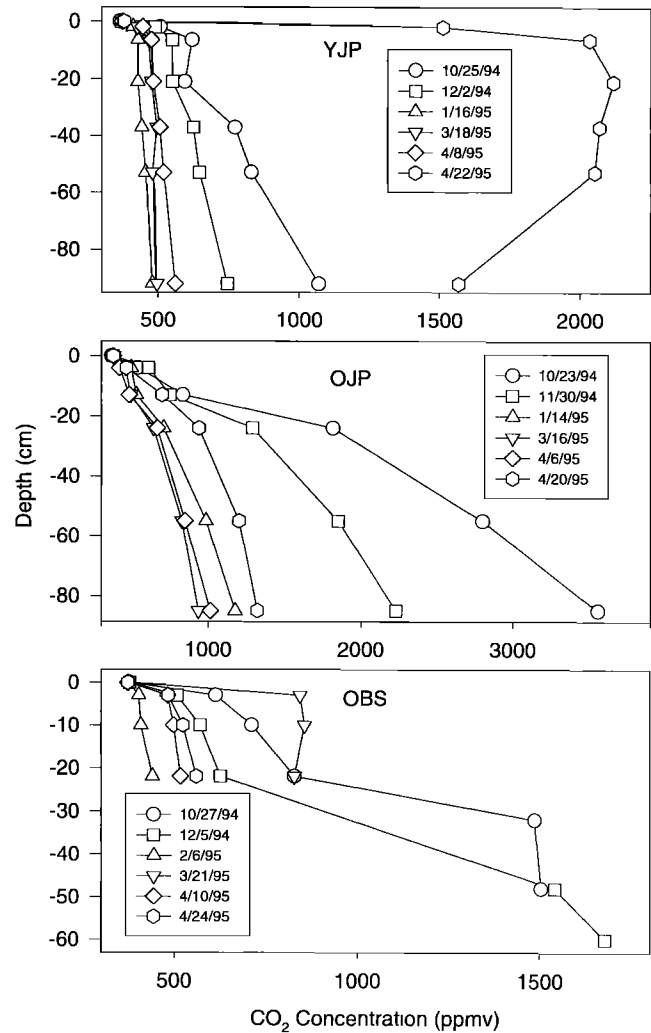
Figure 3. Carbon dioxide concentration versus depth profiles for soils during the winter of 1994–1995. Sites are as described for Figure 1. Depths are relative to the soil surface. Concentrations reported for zero depth are ambient atmospheric CO 2 concentrations at a height of 1.5 m and not the concentrations at the soil-snow interface.
