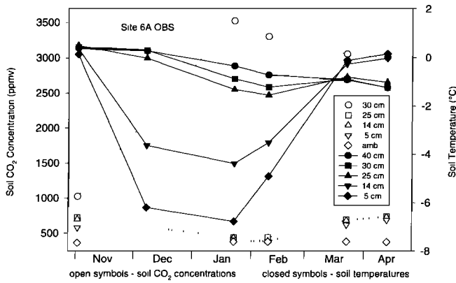
Figure 4. Soil temperatures (solid lines) and CO 2 concentrations (dashed lines) for OBS site 6A in 1994–1995. Depths are relative to the soil surface.
