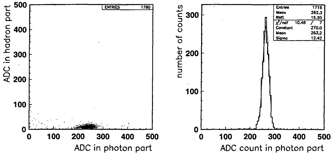
Fig. 3. Correlation plot of the ADC counts in the hadron vs. the photon part for a 30 GeV electron beam incident on cell 67 (left), and its projection onto the photon axis. The solid line is a gaussian fit to the data.
