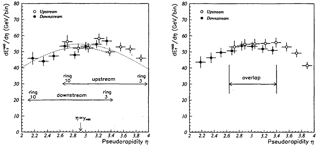
Fig. 10. dE_T^{\text{HAD}}/d\eta distribution before (left) and after (right) the non-uniformity correction for both up/downstream data.
