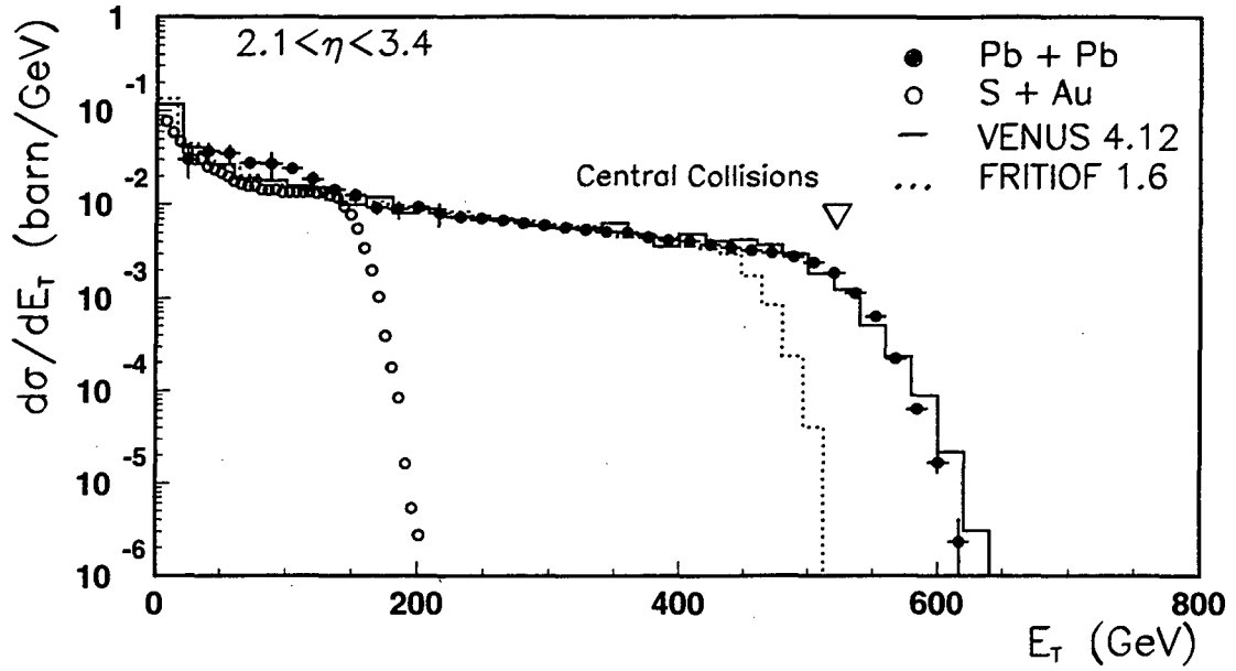
Fig. 13. Transverse energy spectrum for Pb+Pb collisions at 158 GeV/A.
