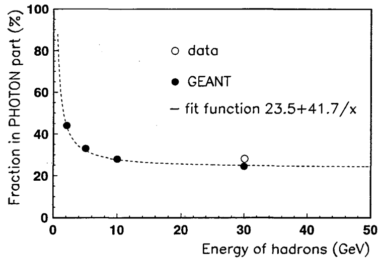
Fig. 7. GEANT estimation of the fraction of hadronic energy deposited in the photon part (filled circles). The corresponding point from the calibration data at 30 GeV is also shown (open circle).
