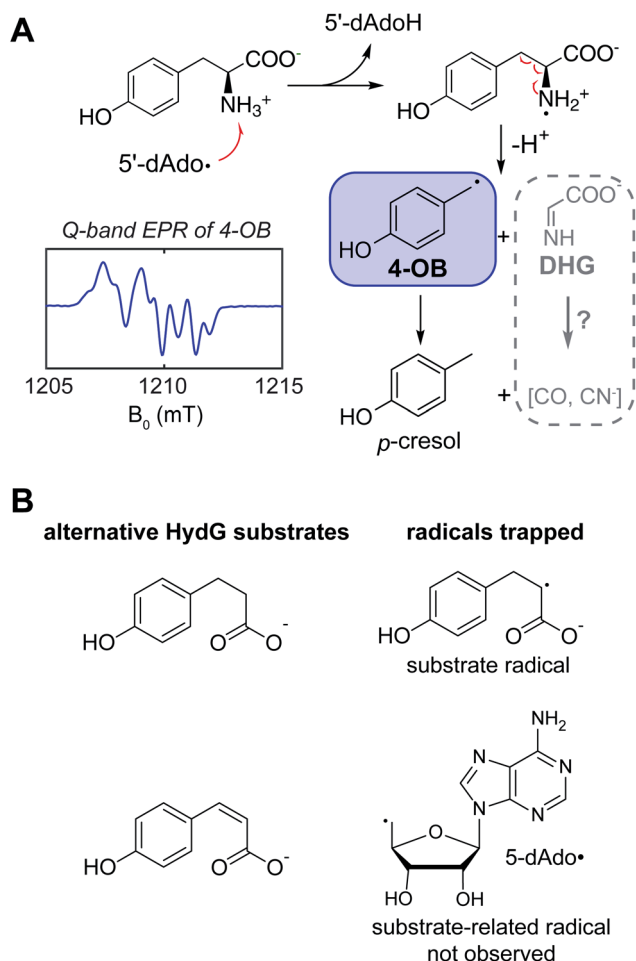
Fig. 3 The rSAM chemistry performed by HydG. (A) Reaction mechanism of tyrosine cleavage into the diatomic CO and CN - ligands. (B) Alternative substrates tested with HydG, 4-hydroxy phenyl propanoic acid and cis-p -coumaric acid, and the corresponding radicals trapped in their reactions.
