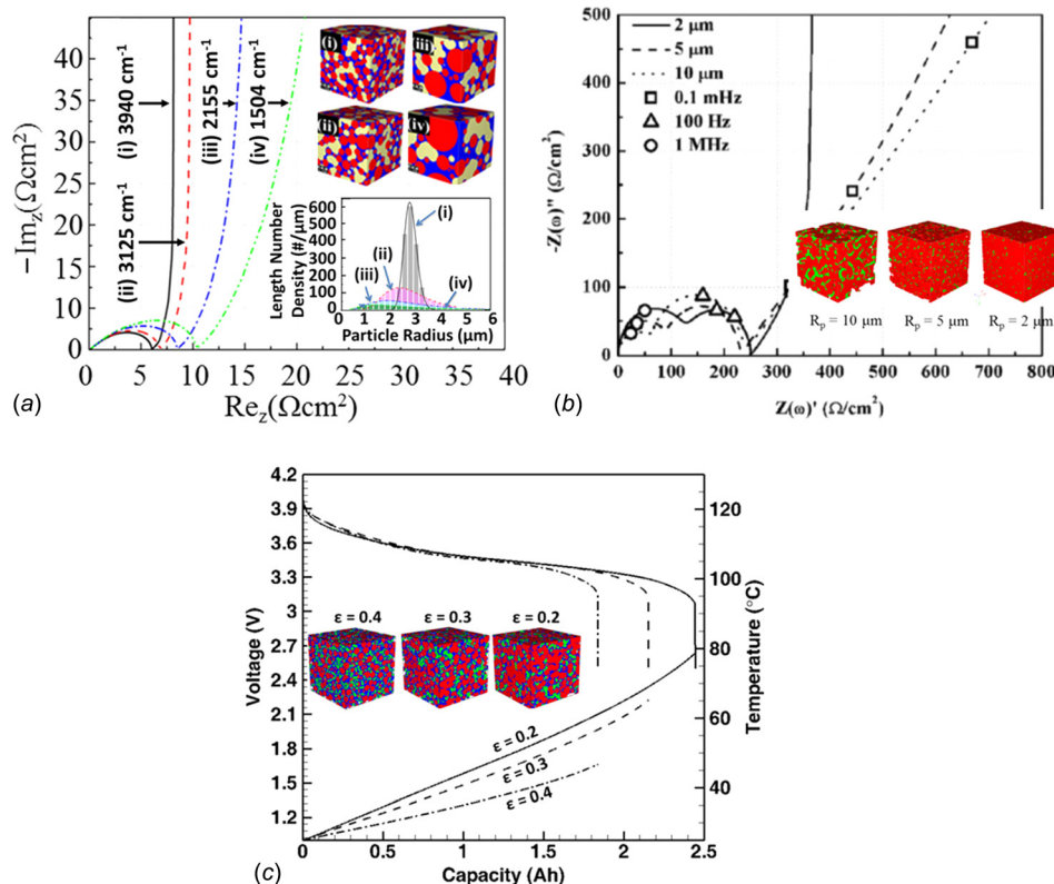
Fig. 14 Effect of typical Li-ion battery electrode microstructures on the impedance and thermal response [161,164]. (a) and (b) Variation in active material mean particle size and size distribution significantly affects the interfacial resistance and impedance response. (c) Electrode porosity plays an important role in electrolyte phase resistance and hence cell temperature rise due to Joule heating. (a) Effect of active material size distribution on EIS (reproduced with permission from Cho et al. [161], copyright 2015 by PCCP, Royal Society of Chemistry), (b) effect of mean particle size on EIS (reproduced with permission from Chen and Mukherjee [164], copyright 2015 by Royal Society of Chemistry), and (c) effect of electrode microstructure on performance and temperature rise.
