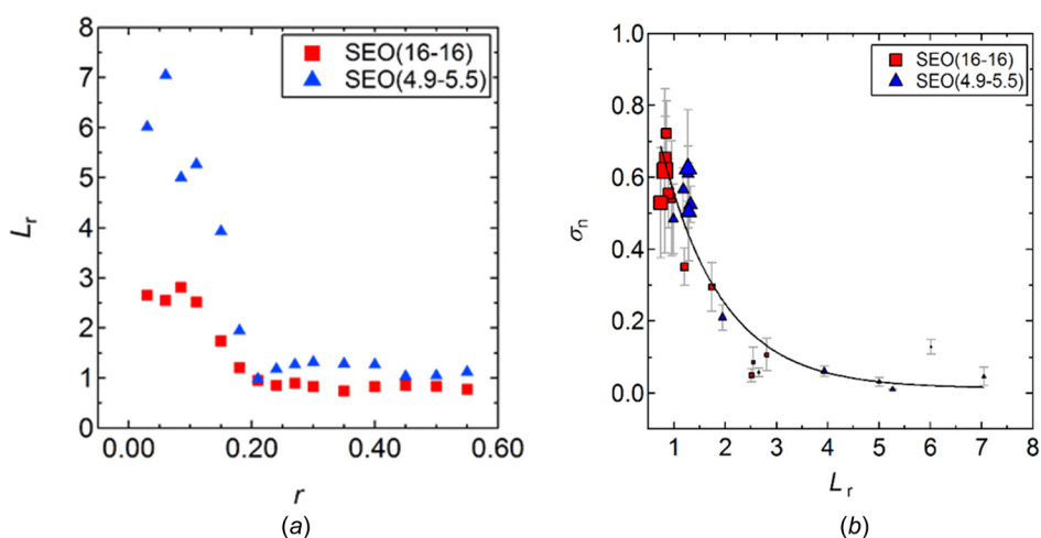
Fig. 3 (a) Grain size, L_r , expressed as a number of lamellae per grain, is plotted as a function of salt concentration, r . Grain size decreases as salt concentration increases, in SEO/LiTFSI of two different molecular weights. (b) Conductivity of SEO/LiTFSI normalized by the conductivity and volume fraction of PEO/LiTFSI, \sigma_n , is plotted as a function of L_r . The marker shows the concomitant changes in r . Larger markers represent higher values of r . Normalized conductivity decreases as grain size increases.
