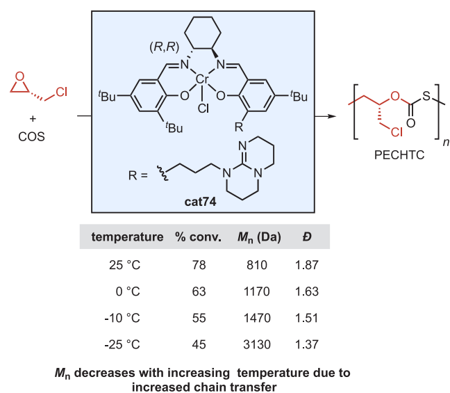
Figure 21. Temperature-dependent activity of cat74 in ECH/COS ROCOP.
