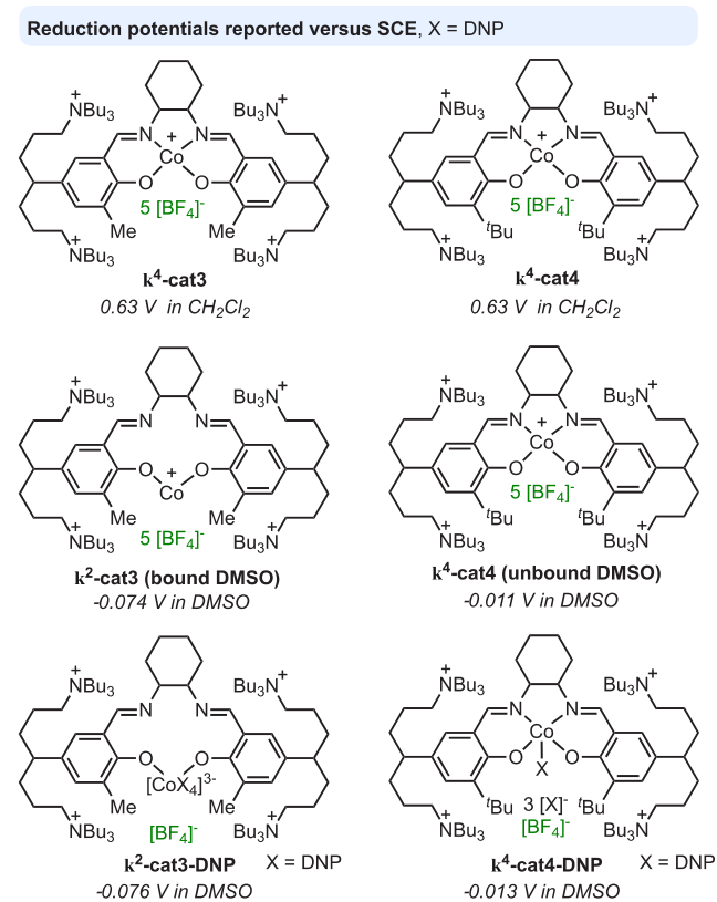
Chart 3. Redox Behavior of κ 4 and κ 2 Multifunctional (salcy)CoX Complexes cat3 and cat4
