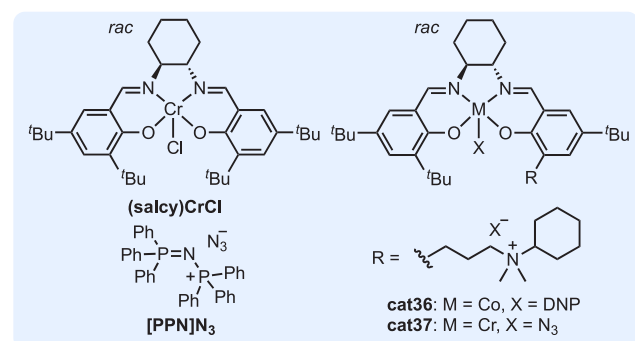
Figure 12. ROCOP of (a) CHO/CO 2 and (b) CPO/CO 2 using the binary catalyst system (salcy)CrCl/[PPN]N 3 . (c) Use of multifunctional catalysts cat36 and cat37 at 70 °C produce exclusively PCPC during CPO/CO 2 ROCOP.
