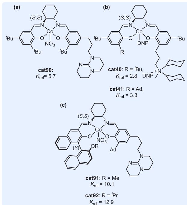
Figure 39. Kinetic resolution copolymerization of ( R )-PO and CO 2 by chiral multifunctional complexes.
