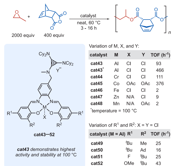
Figure 7. Catalytic activity in PO/CPMA ROCOP with cat43 – cat52 .
