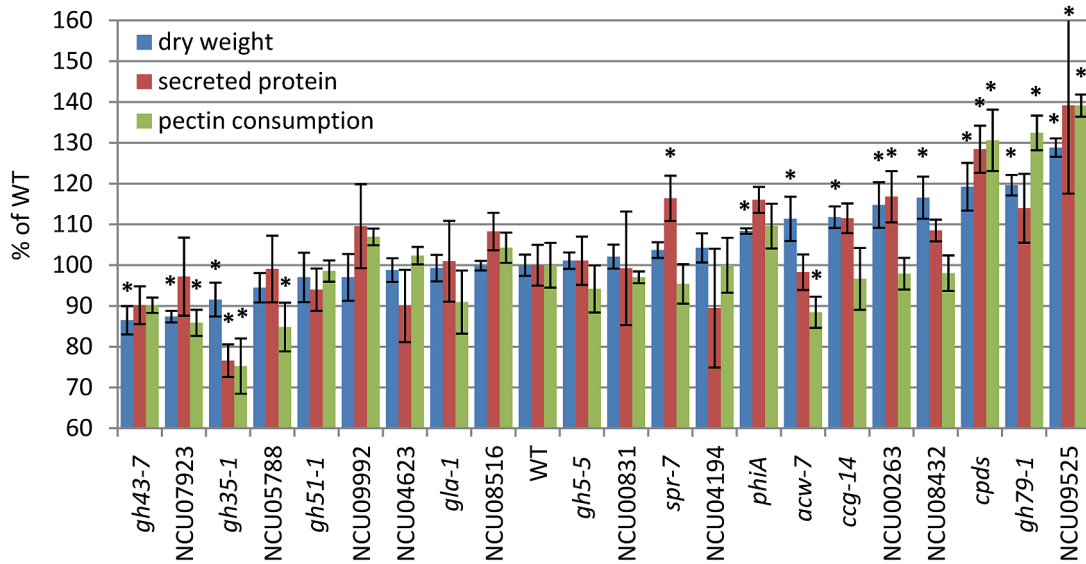
Fig. 7. Screening of strains containing gene deletions for secreted proteins with pectin-specific expression patterns. N. crassa strains containing deletions of genes present in pectin-specific clusters 6 and 10 (Fig. 6) and that were also identified in the pectin and OPP secretomes (see Fig. S7 for annotation) were assayed for their phenotype when grown on pectin as sole C-source for 4 days. The fungal dry weight, the concentration of secreted protein, and the consumed pectin (the difference between day 0 and day 4 in total reducing ends in the culture supernatants) were measured and compared with WT (FGSC# 2489), which was set to 100%. The strains were ordered according to their recorded dry weight from the least (left) to the most (right). Bars represent standard deviations. The asterisk (*) indicates a significant difference from WT with an unadjusted P -value of < 0.003 using a one-way Anova.
