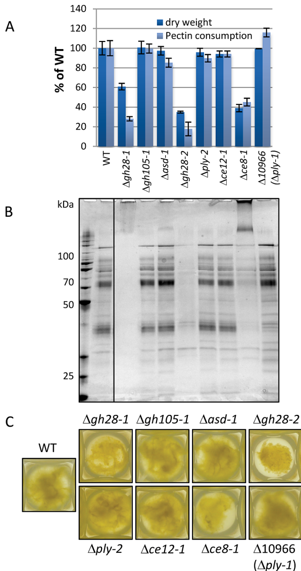
Fig. 3. Pectin methylesterase and polygalacturonases are required for robust growth on pectin. A. N. crassa strains containing deletions of genes involved in pectic backbone degradation (Table 1) were assayed for their phenotype when grown on pectin as sole C-source for 4 days. The fungal dry weight and the consumed pectin (the difference between day 0 and day 4 in total reducing ends in the culture supernatants) were measured and compared to WT (FGSC #2489). Bars represent standard deviations ( n = 3 ). B. Silver stained SDS-PAGE of secreted proteins from the mutants in (A). The same volume (30 \mu l) of supernatant was loaded in each lane. C. Visible growth phenotype of the same cultures as in (A) and (B) after 4 days of growth on 1% pectin in 24-deep-well plates. Representative pictures are shown. Due to a former mis-annotation, \Delta 10966 is actually a deletion of the pectate lyase ply-1 (NCU06326) and NCU06327, encoding a cytochrome P450 protein. However, no phenotype was observed under these conditions.
