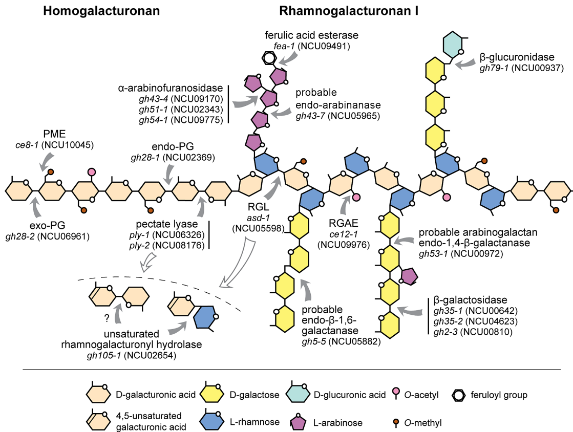
Fig. 10. Model view of the pectin-degrading machinery of N. crassa . Depicted is an inventory of the N. crassa genes encoding enzymes with pectinolytic activities, that were found to be specifically upregulated on pectin and were also identified from the pectin and/or OPP secretomes (exception: gh53-1 was not detectable in the secretome but significantly induced on pectin). Grey solid arrows indicate the points of attack on the pectin backbone or RG-I side chains. The open arrows indicate that the (unsaturated) D-GalA oligomers liberated by the action of the rhamnogalacturonan lyase ASD-1 (but possibly also the pectate lyases PLY-1 and PLY-2) are most likely imported for further hydrolysis inside the cell. Note that the pectin model is not to scale and that the linkages shown are of reported structures, but (in particular for RG-I) are not limited to these. RG-II and XG are not shown, since no dedicated enzymes were found in the N. crassa secretome and transcriptome. PG: polygalacturonase; PME: pectin methyltransferase; RGAE: rhamnogalacturonan acetyltransferase; RGL: rhamnogalacturonan lyase.
