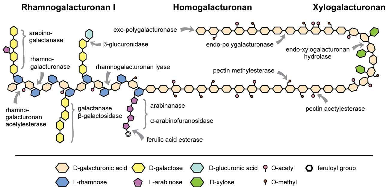
Fig. 1. Schematic structure of pectin and the sites of action of pectinolytic enzymes. Pectin is a family of at least four different types of polysaccharides: homogalacturonan (HG), rhamnogalacturonan I (RG-I), xylogalacturonan (XG), and rhamnogalacturonan II (which is not shown here since it is not known to be a substrate for microbial degradation). The figure shows representative structures and is not to scale. HG and RG-I are generally much more abundant in plant cell walls than the other components. Please note that the enzyme classes indicated here are not necessarily found in all fungi.
