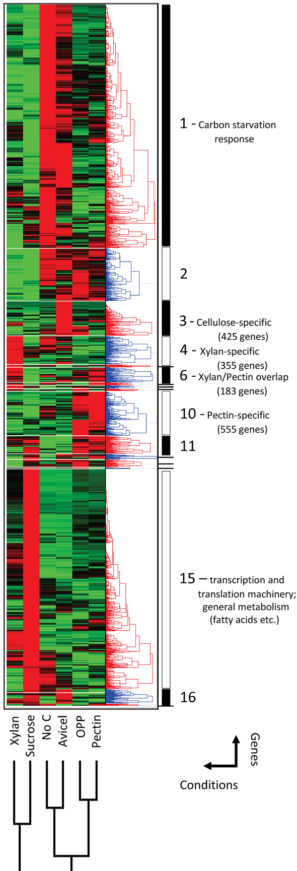
Fig. 6. Hierarchical clustering of expression profiles for pectin, OPP, xylan, Avicel, sucrose and no carbon response. The averaged transcriptional expression profiles for the full-genome response to all three major plant cell wall polysaccharides (cellulose, xylan and pectin) as well as OPP and control conditions (no carbon and sucrose) were normalized and clustered in two dimensions: six conditions (horizontal) and ~ 8500 genes (vertical), using the software Hierarchical Clustering Explorer v3.0 (see also Supporting data set 4). The resulting heat map (normalized from bright green = low expression to bright red = strong expression) was divided into 17 sub-clusters. Large clusters are marked by black and white bars, while smaller clusters are indicated by short dashes. Genes with consistently low expression (< 10 FPKMs in all conditions) were not included in the clustering.
