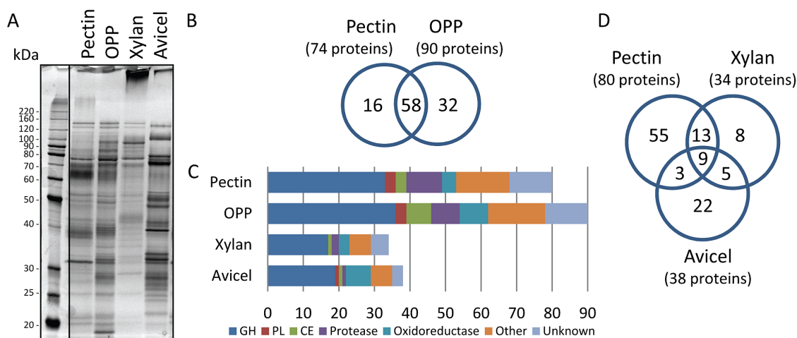
Fig. 2. Comparative proteomic analysis of the N. crassa secretome on pectin and OPP.
