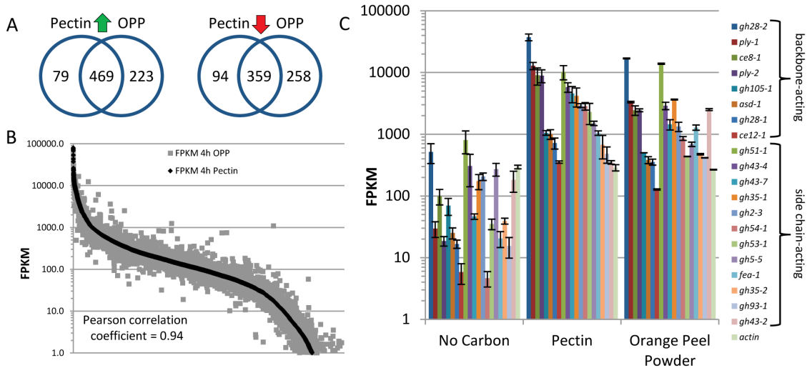
Fig. 4. Transcriptional induction of pectinolytic genes by pectin and OPP in N. crassa .
