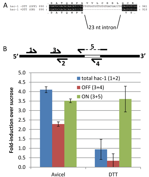
Fig. 8. Growth on Avicel triggers the unfolded protein response (UPR).
