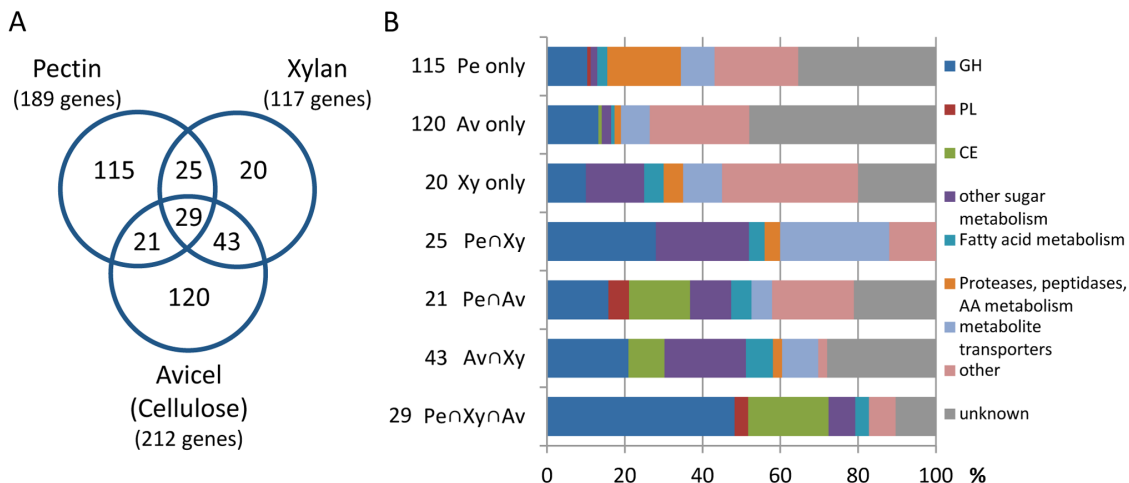
Fig. 5. Comparative transcriptomics reveals the importance of polysaccharide esterases and oligosaccharide hydrolases.
