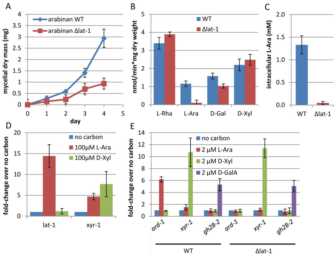
Fig. 9. Characterization of the newly identified L-arabinose transporter LAT-1.
