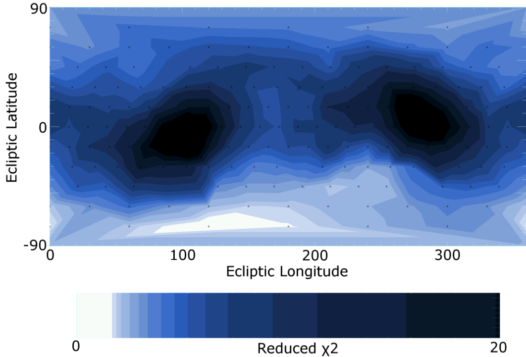
Figure 4 Map of \chi^2 with pole orientation using the combined 1999 and 2005 data set and an 8 th order spherical harmonic shape. Triangles show the poles for individual model runs. Black regions have the highest \chi^2 (poorest fit) and white regions the lowest. The two large dark areas show that the regions where the line of sight lies nearly along the pole are “forbidden”, because the Doppler bandwidth would change dramatically with viewing angle, which is not observed. The North-South ambiguity intrinsic to radar observations is broken due to the motion of the target with respect to the Earth. The pole solution near ecliptic latitude -90 is clearly favored. Further studies examined only poles near this one.
