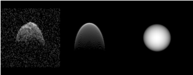
Figure 3. Data (left), simulated data (center) and plane-of-sky image for one of the best-fit triaxial ellipsoid poles. Note that the shape of the leading edge is fairly well matched by the model, but the terminator is too far back in the model.
