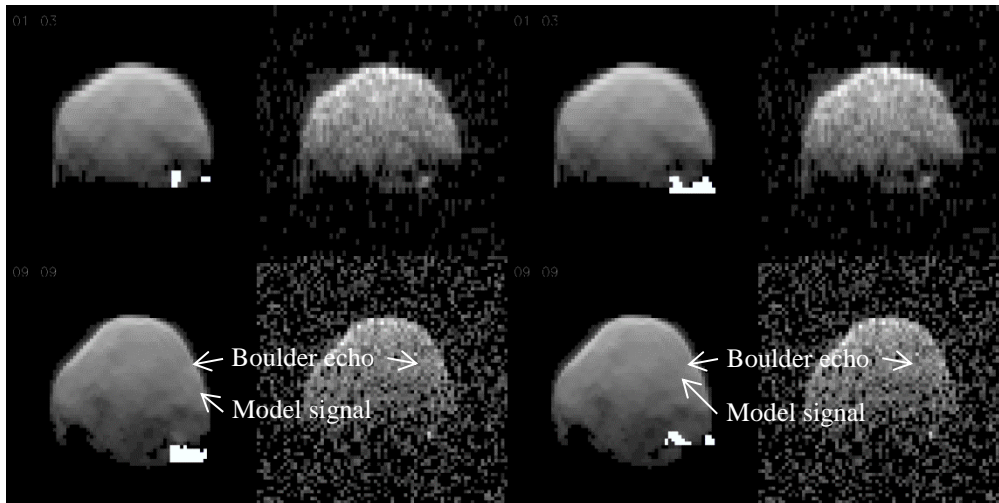
Figure 6. Images showing the model images with the boulder feature. The left set of images has the boulder in the northern hemisphere and the right set has it in the south. The top row is from 1999, and the bottom row is from 2005. The white marks show the computed location of the signal from the boulder. For both northern and southern boulders, the 1999 model overlaps the data. But for the 2005 geometry, the northern boulder does not overlap the data, while the southern boulder does. Therefore, the boulder is in the southern hemisphere.
