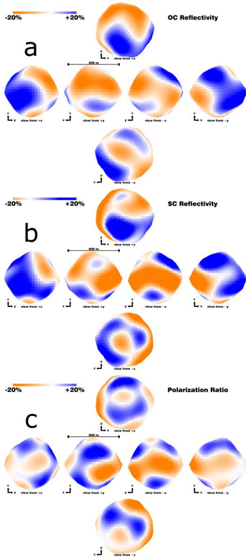
Figure 8 OC (a), SC (b), and SC/OC ratio \mu_C (c) maps of the Benu based on fitting the reflectivity of the surface to the 1999 data. The maps are 4 th -order spherical harmonic fits to the data overlain on the shape model oriented as shown in Figure 5. Orange is low and blue is high reflectivity / ratio, with scale bars showing + and - 20% from the mean. The standard deviations of all of the values are about 10%.
