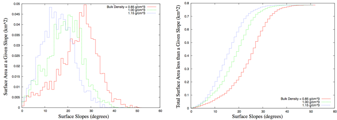
Figure 7 Differential (left) and cumulative (right) distribution of facet-scale surface slopes vs. surface area for Benu for the three different densities. The histogram is computed at a resolution of 1 degree of slope. The total surface area of the asteroid is 0.7855 \text{ km}^2 .
