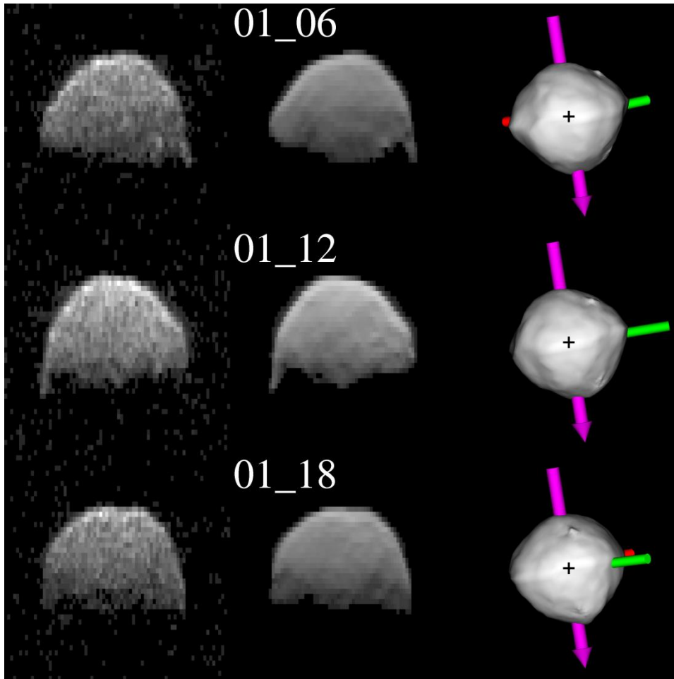
Figure 1. Sample of radar images and the model on 1999 September 24. The left column shows the radar data. The center column shows the model fit to the data. The right column shows the model as it would appear on the sky. In the radar frames, the observer is at the top of the frame looking down. The vertical scale is range from the observer in units of 100 ns, or 15 m. The horizontal axis is Doppler shift, or rotation velocity, which, for a solid body, corresponds to linear distance from the rotation axis after projection onto the plane of the sky, and has been scaled to give approximately square pixels. The numbers label the data sets as described in supplementary online table S1. The complete set of data and fits are shown in the supplementary online figure S1.
