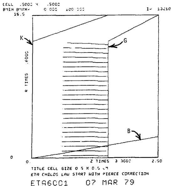
Figure 1: First section of the ETA simulation extending from the Pierce corrected cathode K, to the grid G. The plot shows the magnetic field B. The electrons originate along an equipotential line 0.6 cm before the cathode and terminate on the grid.
