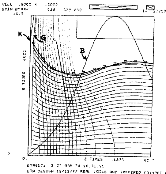
Figure 2: Second section of the ETA simulation extending from the cathode to 60 cm. The electrons are picked up from the previous problem at the grid and accelerated to 2.5 MeV.
