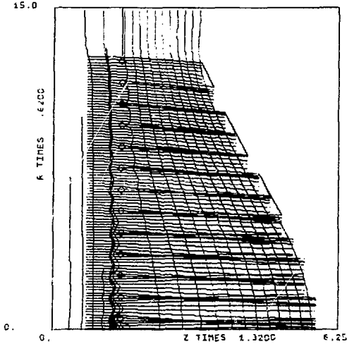
TITLE CELL 0.25 X 0.25 CM PHASE SPACE FROM WIRE MESH GRID WIRE ANALYSIS ANODE A1 250 KV EQUIPOTENTIAL LINE X7UCIO2 07 MAR 79
