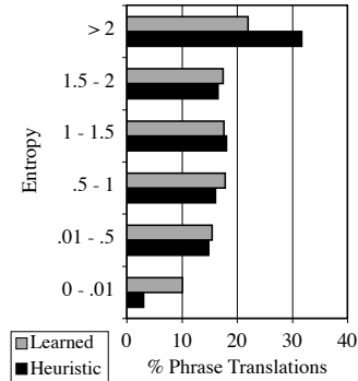
Figure 3.5: Many more French phrases have very low entropy under the learned parameterization.
