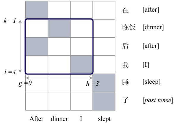
Figure 5.1: A^* search for pseudo-gold ITG alignments uses an admissible heuristic for bispan that counts the number of gold links outside of f_{[k:\ell]} but within e_{[g:h]} . Above, the heuristic is 1, which is also the minimal number of alignment errors that an ITG alignment will incur using this bispan.
