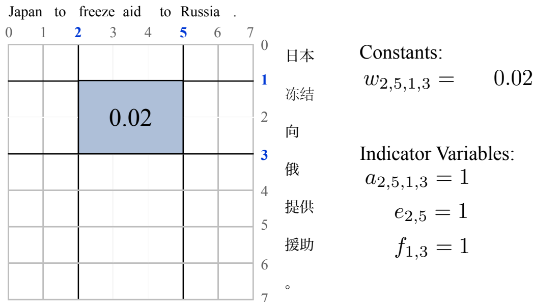
Figure 3.3: This example depicts the indicator variables and constants in the integer linear program construction of \mathcal{O} that must be set in order to properly describe the inclusion of the single shaded bispan above.
