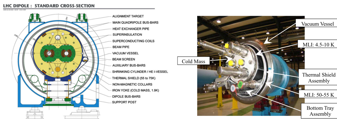
Figure 5.4. Diagram of the cross-section of the twin-bore LHC dipole magnets (left) and an image of an actual LHC dipole magnet (right), reproduced from Ref. [35].
