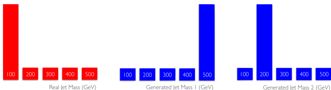
Figure D.1. Example real and generated jet mass distributions used to illustrate the benefit of IPMs in Appendix D.1, based on Refs. [63, 64].
