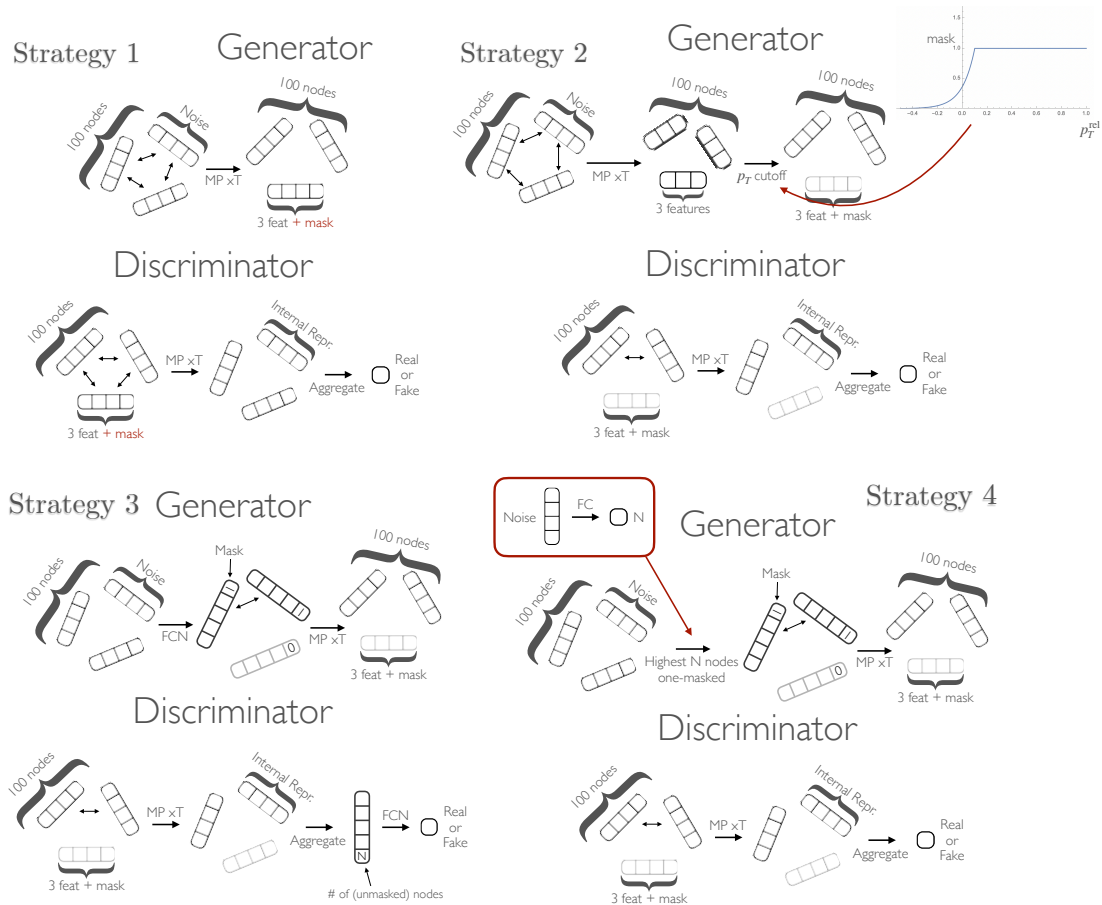
Figure C.3. The four alternative masking strategies which we test.
