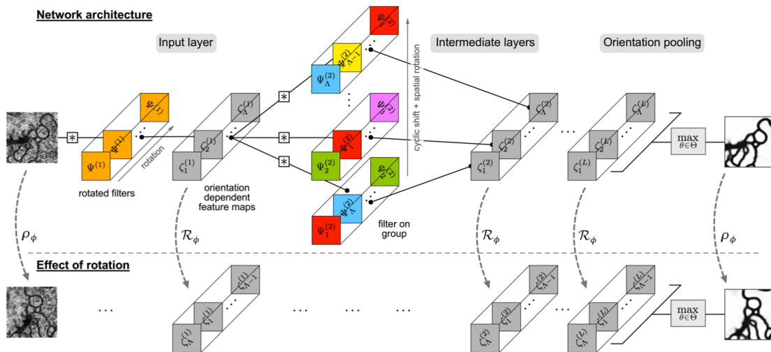
Figure 7.8. Schematic of a steerable CNN, reproduced from Ref. [52].
