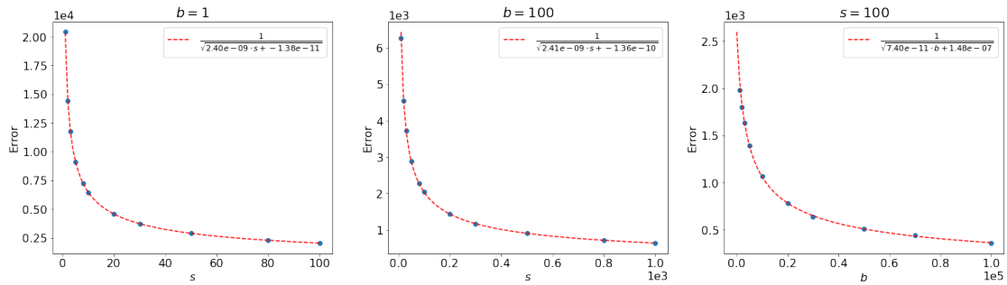
Figure 8.24. Error between the sampled toy distributions, using 50,000 toys each, and the asymptotic distributions of the MLE of \mu for different s and b (blue), with 1/\sqrt{N} fits in red.
