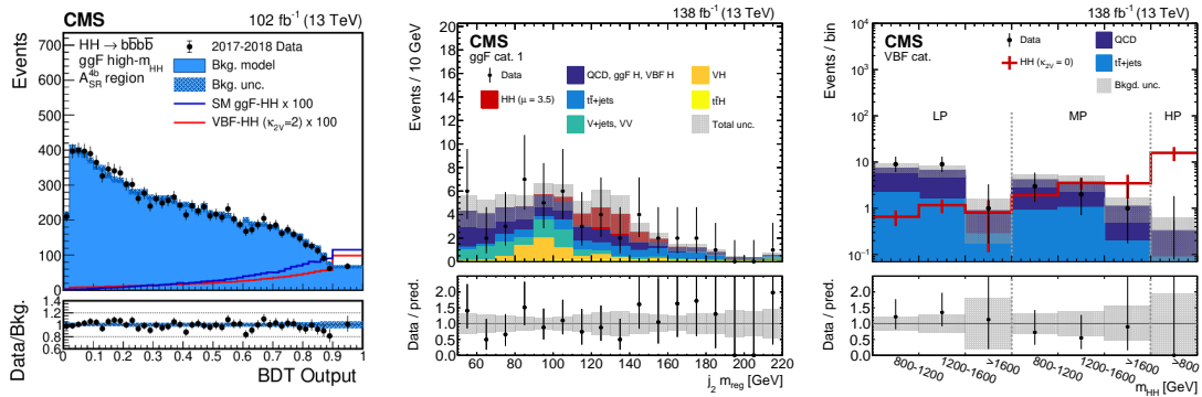
Figure 4.25. Distribution of events in the high- m_{HH} ggF category of the Run 2 CMS HH \rightarrow b\bar{b}b\bar{b} resolved analysis [28] as a function of the BDT discriminant (left), and of the Run 2 boosted analysis' [162] most sensitive ggF category, as a function of the second-highest tagged bb -jet's mass (middle), and VBF categories, as a function of m_{HH} (right).
