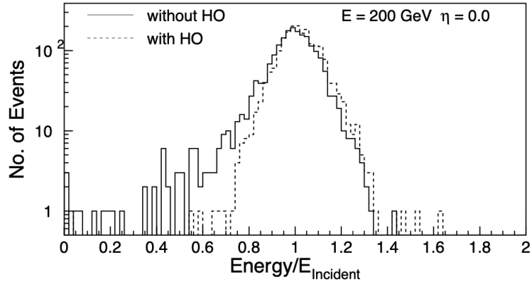
Figure 6.12. Simulation of the distribution of measured / incident energy for pions with incident energies of 200 GeV at \eta = 0 , reproduced from Ref. [46]. Without the HO, there is an excess of events with the measured energy lower than the incident, while with the HO the distribution is a Gaussian centered at 1, implying recovery of the total pion shower energy.
