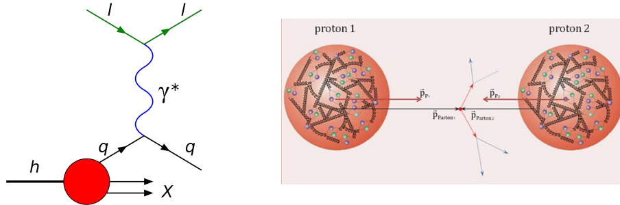
Figure 4.7. Feynman diagram for deep inelastic scattering, reproduced from Ref. [12] (left) and an illustrative example of proton-proton collisions reproduced from Ref. [13] (right).
