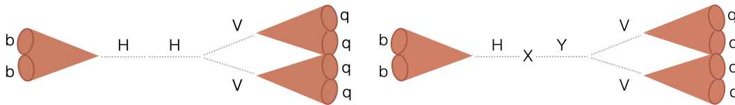
Figure 14.1. The boosted HH \rightarrow b\bar{b}(VV \rightarrow 4q) (left) and X \rightarrow (H \rightarrow b\bar{b})(Y \rightarrow VV \rightarrow 4q) (right) processes.
