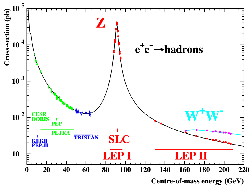
Figure 3.3. Cross section for e^+e^- \rightarrow \text{hadron} scattering as a function of \sqrt{s} with a clear resonance at the Z boson mass, reproduced from Ref. [2].
