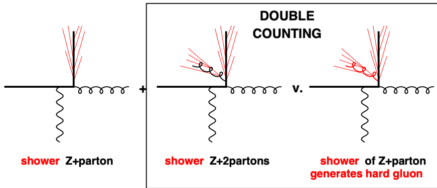
Figure 4.14. An illustration of double-counting when combining matrix element predictions (in black) with parton showering algorithms (in red) for Z +parton and Z +2-parton events, reproduced from Ref. [21].
