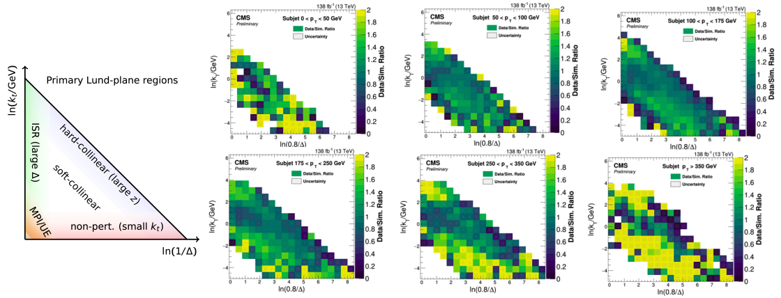
Figure 13.4. Regions of the primary Lund plane (left) and data versus MC Lund plane ratios in W \rightarrow q\bar{q} jets, binned in subjet p_T (right), reproduced from Refs. [61] and [62], respectively.
