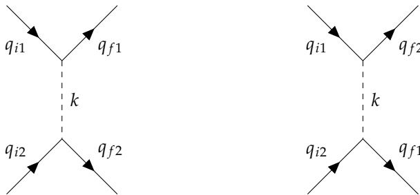
Figure B.2. The two lowest order nucleon scattering diagrams.
