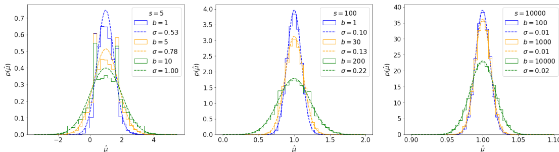
Figure 8.21. Gaussian fits to distributions of \hat{\mu} for different s and b from Figure 8.20.
