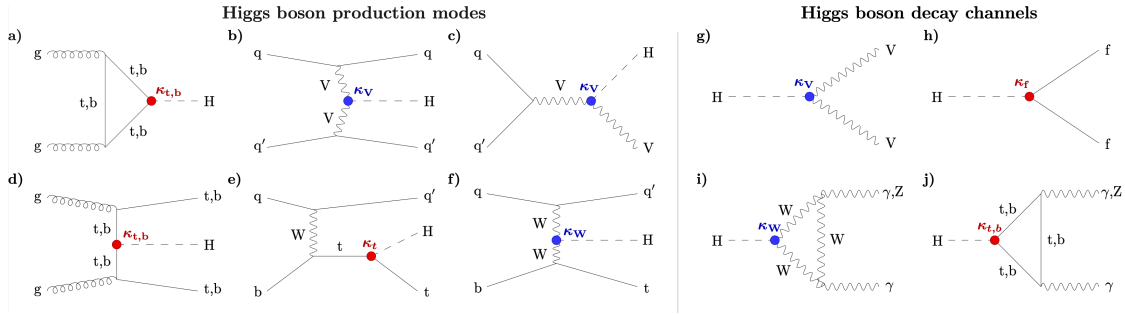
Figure 4.17. Single Higgs boson production modes and decay channels at the LHC, reproduced from Ref. [23].
