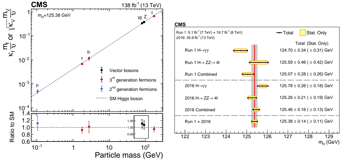
Figure 4.19. Constraints on Higgs to fermion and vector boson couplings, reproduced from Ref. [23] (left) and measurements of the Higgs mass, reproduced from Ref. [26] (right) by the CMS experiment.
