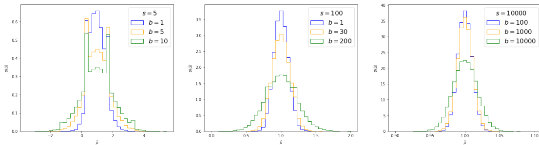
Figure 8.20. Distribution of the MLE of \mu for different s and b produced using 30,000 toy experiments each. (Note the x-axis range is becoming narrower from the left-most to the right-most plot.)
