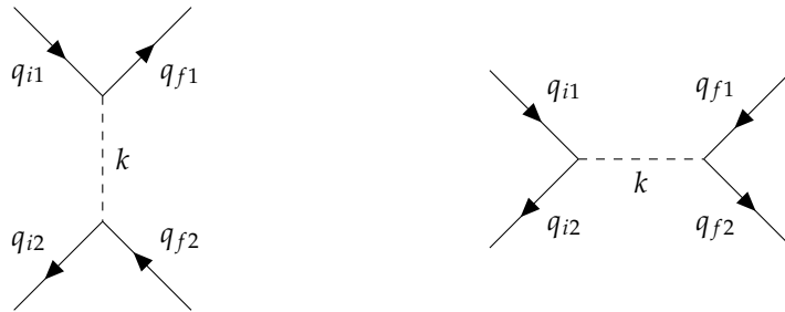
Figure 3.2. The two lowest order nucleon-antinucleon scattering diagrams.
