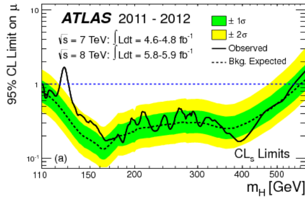
Figure 8.19. Expected and observed 95% CL_s upper limits for the SM Higgs by ATLAS in 2012, for different hypothetical Higgs masses [60].
