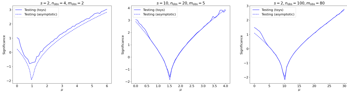
Figure 8.29. Comparing the significances, as a function of the signal strength \mu of the hypothesis being tested, for simple counting experiments (Eq. 8.2.3) with different s, n_{\text{obs}}, m_{\text{obs}} 's, derived using 30,000 toys each (solid) to estimate the p(t_\mu|\mu) distribution vs. the asymptotic approximation (dashed).
