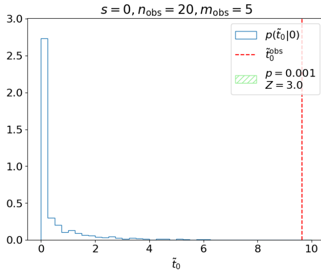
Figure 8.9. Testing the background-only hypothesis in Example 8.2.1.
