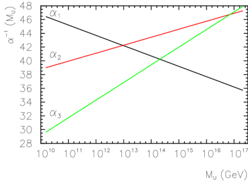
Figure 3.6. The running of the inverse strength of the SM coupling constants, with the strong coupling constant (SU(3)) in green, weak (SU(2)) in red, and electromagnetic (U(1)) in black, reproduced from Ref. [4].
