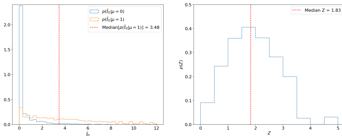
Figure 8.15. Left: Distributions of \tilde{t}_0 under the background-only and background + signal hypotheses using 30,000 toys each. The median of the latter is marked in red. Right: Distribution of the significances (with respect to the background-only hypothesis) of each sampled \tilde{t}_0 under the signal hypothesis.
