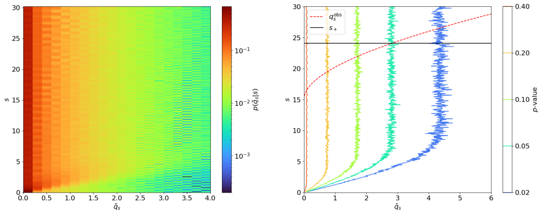
Figure 8.13. Extending the Neyman construction to an upper limit on s . Left: Scanning the upper limit test statistic distribution p(\tilde{q}_s|s) using 10,000 toys each for different values of s . Right: Converting this to a contour plot of the p -values for different \tilde{q}_s 's as a function of s , with the observed q_s^{\text{obs}} in red. The point at which q_s^{\text{obs}} intersects with the p -value = 0.05 contour is marked in black and signifies the upper limit at 95% CL.
