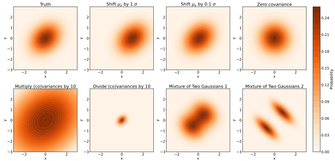
Figure 11.1. Samples of (mixtures of) Gaussian distributions used for testing evaluation metrics.
