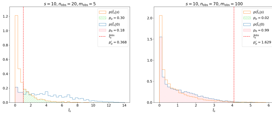
Figure 8.14. Demonstration of \text{CL}_s criterion for Examples 8.2.1 (left) and 8.2.2 (right).
