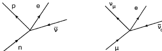
Figure 4.16. Feynman diagrams for beta decay (left) and muon decay (right) in Fermi’s theory.
