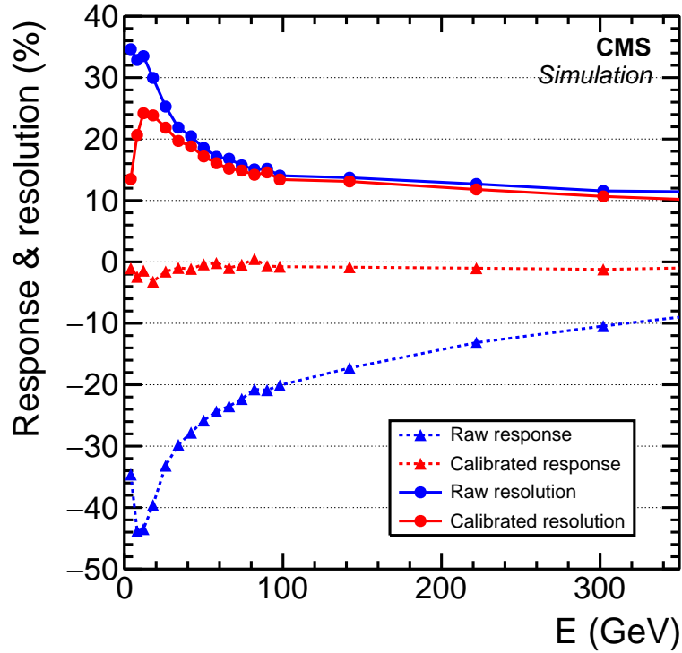
Figure 6.14. Response and resolution of single neutral hadron energies in the barrel as a function of the true energy, before and after calibration, reproduced from Ref. [48].
