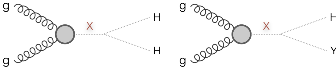
Figure 4.31. X \rightarrow HY production in the symmetric (left) and asymmetric (right) cases.
