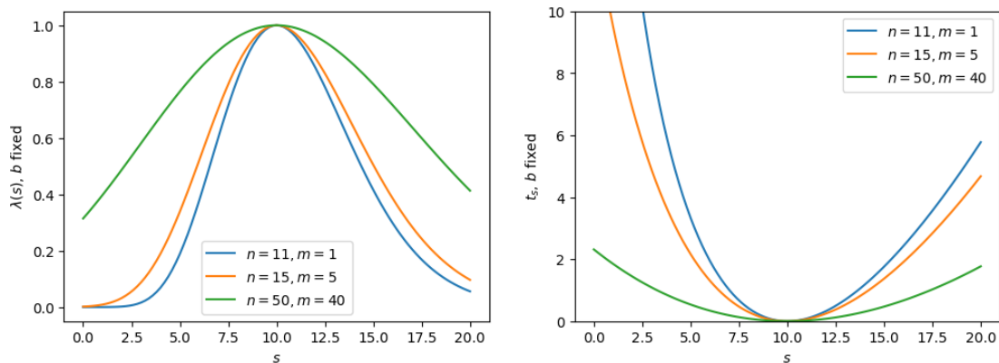
Figure 8.3. The profile likelihood ratio \lambda(s) (left) and the t_s test statistic (right) with b = m , demonstrating the effect of decreasing uncertainties on our nuisance parameters.
