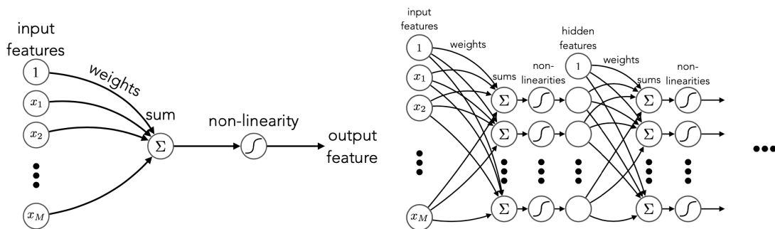
Figure 7.3. (Left) a single perceptron and (right) a neural network built using multiple layers of perceptrons (MLPs).
