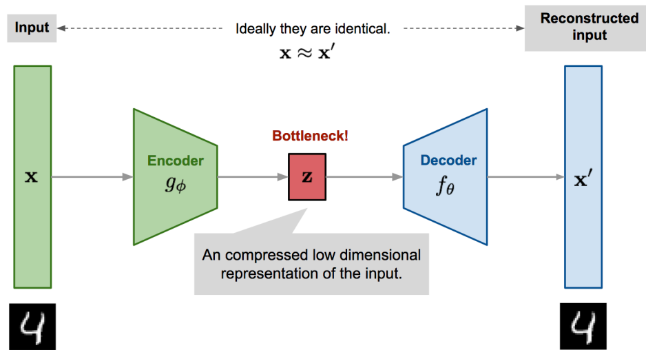
Figure 7.11. Diagram of an image autoencoder, reproduced from Ref. [55].
