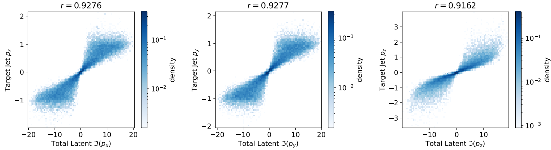
Figure 16.5. The correlations between the total momentum of the imaginary components in the \tau_{(1/2,1/2)} = 2 LGAE-Mix model and the target jet momenta. The Pearson correlation coefficient r is listed above.
