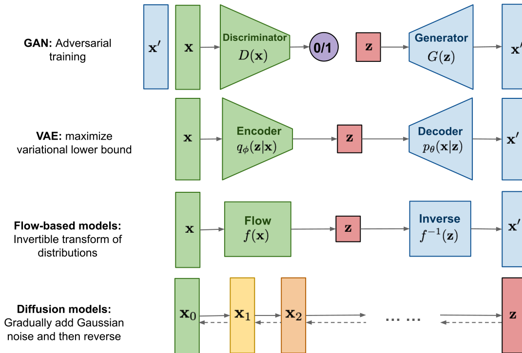
Figure 7.12. Summary of popular generative models, reproduced from Ref. [56].
