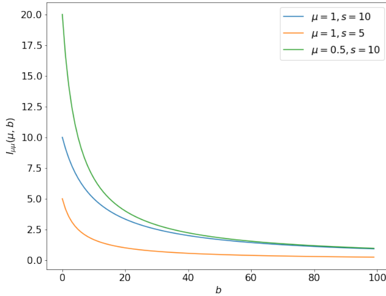
Figure 8.22. The Fisher information \mathcal{I}_{\mu\mu}(\mu, b) for different \mu and s , as a function of the expected background b .
