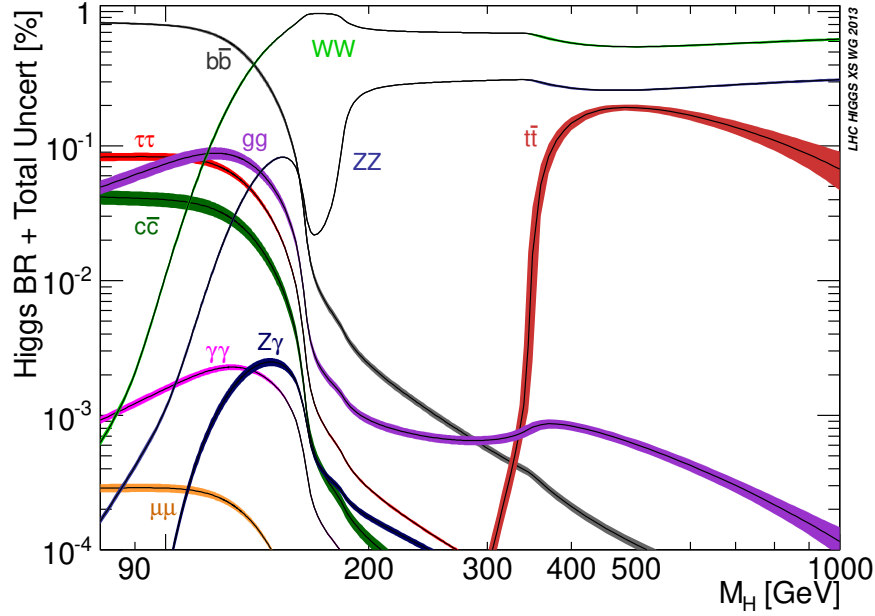
Figure 4.18. Higgs branching fractions predicted in the SM as a function of m_H (reproduced from Refs. [24, 25]).
