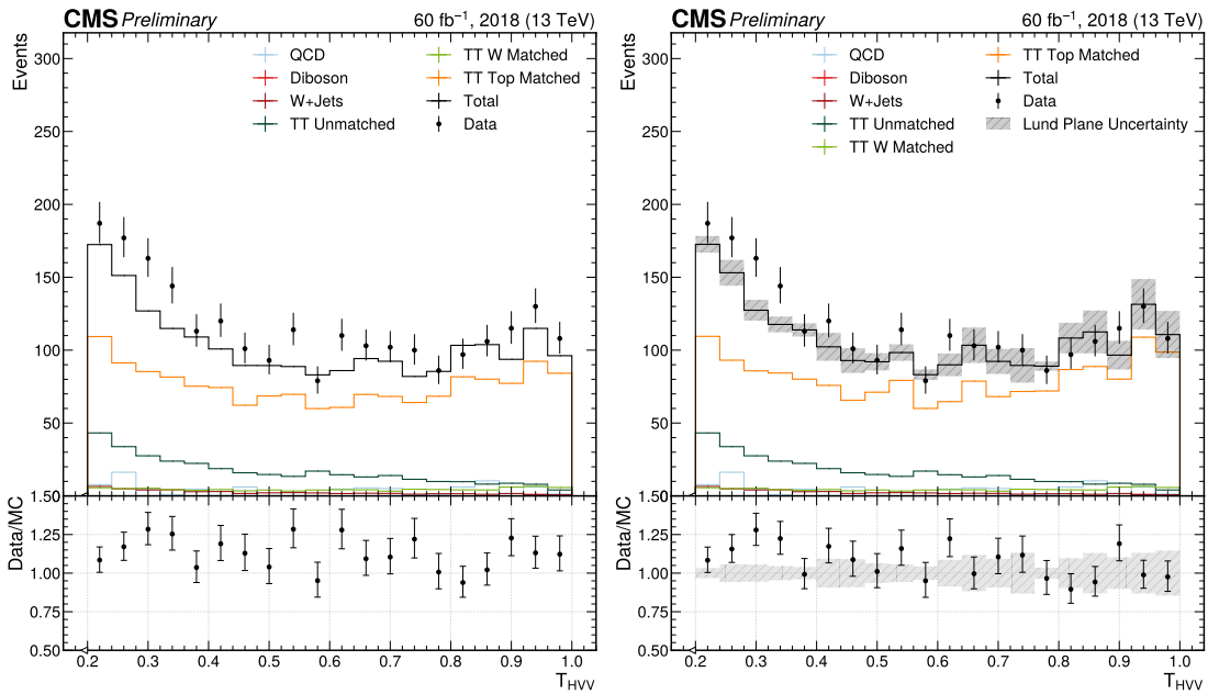
Figure 13.5. Distributions of the GloParT T_{\text{HVV}} discriminant before (left) and after (right) the Lund plane reweighting of top matched jets. The combined uncertainties from Lund-plane-based scale factors on the MC yield per bin are shown in gray on the right.
