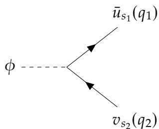
Figure B.3. Tree-level Feynman diagram for meson decay via a Yukawa interaction.
