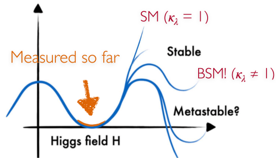
Figure 4.20. Cartoon of the Higgs potential in the SM and potential deviations due to BSM physics.
