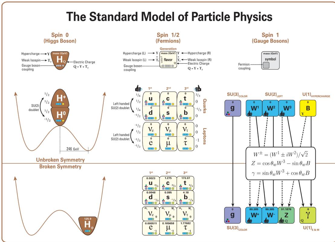
Figure 4.1. A graphical summary of the SM, reproduced from Ref. [6].
