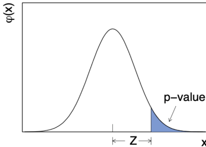
Figure 8.8. Relationship between significance Z and the p -value, reproduced from Ref. [58].
