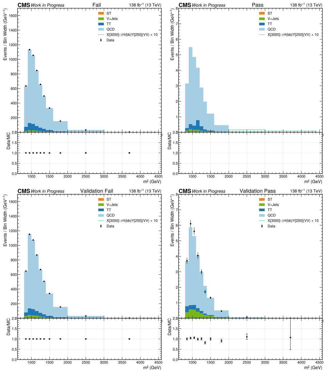
Figure 14.7. Post-background-only-fit distributions in the fully-merged category of the VV-candidate jet regressed mass ( m_{reg}^{VV} ) in the validation fail (bottom left), and validation pass (bottom right) regions, as well as distributions in the pass region after applying the post-fit transfer factor from the validation regions (top right), and the fail region (top left). The data is not shown in the pass region.
