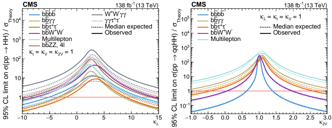
Figure 4.30. The expected and observed limits on the ratio of experimentally estimated production cross section and the theory expectation for different values of \kappa_\lambda (left) and \kappa_{2V} (right), reproduced from Ref. [32].
