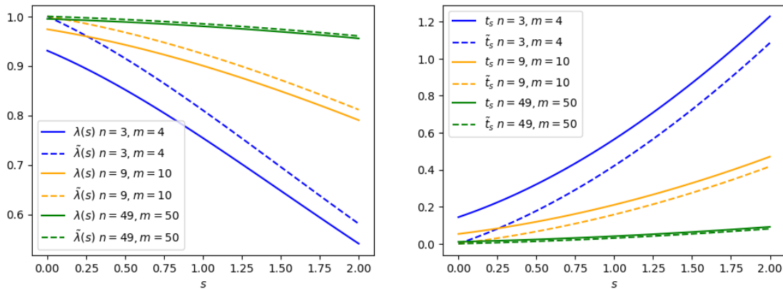
Figure 8.4. Comparing the nominal vs alternative test statistic.
