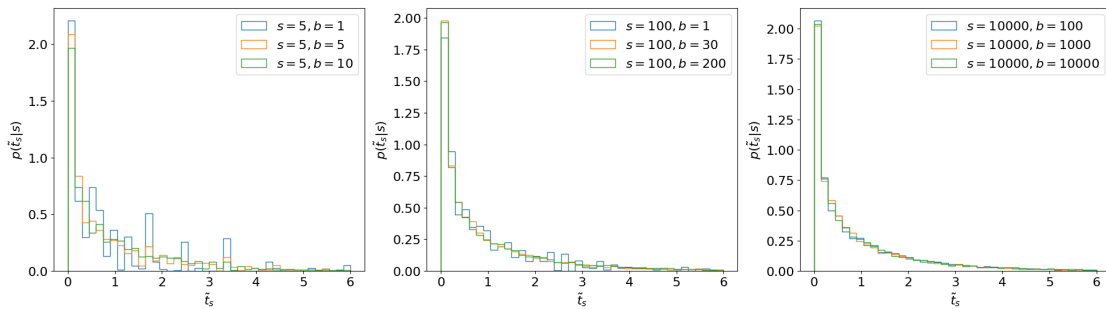
Figure 8.5. Estimating p(\tilde{t}_s|s) through toys.
