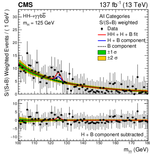
Figure 4.27. Invariant two-photon mass distribution of the Run 2 CMS HH \rightarrow b\bar{b}\gamma\gamma analysis [30], combined for all signal categories, weighted by S/(S+B) , where S ( B ) is the number of signal (background) events extracted from the signal-plus-background fit.
