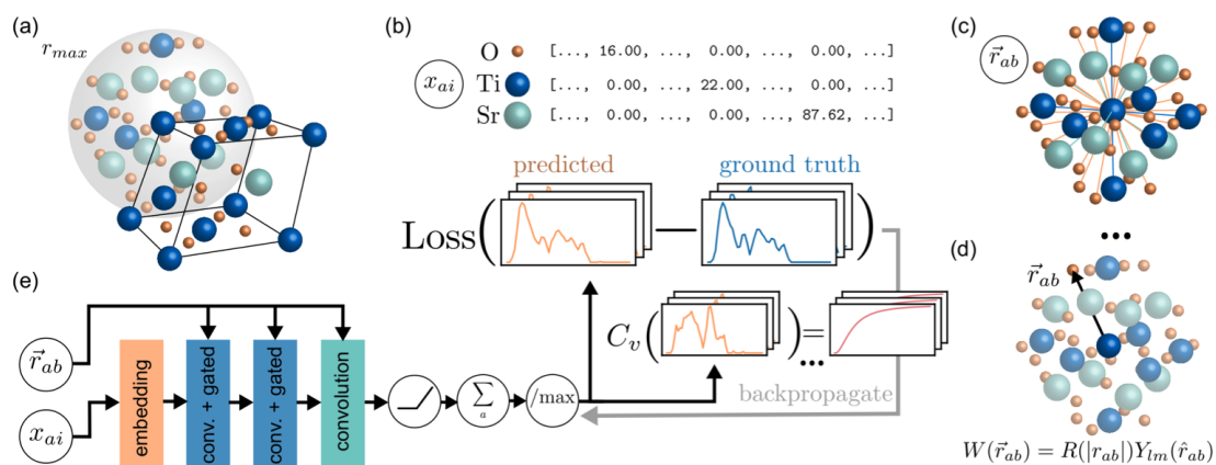
Figure 7.9. Schematic of the E(3)-equivariant neural network architecture used for predicting phonon density of states, reproduced from Ref. [53].
