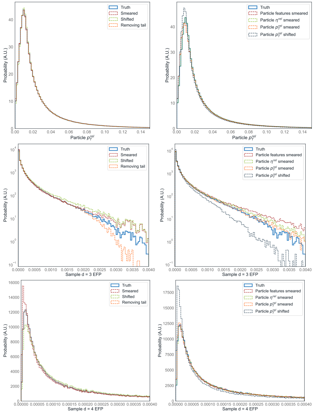
Figure D.5. The probability, in arbitrary units (A.U.), of the particle p_T^{\text{rel}} , a sample d = 3 EFP, and a sample d = 4 EFP for truth and distorted gluon jet distributions. On the left are distribution-level distortions, and on the right particle-level.
