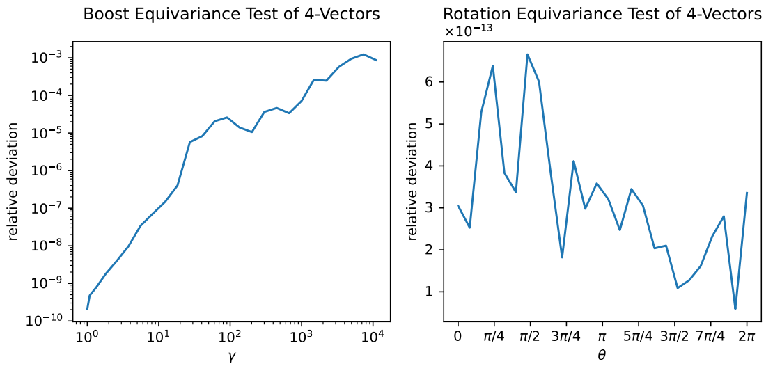
Figure E.2. The relative deviations, as defined in Eq. E.3.1, of the output 4-momenta p^\mu to boosts along the z -axis (left) and rotations around the z -axis (right).
