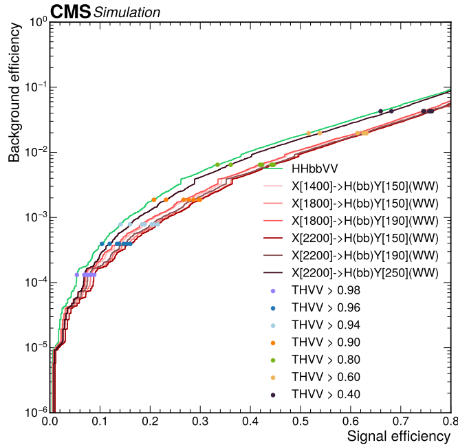
Figure 13.3. Receiver operating characteristic (ROC) curve for the T_{\text{HVV}} discriminator on VV-candidate jets passing the AK8 online and offline selections for a subset of nonresonant and resonant signals versus QCD and t\bar{t} backgrounds.
