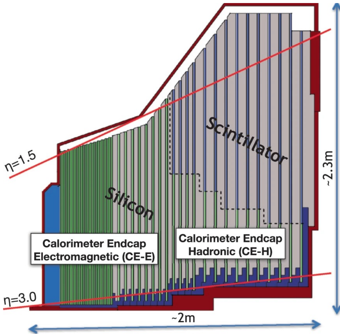
Figure 6.15. Layout of the CMS HGCAL, reproduced from Ref. [49].
