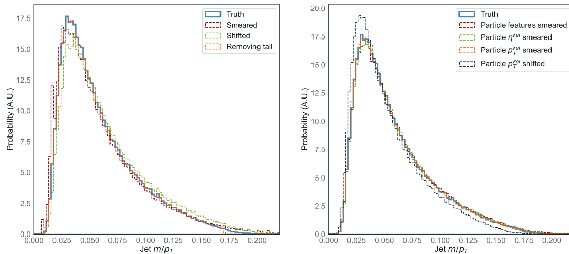
Figure 11.3. The probability, in arbitrary units (A.U.), of the relative jet mass for truth and distorted gluon jet distributions. On the left are distribution-level distortions, and on the right particle-level.
