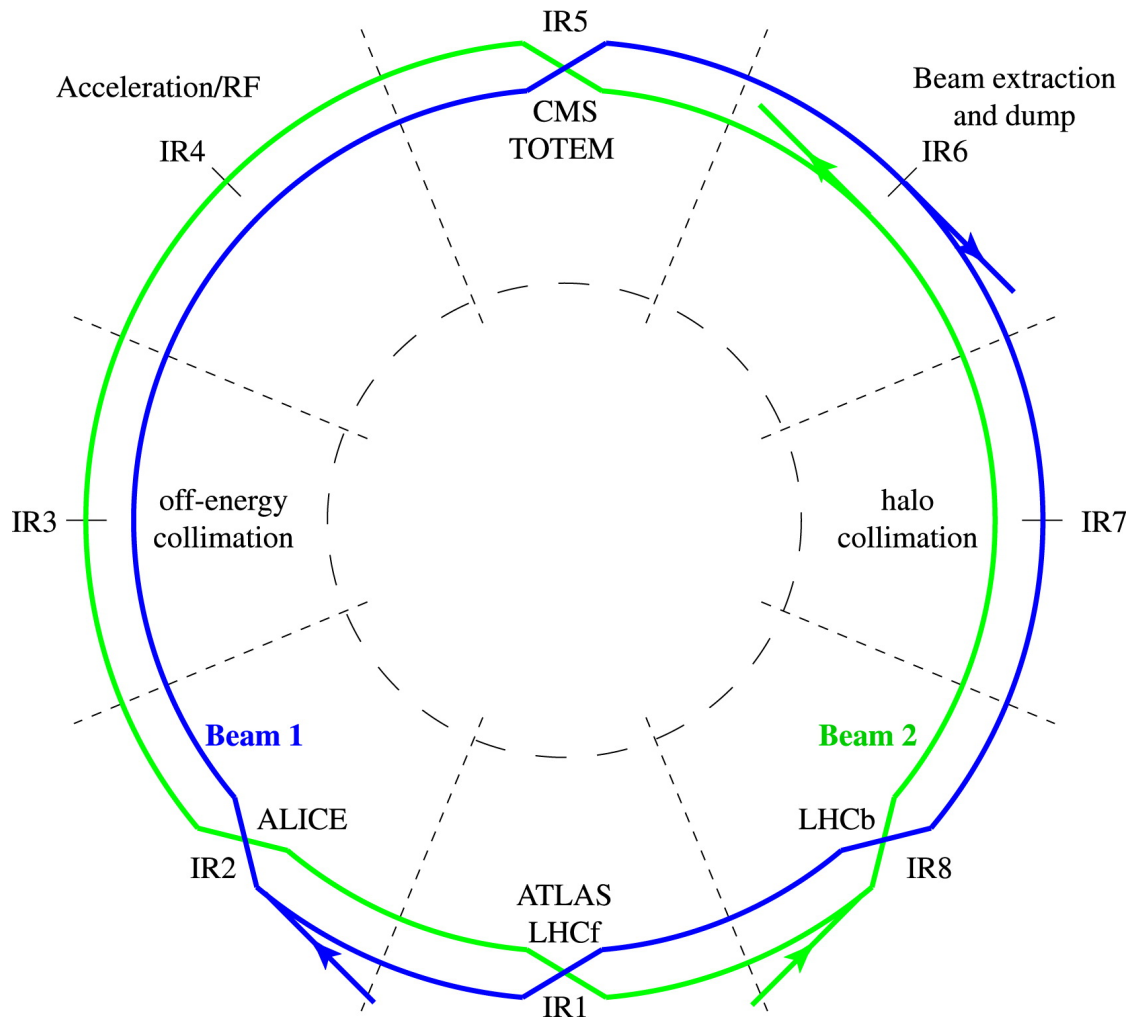
Figure 5.5. Schematic of the LHC layout showing the two proton beams in green and blue and its division into eight octants, reproduced from Ref. [34].
