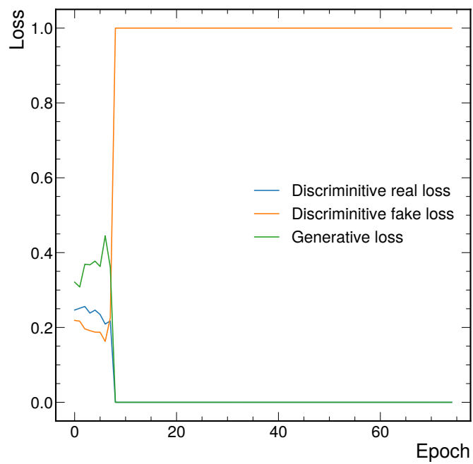
Figure C.4. Loss curve of a training on light quark jets with masking strategy 3, typical of loss curves with all four strategies.
