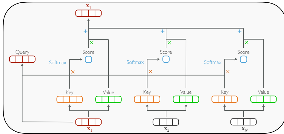
Figure 7.6. Schematic of set self-attention.
