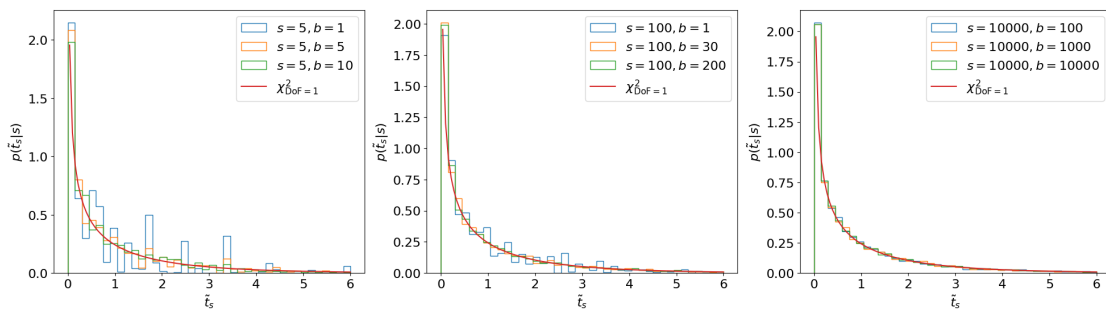
Figure 8.6. Asymptotic form of p(\tilde{t}_s|s) .
