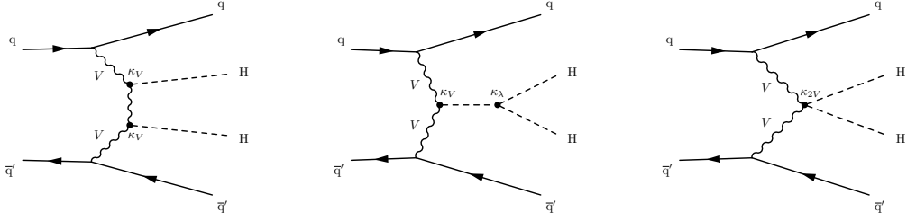
Figure 4.22. Leading-order diagrams for nonresonant HH production via vector boson fusion. In this chapter, we refer to the left-most VBF diagram as the (\text{HVV})^2 and the right-most as the HHVV diagram.
