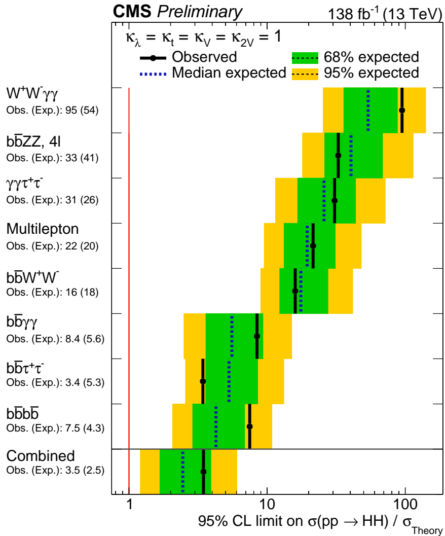
Figure 4.29. The expected and observed limits on the ratio of experimentally estimated production cross section and the expectation from the SM in searches using different final states and their combination, reproduced from Ref. [32]. The search modes are ordered, from upper to lower, by their expected sensitivities from the least to the most sensitive. The overall combination of all searches is shown by the lowest entry.
