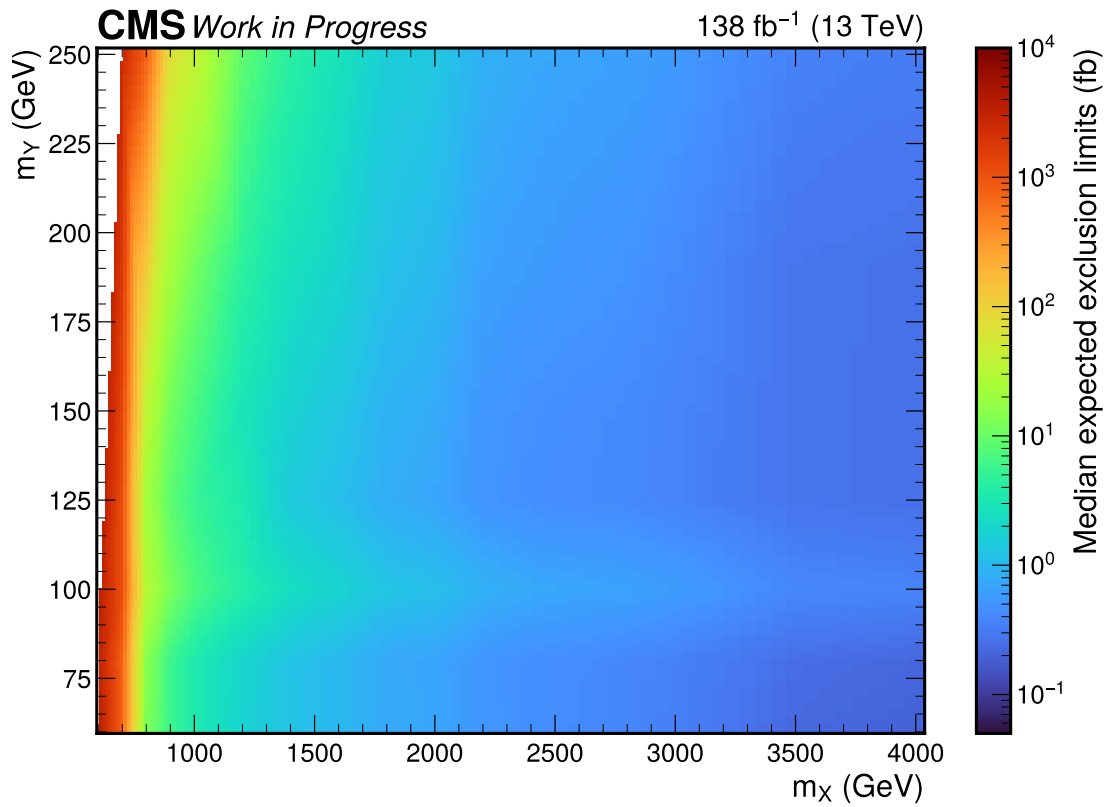
Figure 14.9. Median expected exclusion limits in the fully-merged category for resonant X \rightarrow (H \rightarrow b\bar{b})(Y \rightarrow VV \rightarrow 4q) signals for different m_X and m_Y .
