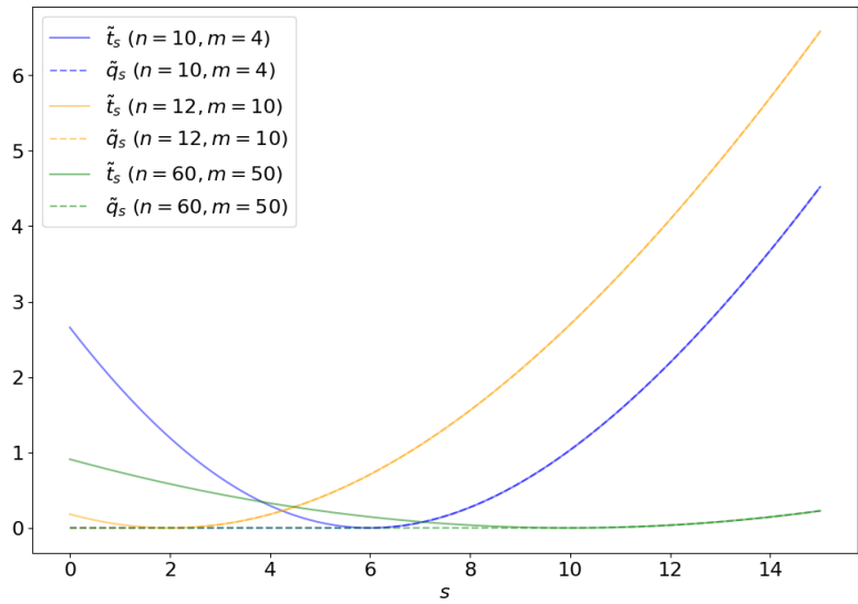
Figure 8.11. Comparing \tilde{t}_s and \tilde{q}_s .
