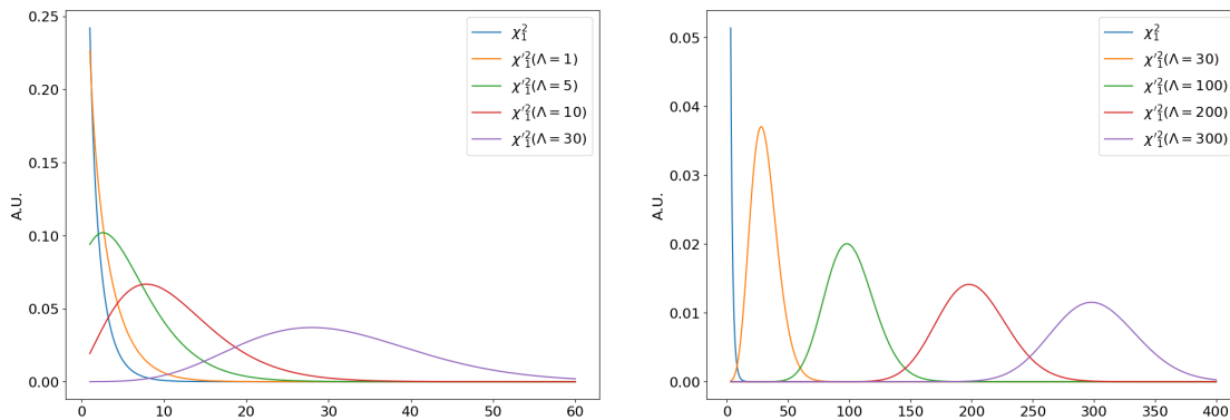
Figure 8.25. Central \chi_k^2 and non-central \chi_k'^2(\Lambda) distributions for \Lambda between 1 – 30 (left) and 30 – 300 (right).
