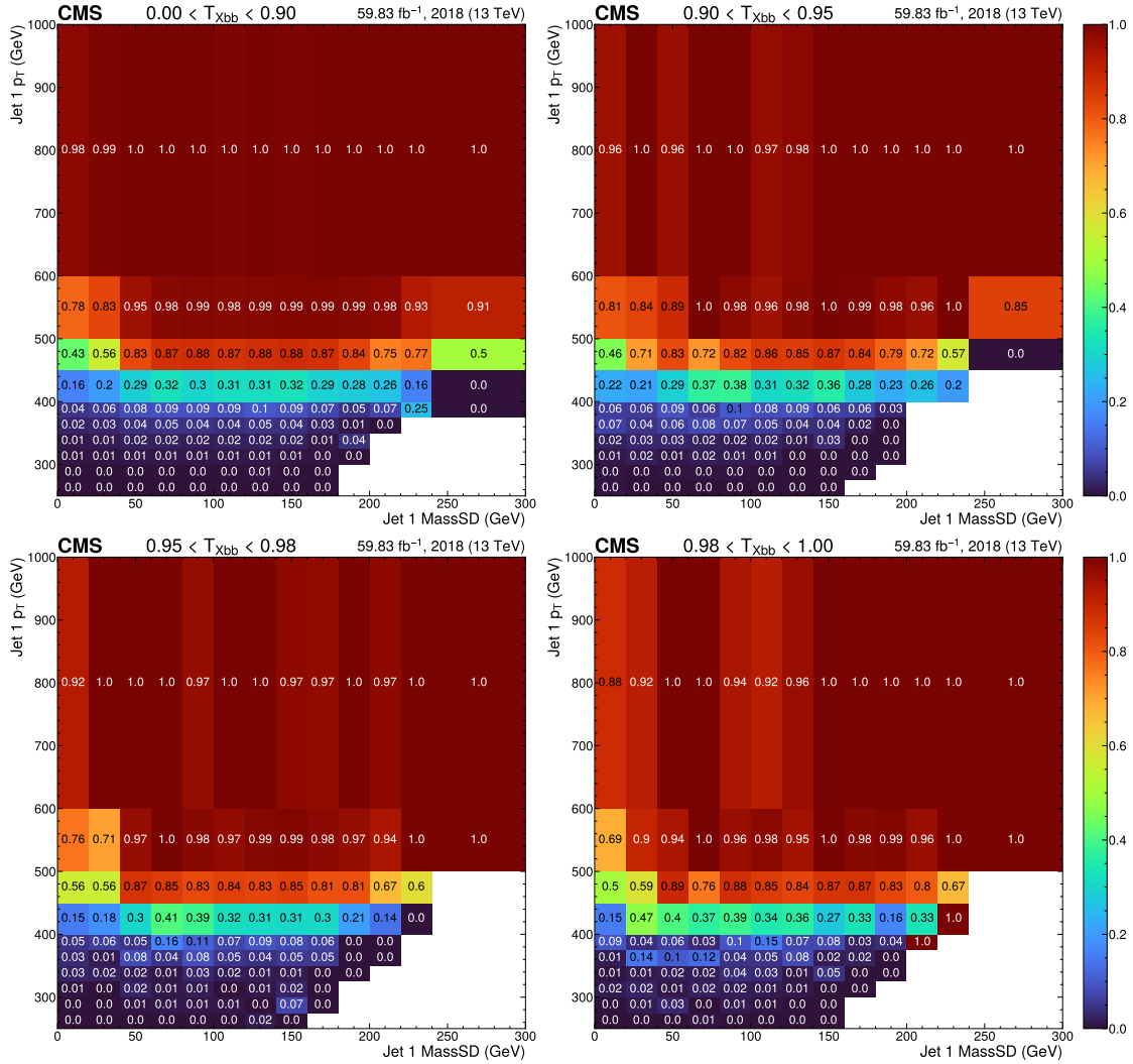
Figure 14.2. Trigger efficiencies for the 2018 dataset measured in bins of the AK8 jet p_T , soft drop mass (MassSD) and T_{Xbb} score.
