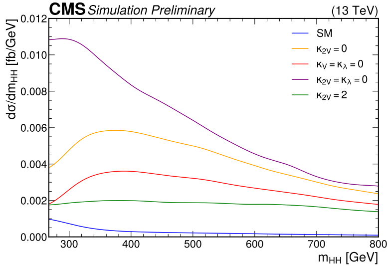
Figure 4.23. Differential cross section at 13 TeV center of mass for VBF HH production as a function of the invariant mass of the HH system ( m_{HH} ) for different diagrams and couplings.
