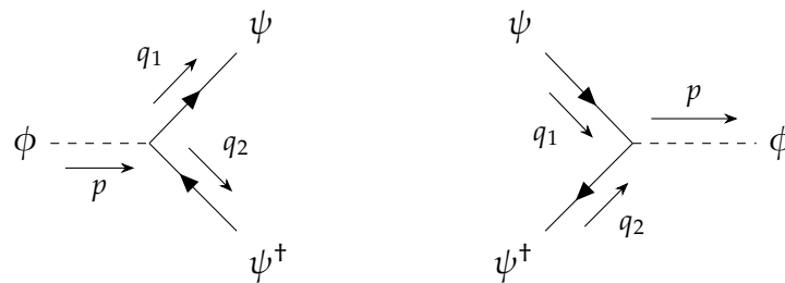
Figure 3.1. Feynman diagrams for meson decay (left) and nucleon-antinucleon annihilation (right).
