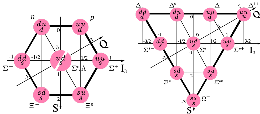
Figure 4.6. Baryons in the octet (left) and decuplet (right) representations of SU(3), reproduced from Ref. [11].
