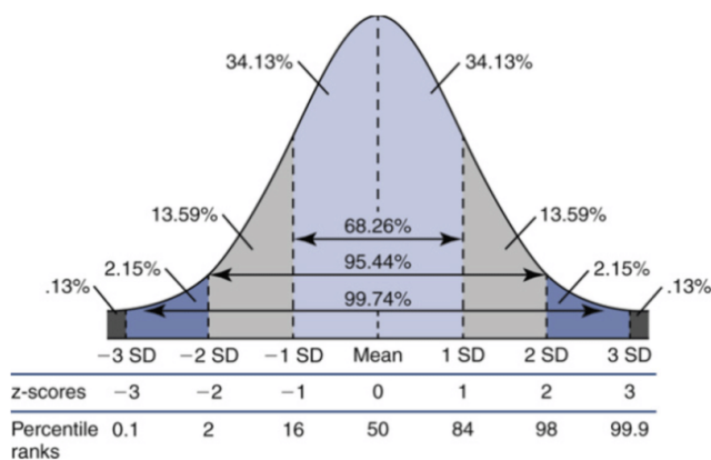
Figure 8.16. Gaussian quantiles, reproduced from Ref. [59].
