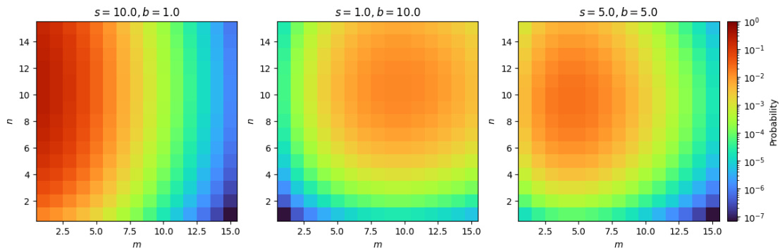
Figure 8.1. Sample 2D Poisson distributions.
