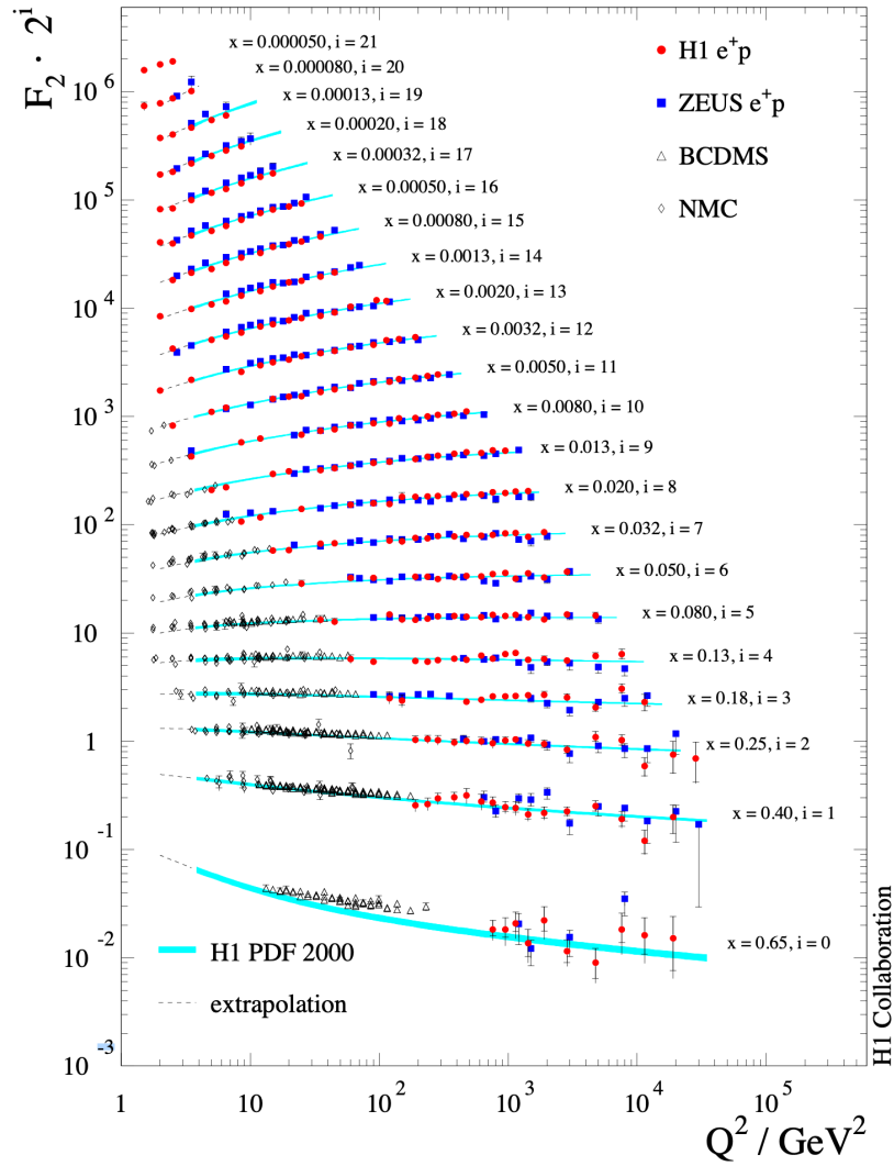
Figure 4.11. PDF measurements at different energy scales Q^2 and momentum fraction x by the H1 collaboration in DIS experiments, reproduced from Ref. [17].
