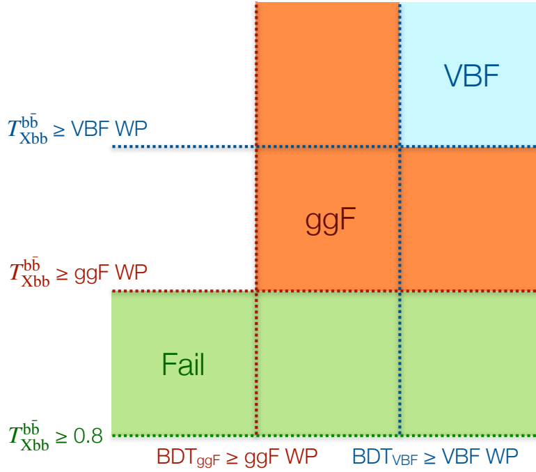
Figure 14.3. Illustration of the signal and fail nonresonant analysis region selections in terms of the T_{Xbb}^{bb} and BDT scores.
