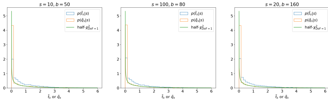
Figure 8.12. Comparing p(\tilde{t}_s|s) and p(\tilde{q}_s|s) . p(\tilde{q}_s|s) asymptotically follows a half- \chi^2 distribution (green).
