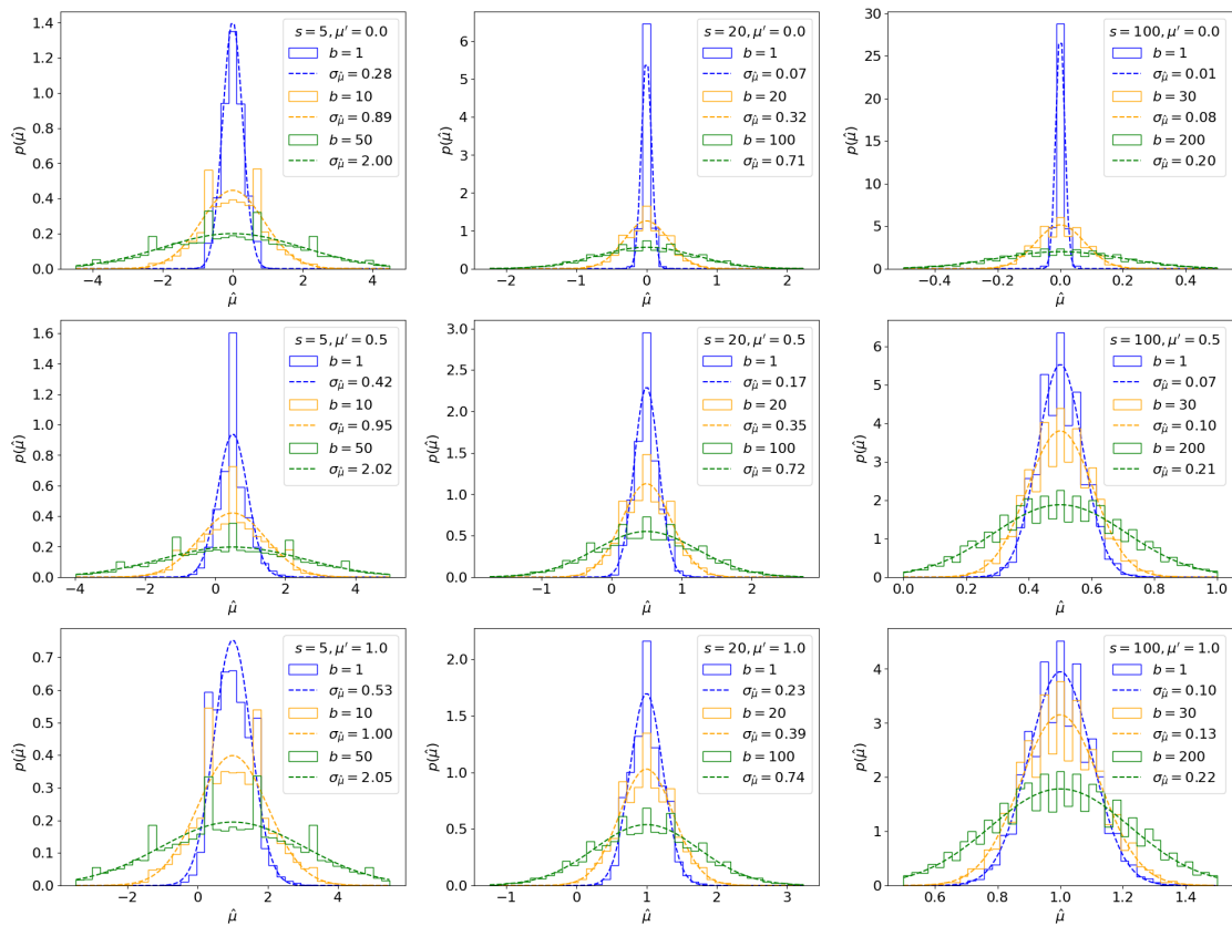
Figure 8.23. Asymptotic (dotted lines) and toy-based (solid lines) distributions, using 30,000 toys each, of the MLE of \mu for different s , b , and true signal strengths \mu' .
