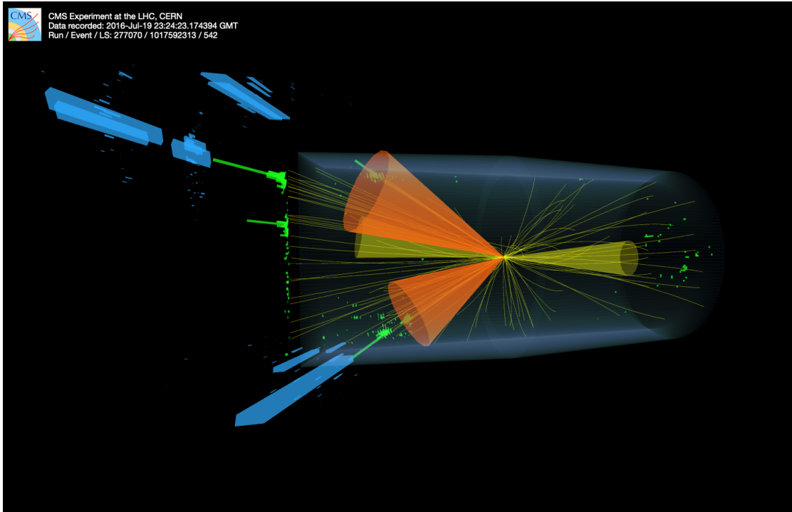
Figure 4.13. An example of real jets in an event collected by CMS and identified in the search described in Chapter 14 [19, 20]. An interactive version of this event display is available at https://cms3d.web.cern.ch/HIG-23-012/ .
