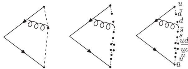
Figure 4.15. An illustration of the Lund string model of hadronization, reproduced from Ref. [22].
