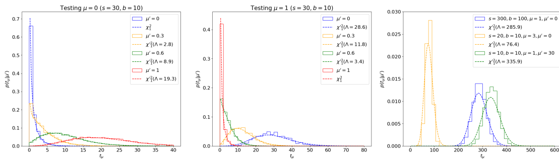
Figure 8.27. Comparing the sampling distribution p(t_{\mu}|\mu') with non-central \chi_1^2(\Lambda) distributions for a range of s, b, \mu, \mu' values, with the Asimov sigma estimation for \sigma_{\hat{\mu}}^2 .
