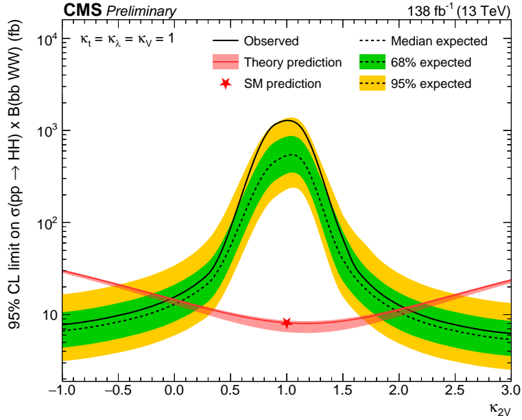
Figure 14.6. 1D upper limits scans on the inclusive HH cross section as a function of \kappa_{2V} .
