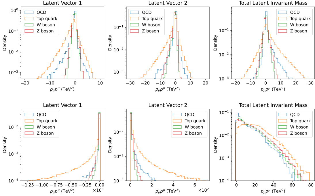
Figure 16.6. Top: distributions of the invariant mass squared of the latent 4-vectors and jet momenta of the LGAE-Mix with \tau_{(1/2,1/2)} = 2 latent 4-vectors. Bottom: distributions of the invariant mass squared of two latent 4-vectors and jet momenta of the LGAE-Min-Max with \tau_{(1/2,1/2)} = 2 latent 4-vectors.
