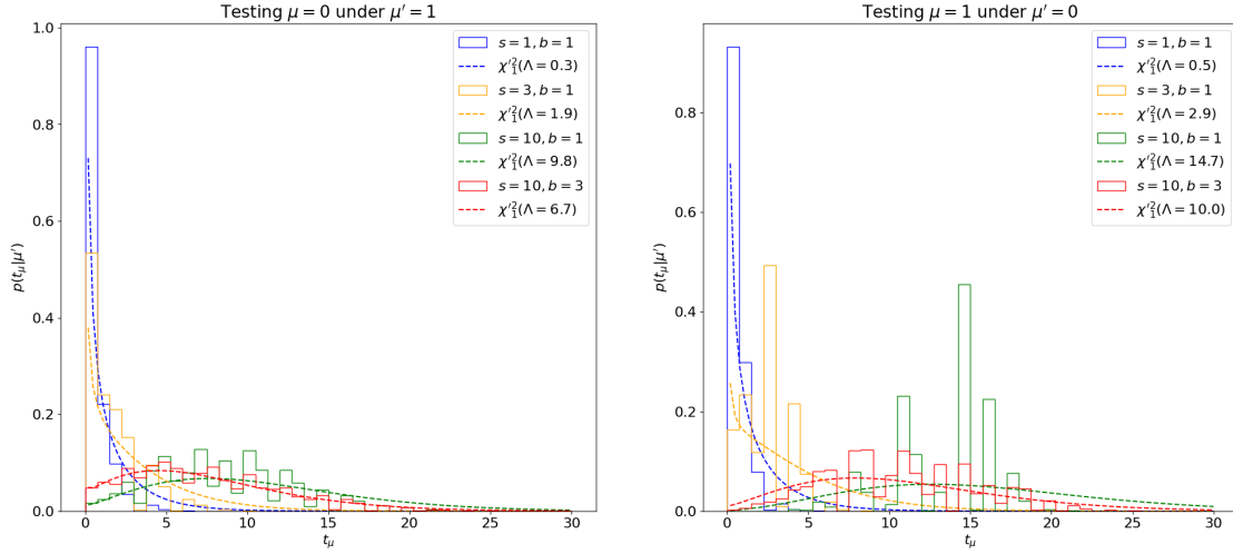
Figure 8.28. Comparing the sampling distribution p(t_\mu|\mu') with non-central \chi_1^2(\Lambda) distributions for different s, b \leq 10 , showing the break-down of the \sigma_A approximation for \sigma_{\hat{\mu}}^2 at low statistics.
