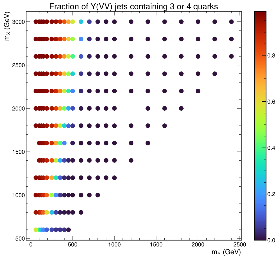
Figure 4.32. The fraction of Y \rightarrow VV jets containing three or four generator-level quarks for the resonant X \rightarrow (H \rightarrow b\bar{b})(Y \rightarrow VV) signal as a function of the X and Y boson masses.
