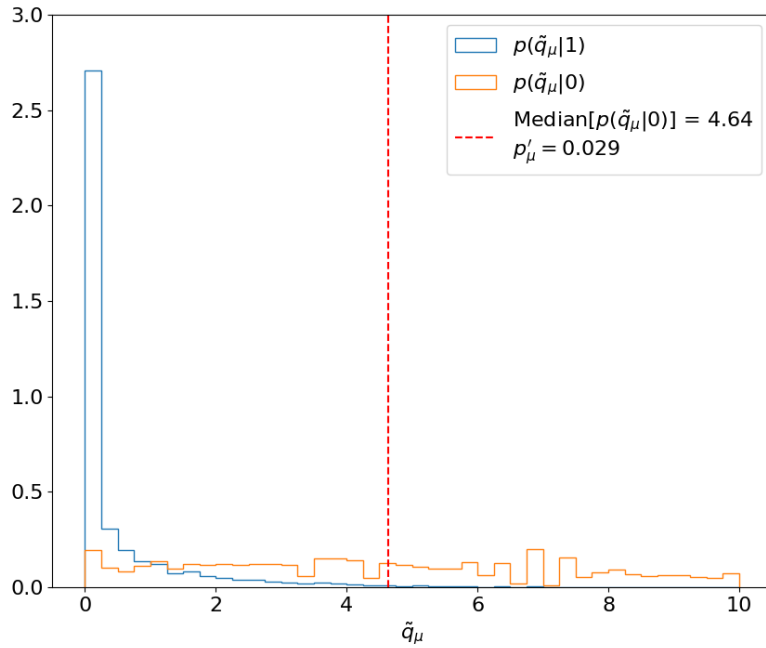
Figure 8.17. Calculating the median expected p'_{\mu=1} -value with respect to the signal + background hypothesis, for test statistics \tilde{q}_\mu sampled under the background-only hypothesis. p(\tilde{q}_\mu|1) and p(\tilde{q}_\mu|0) are estimated using 30,000 toys each. Then, the median p(\tilde{q}_\mu|0) (red) is used to calculate the p'_\mu -value following the \text{CL}_s criterion.
