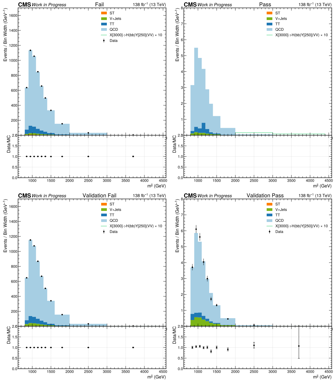
Figure 14.8. Post-background-only-fit distributions in the fully-merged category of the dijet mass ( m^{jj} ) in the validation fail (bottom left), and validation pass (bottom right) regions, as well as distributions in the pass region after applying the post-fit transfer factor from the validation regions (top right), and the fail region (top left). The data is not shown in the pass region.
