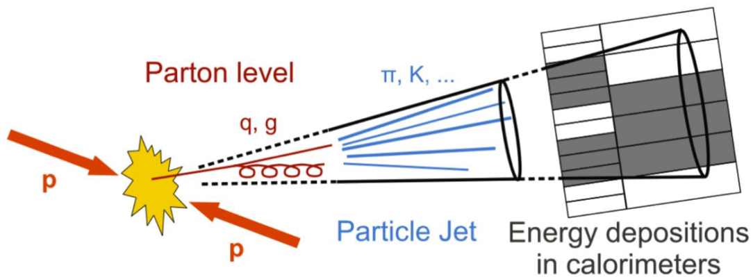
Figure 4.12. A cartoon of a jet, reproduced from Ref. [18].
