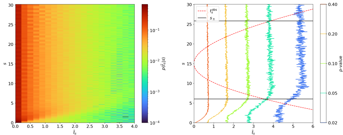
Figure 8.10. Demonstration of the Neyman construction for a 95% confidence interval for the experiment in Example 8.2.1 ( n_{\text{obs}} = 20, m_{\text{obs}} = 5 ). Left: Scanning p(\tilde{t}_s | s) using 10,000 toys each for different values of s . Right: Converting this to a contour plot of the p -values for different \tilde{t}_s 's as a function of s , with the observed t_s^{\text{obs}} in red. The points at which t_s^{\text{obs}} intersects with the p -value = 0.05 contour are marked in black and signify the limits of the 95% confidence interval for s - in this case, [6.0, 25.8] .
