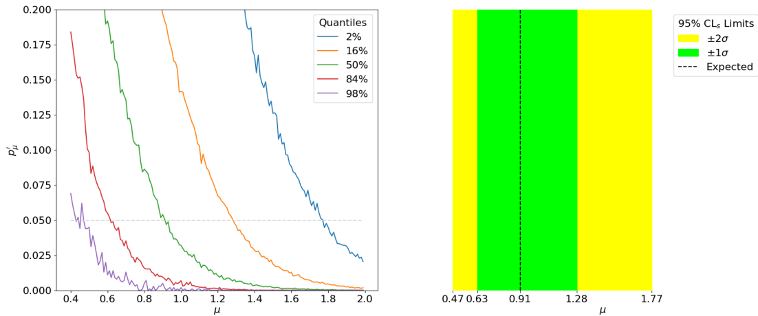
Figure 8.18. Left: The expected median and \pm 1\sigma , \pm 2\sigma quantiles of p'_\mu for different \mu 's. The intersection of these with p'_\mu = 0.05 (gray) corresponds to the expected exclusion limits. Right: The median and \pm 1\sigma , \pm 2\sigma expected limits at 95% CL s on \mu .
