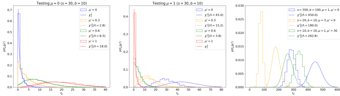
Figure 8.26. Comparing the distribution p(t_\mu|\mu') (solid) with non-central \chi_1^2(\Lambda) distributions (dotted) for a range of s, b, \mu, \mu' values, with \sigma_{\hat{\mu}}^2 estimated using the inverse of the Fisher information matrix.
