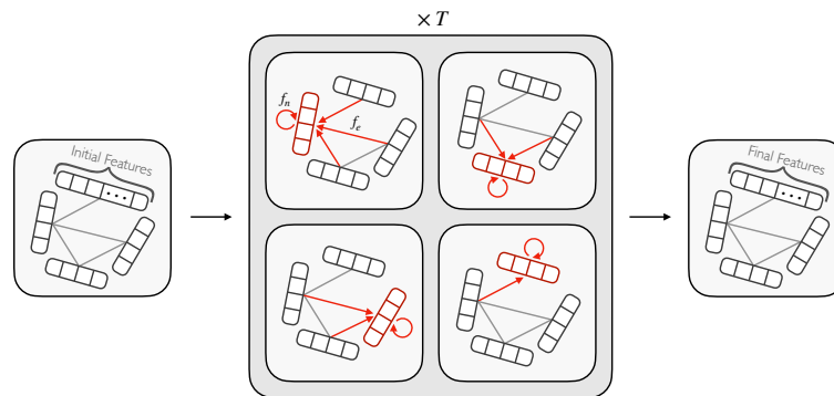
Figure 7.5. Schematic of a message passing graph neural network.
