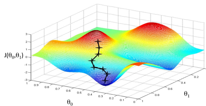
Figure 7.2. Illustration of gradient descent in a 2D parameter space of (\theta_0, \theta_1) .
