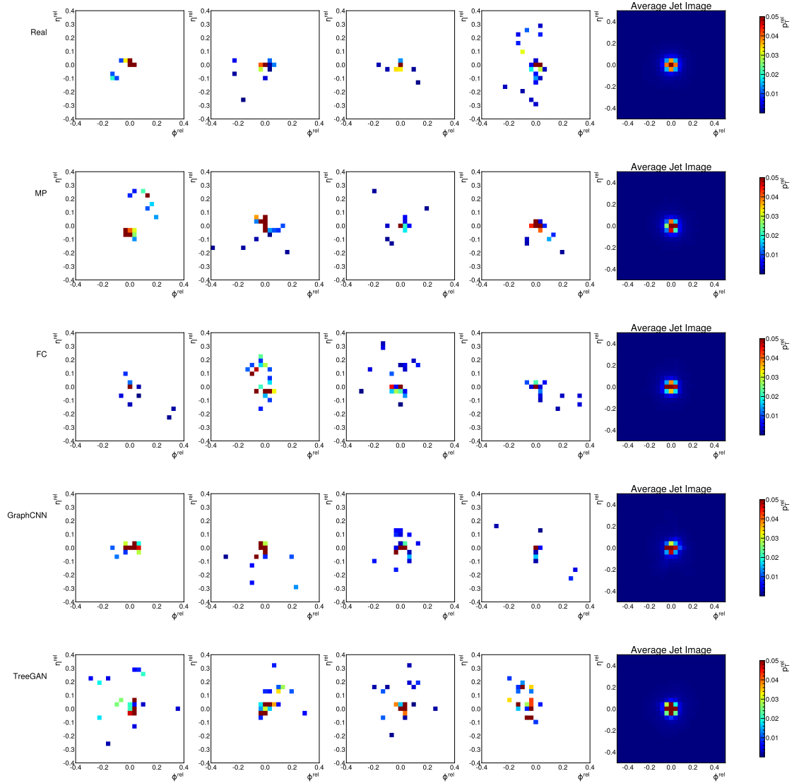
Figure 10.5. Random samples of discretized images in the \eta^{\text{rel}} - \phi^{\text{rel}} plane, with pixel intensities equal to particle p_{\text{T}}^{\text{rel}} , of real and generated light quark jets (left), and an average over 10,000 such sample images (right).
