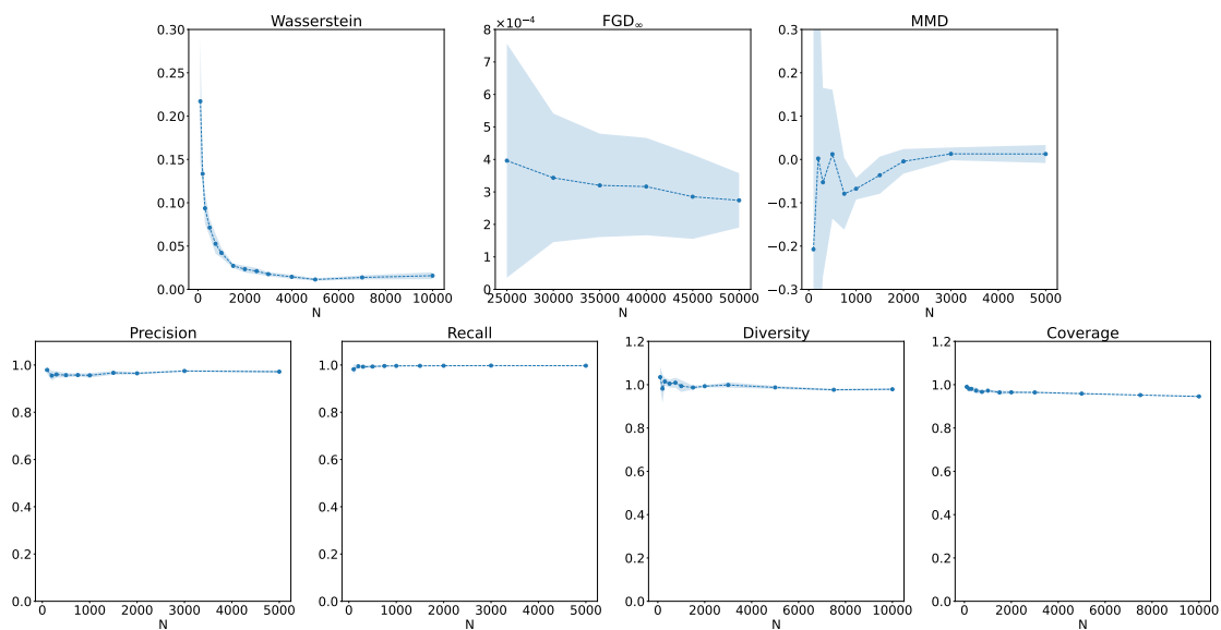
Figure 11.2. Scores of each metric on samples from the true distribution for varying sample sizes.
