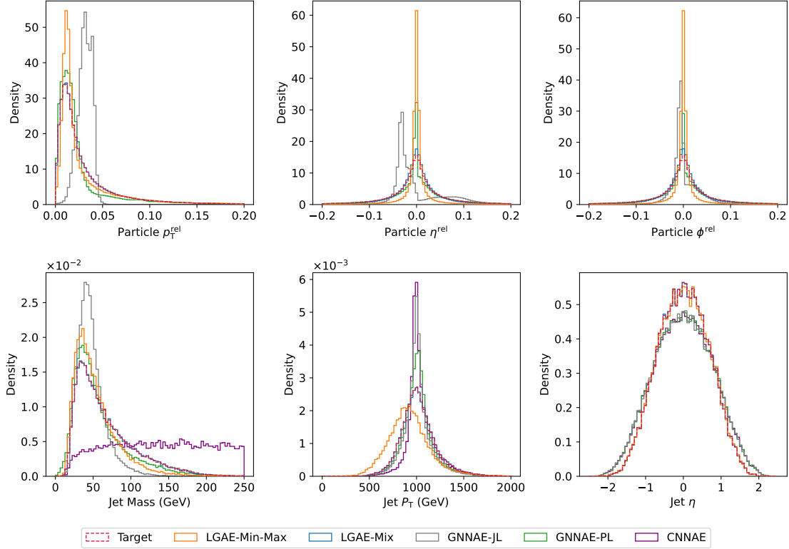
Figure 16.3. Top: particle momenta ( p_T^{\text{rel}}, \eta^{\text{rel}}, \phi^{\text{rel}} ) reconstruction by LGAE-Min-Max ( \tau_{(1/2,1/2)} = 4 , resulting in 56.67% compression) and LGAE-Mix ( \tau_{(1/2,1/2)} = 9 , resulting in 61.67% compression), and GNNAE-JL ( \dim(L) = 55 , resulting in 61.11% compression) and GNNAE-PL ( \dim(L) = 2 \times 30 , resulting in 66.67% compression). The reconstructions by the CNNAE are not included due to the discrete values of \eta^{\text{rel}} and \phi^{\text{rel}} , as discussed in the text. Bottom: jet feature ( M, p_T, \eta ) reconstruction by the four models. For the jet feature reconstruction by the GNNAEs, the particle features in relative coordinates were transformed back to absolute coordinates before plotting. The jet \phi is not shown because it follows a uniform distribution in (-\pi, \pi] and is reconstructed well.
