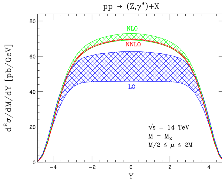
Figure 4.9. LO, NLO, and NNLO predictions and uncertainties for pp to Z boson production, differential in rapidity Y at the LHC, reproduced from Ref. [15].
