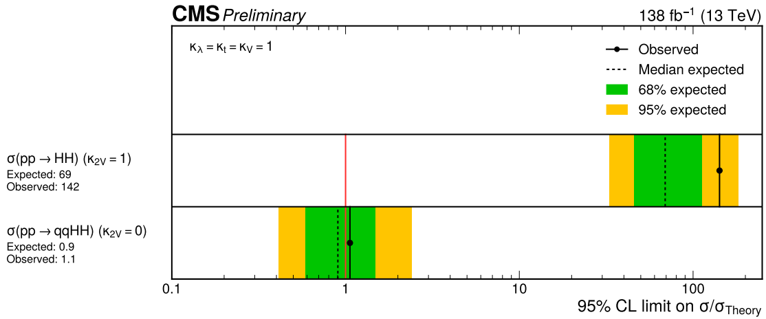
Figure 14.5. Observed and expected exclusion limits at 95% CL for the HH \rightarrow b\bar{b}VV signal SM cross section (top) and cross section at \kappa_{2V} = 0 (bottom).
