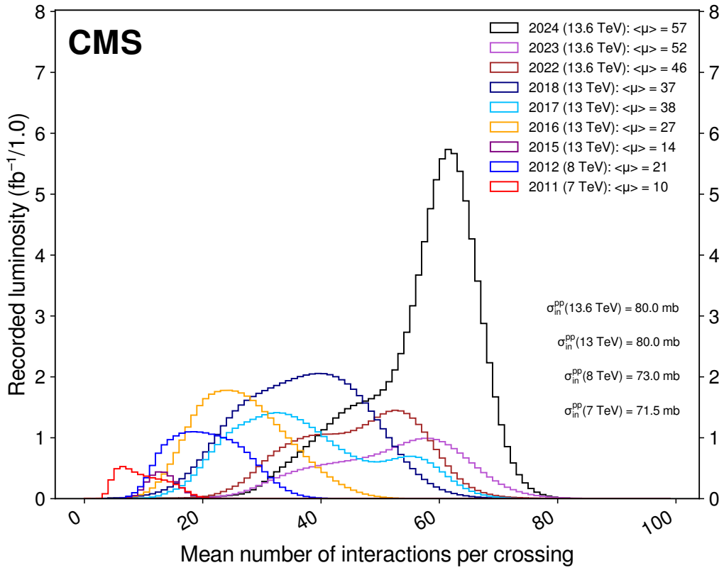
Figure 5.6. Mean number of interactions per crossing (pileup) in CMS between 2011–2024, reproduced from Ref. [36].
