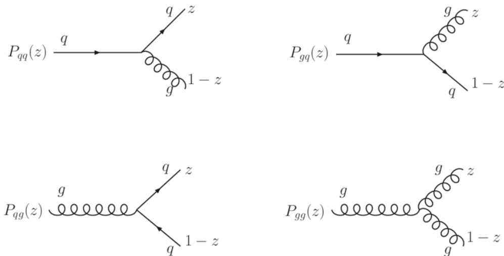
Figure 4.10. The splitting functions for quarks and gluons, reproduced from Ref. [16].
