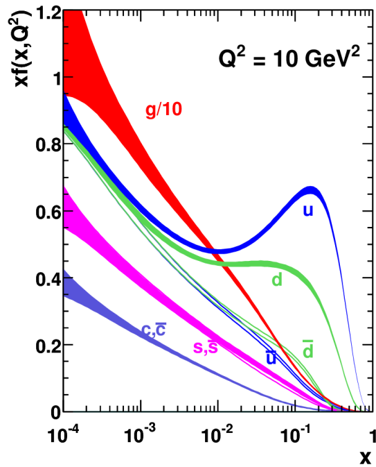
Figure 4.8. PDFs for the proton at Q^2 = 10 \text{ GeV} , reproduced from Ref. [14].
