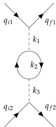
Figure 3.4. An example of a higher-order scattering diagram with a “loop”.
