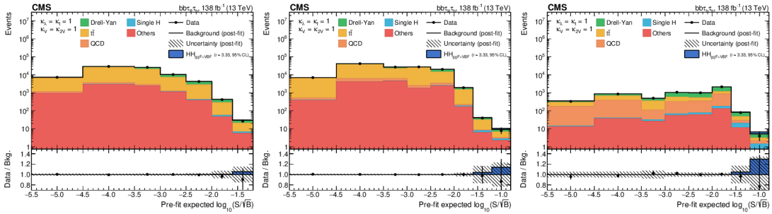
Figure 4.26. Combination of bins of all postfit distributions of the Run 2 CMS HH \rightarrow b\bar{b}\tau\tau analysis [29], ordered according to the expected signal-to-square-root-background ratio, separately for the \tau_h\tau_e (left), the \tau_h\tau_\mu (center), and \tau_h\tau_h (right) channels.
