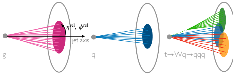
Figure 9.1. The three jet classes we simulate. Gluon (g) and light quark (q) jets have simple topologies, with q jets generally containing fewer particles. Top quark (t) jets have a complex three-pronged structure. Shown also are the relative angular coordinates \eta^{\text{rel}} and \phi^{\text{rel}} , measured from the jet axis.
