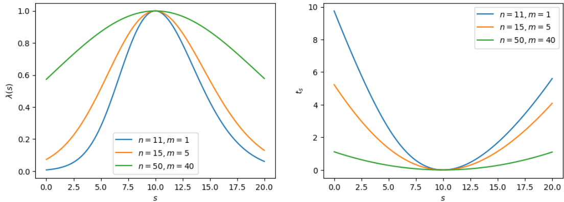
Figure 8.2. The profile likelihood ratio \lambda(s) (left) and the t_s test statistic (right) for our one-bin Poisson model.
