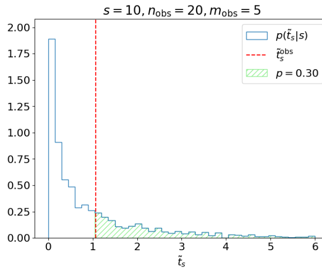
Figure 8.7. Testing H_s in Example 8.2.1.
