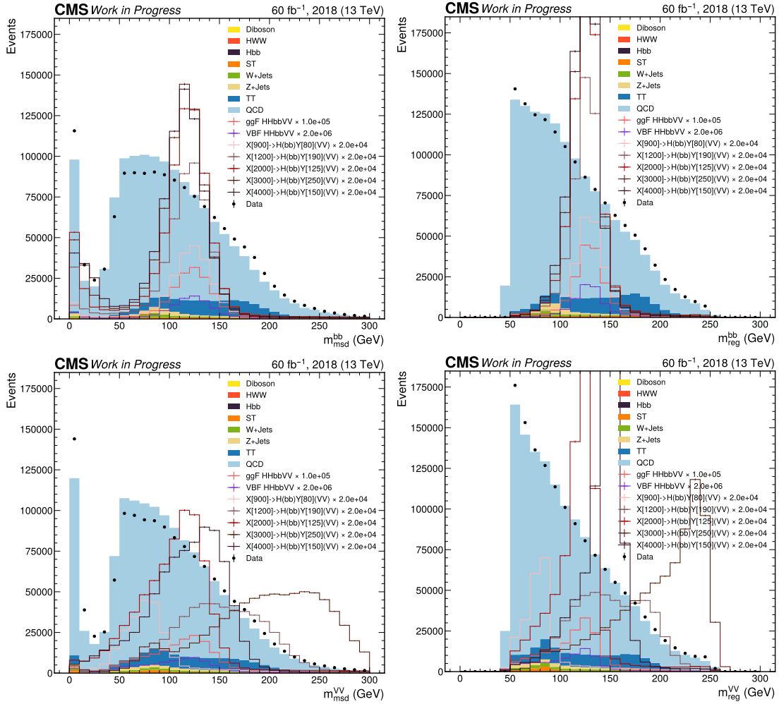
Figure 13.1. Soft drop (left) and regressed (right) mass distributions for the bb and VV -candidate AK8 jets for 2018 data and simulated samples following a loose pre-selection for boosted jets.
