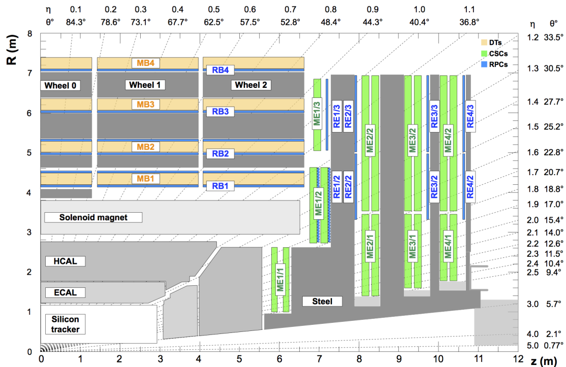
Figure 6.13. Layout of the CMS detector in the r - z plane, with the muon system highlighted and the steel return yoke in dark grey, reproduced from Ref. [47]. The drift tube stations (DTs) are labeled MB (“Muon Barrel”) and the cathode strip chambers (CSCs) are labeled ME (“Muon Endcap”). Resistive plate chambers (RPCs) are mounted in both the barrel and endcaps of CMS, where they are labeled RB and RE, respectively.
