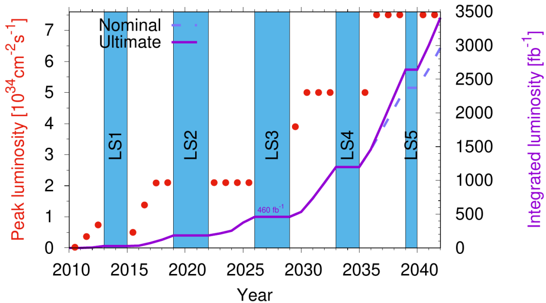
Figure 5.7. Integrated luminosity delivered by the LHC so far and the projection up to 2041, reproduced from Ref. [37].
