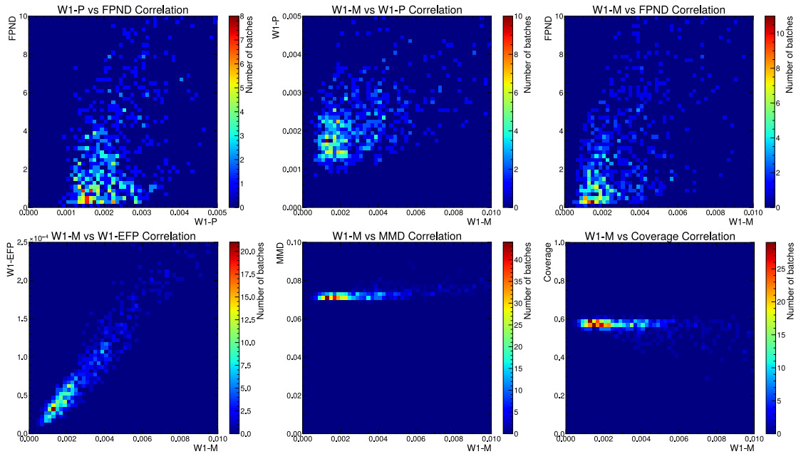
Figure 10.7. Correlation plots between pairs of evaluation metrics, evaluated on 400 separate batches of 50,000 MPGAN generated top quark jets.
