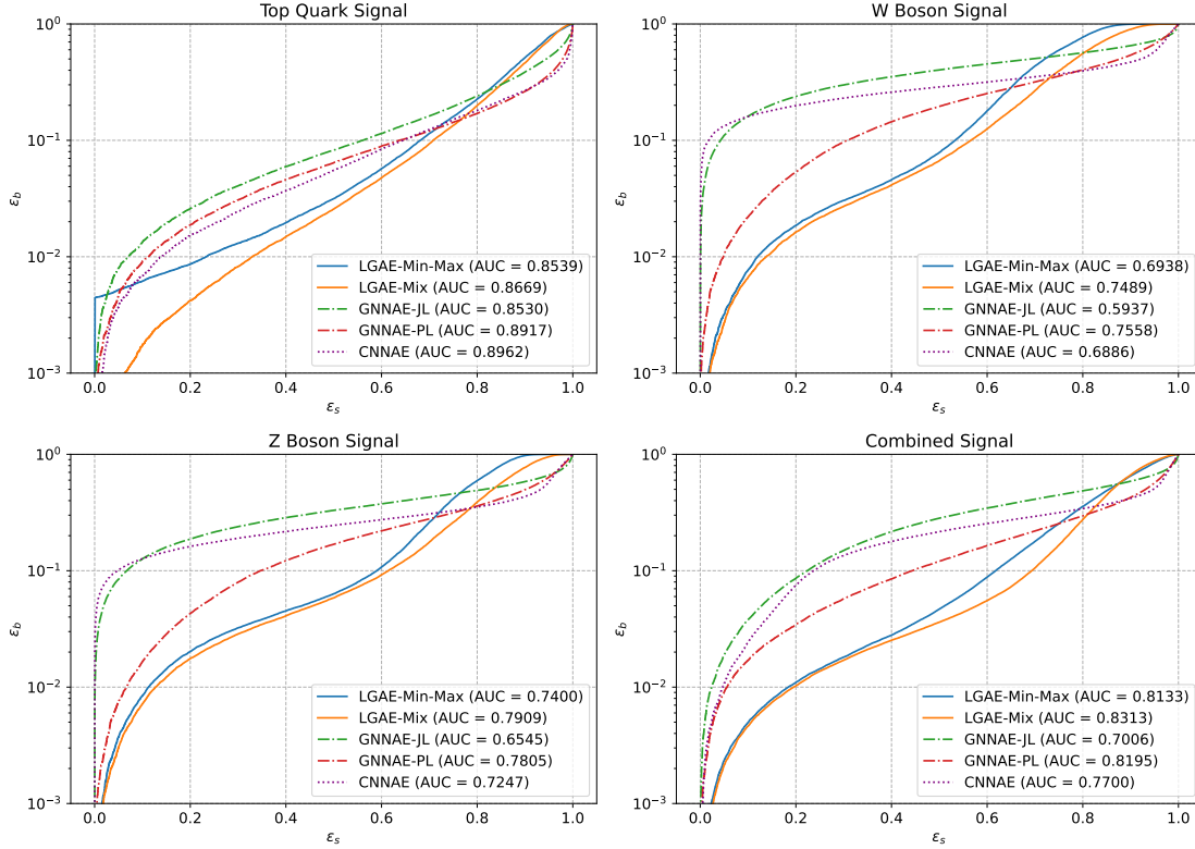
Figure 16.4. Anomaly detection ROC curves for the top quark signal (upper left), W boson signal (upper right), Z boson signal (lower left), and the combined signal (lower right) by the selected LGAE-Min-Max ( \tau_{(1/2,1/2)} = 7 ), LGAE-Mix ( \tau_{(1/2,1/2)} = 2 ), GNNAE-JL ( \dim(L) = 30 ), GNNAE-PL ( \dim(L) = 2 \times 30 ), and CNNAE ( \dim(L) = 55 ) models.
