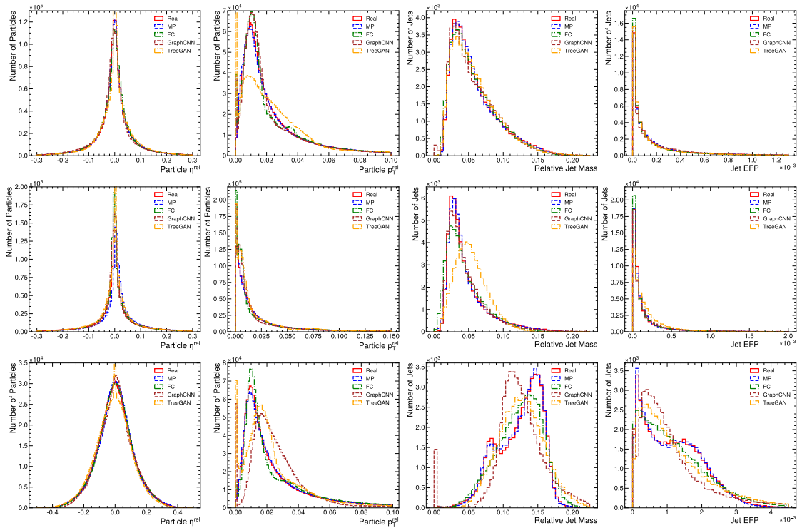
Figure 10.3. Comparison of real and generated distributions for a subset of jet and particle features. We use the best performing model for each of the FC, GraphCNN, TreeGAN, and MP generators, as per Table 10.2. Top: gluon jet features, Middle: light quark jets, Bottom: top quark jets.
