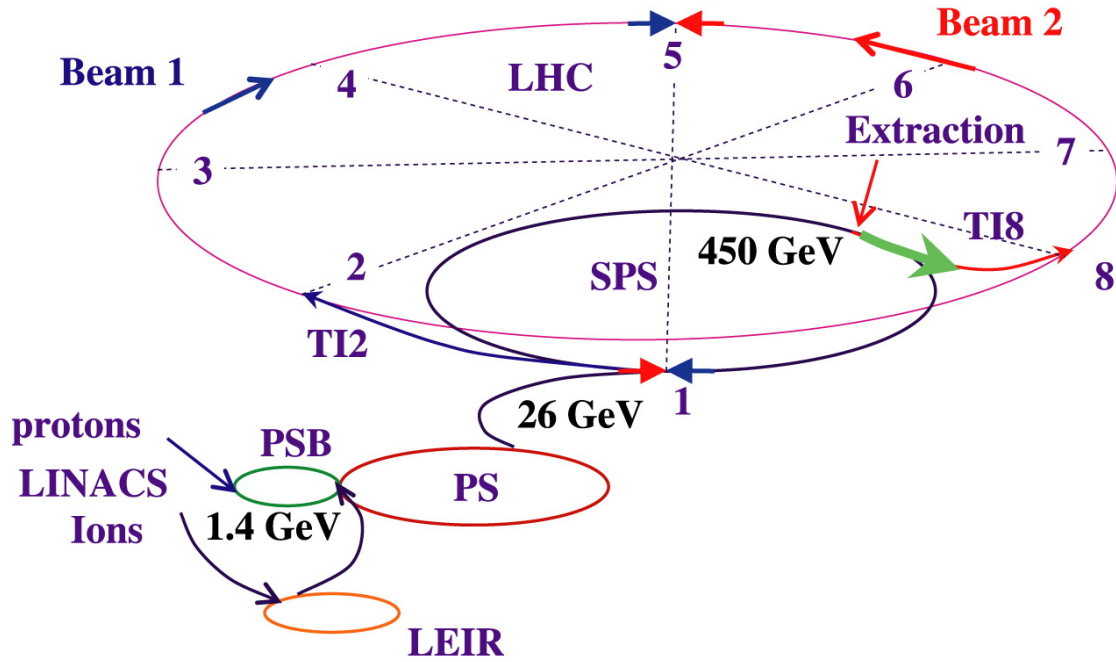
Figure 5.3. Schematic of the LHC injectors, reproduced from Ref. [34].
