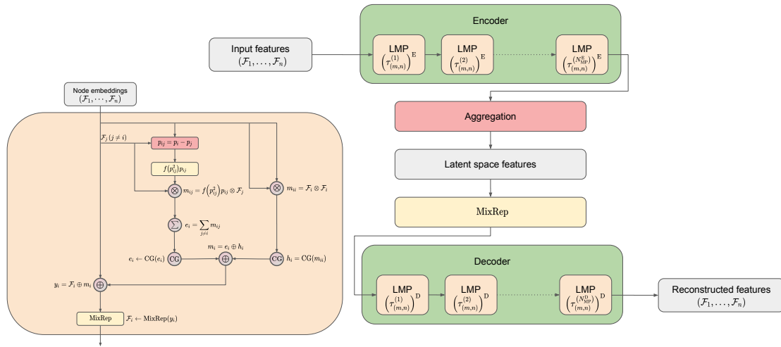
Figure 16.1. Individual Lorentz group equivariant message passing (LMP) layers are shown on the left, and the LGAE architecture is built out of LMPs on the right. Here, MixRep denotes the node-level operator that upsamples features in each (m, n) representation space to \tau_{(m,n)} channels; it appears as W in Eq. (16.2.4).
