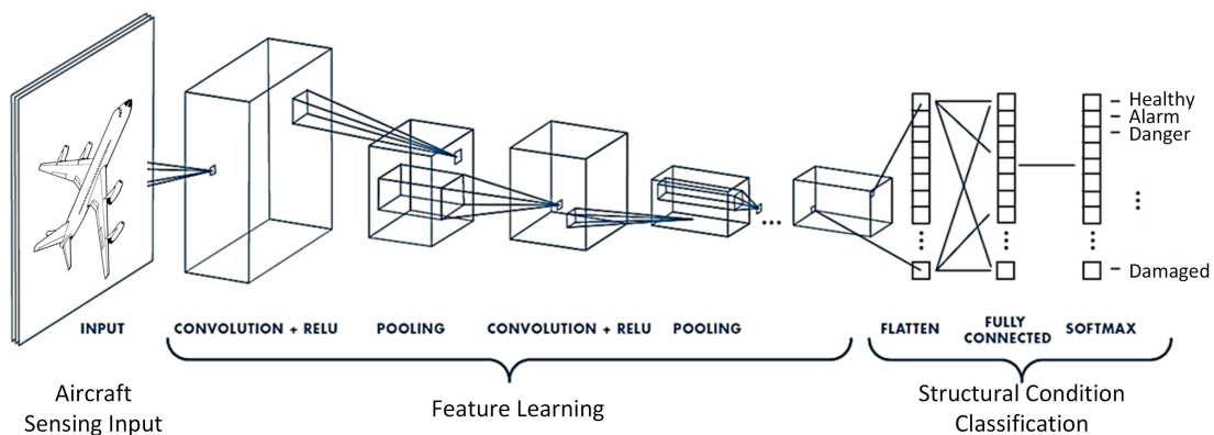
Figure 7.4. Schematic of a convolutional neural network, reproduced from Ref. [51].
