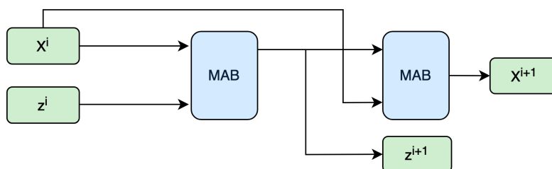
Figure 10.9. Illustration of an induced particle attention block (IPAB).
