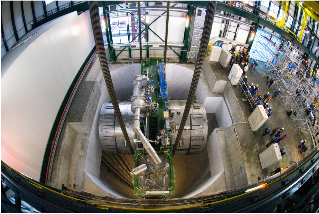
Figure 6.5. The CMS solenoid, as it was being lowered into the CMS cavern in 2007, reproduced from Ref. [41].
