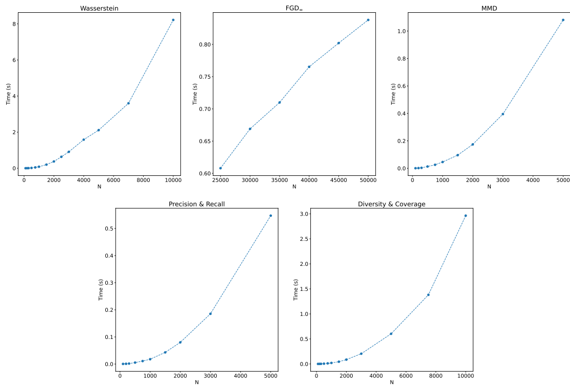
Figure D.2. Time taken per each metric on Gaussian-distributed datasets as described in Section 11.2.
