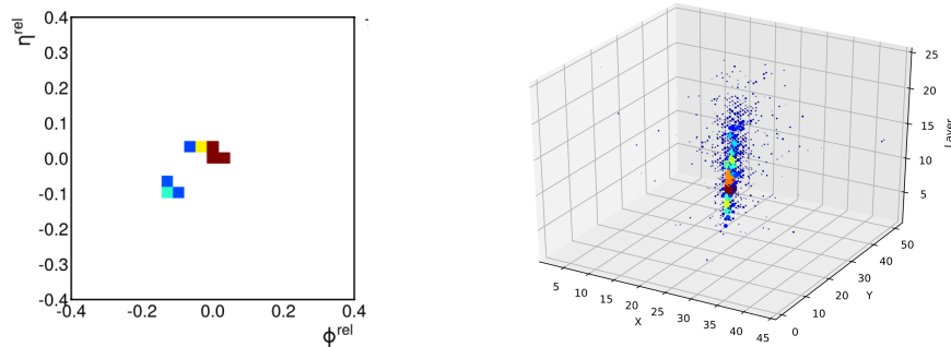
Figure 7.7. Examples of a jet (left) and calorimeter shower (right) represented as 2D and 3D images, respectively.
