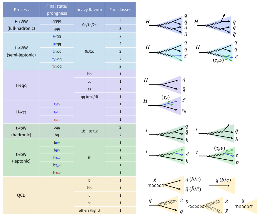
Figure 13.2. Full set of training jet classes for GloParT.
