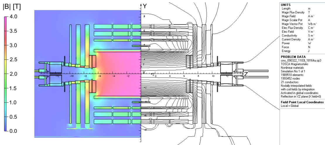
Figure 6.6. Measurement using cosmic rays (left) and illustration (right) of the CMS magnetic field, reproduced from Ref. [42].
