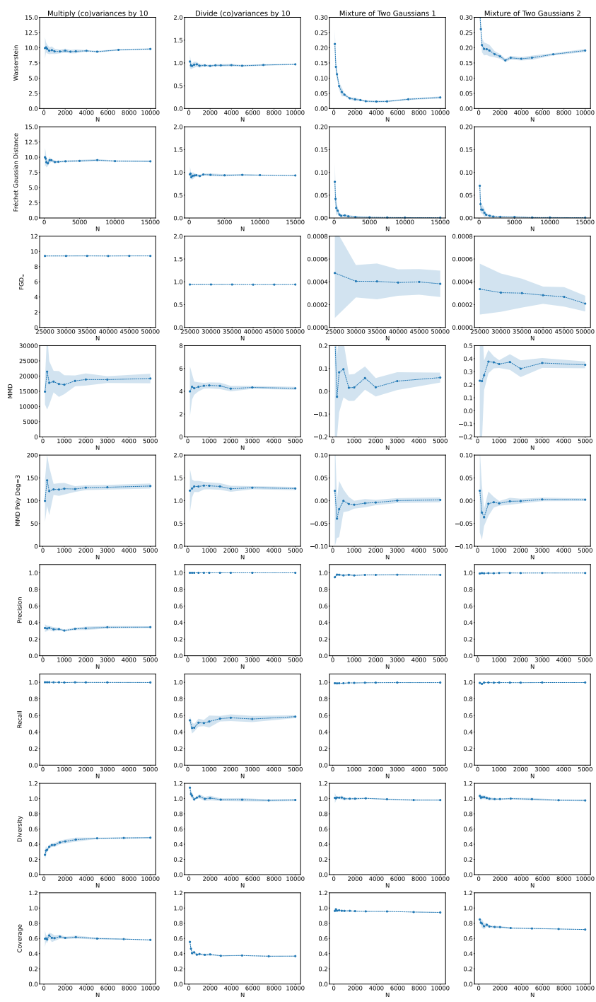
Figure D.4. Scores of each metric on Gaussian-distributed datasets as described in Section 11.2.
