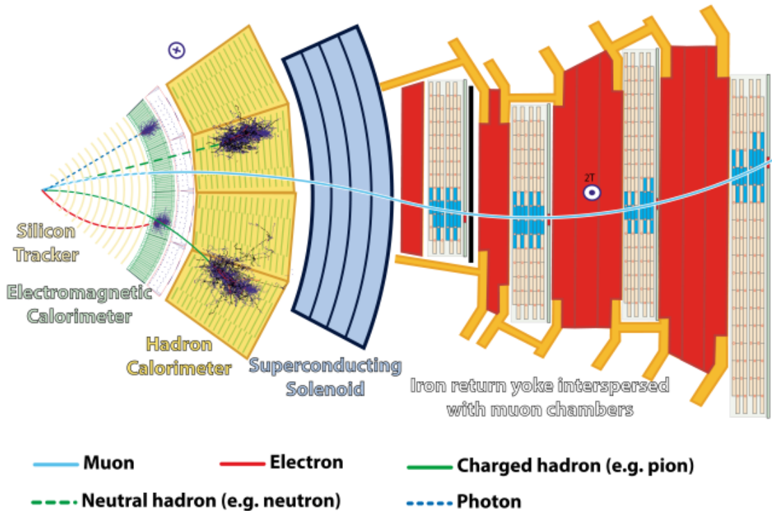
Figure 6.4. Illustration of the different detector layers in the CMS barrel region and the expected hits and energy deposits from various particles, reproduced from Ref. [40].
