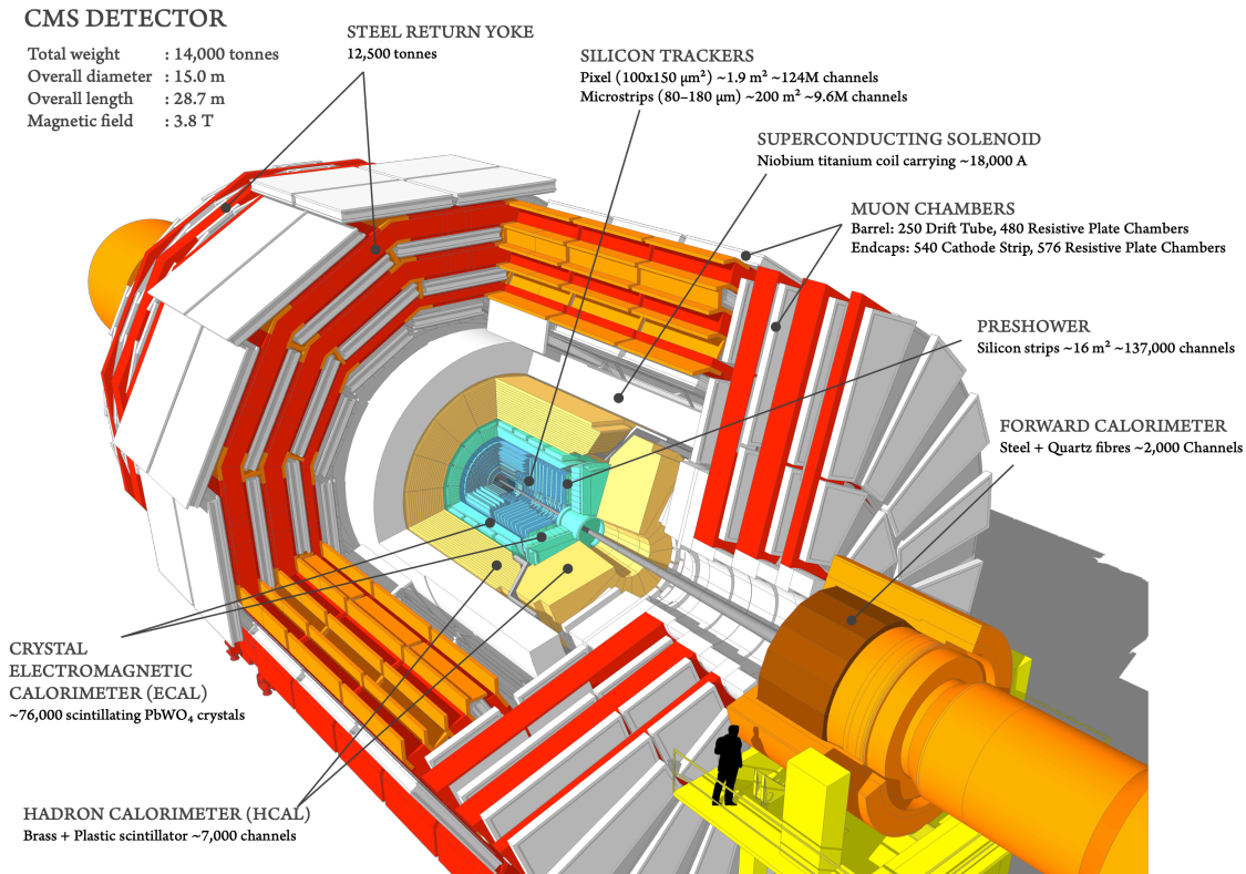
Figure 6.1. A cutaway view of the CMS detector showing the various subdetectors and the solenoid magnet, reproduced from Ref. [39].
