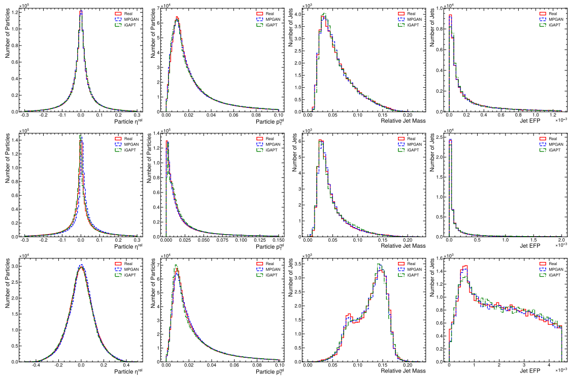
Figure 10.10. Low-level particle feature distributions (far left and center left) and high-level jet feature distributions (center right and far right) for the real data (red), MPGAN-generated data (blue), and iGAPT-generated data (green), for 30-particle gluon (top row), light quark (middle), and top quark jets (bottom). A sample d = 4 energy flow polynomial [322] is plotted in the rightmost column.
