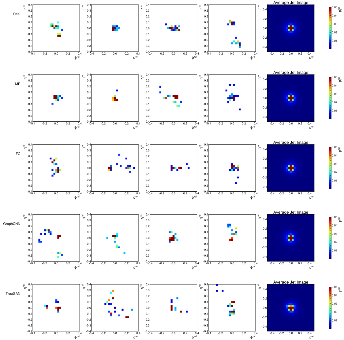
Figure 10.4. Random samples of discretized images in the \eta^{\text{rel}} - \phi^{\text{rel}} plane, with pixel intensities equal to particle p_{\text{T}}^{\text{rel}} , of real and generated gluon jets (left), and an average over 10,000 such sample images (right).
