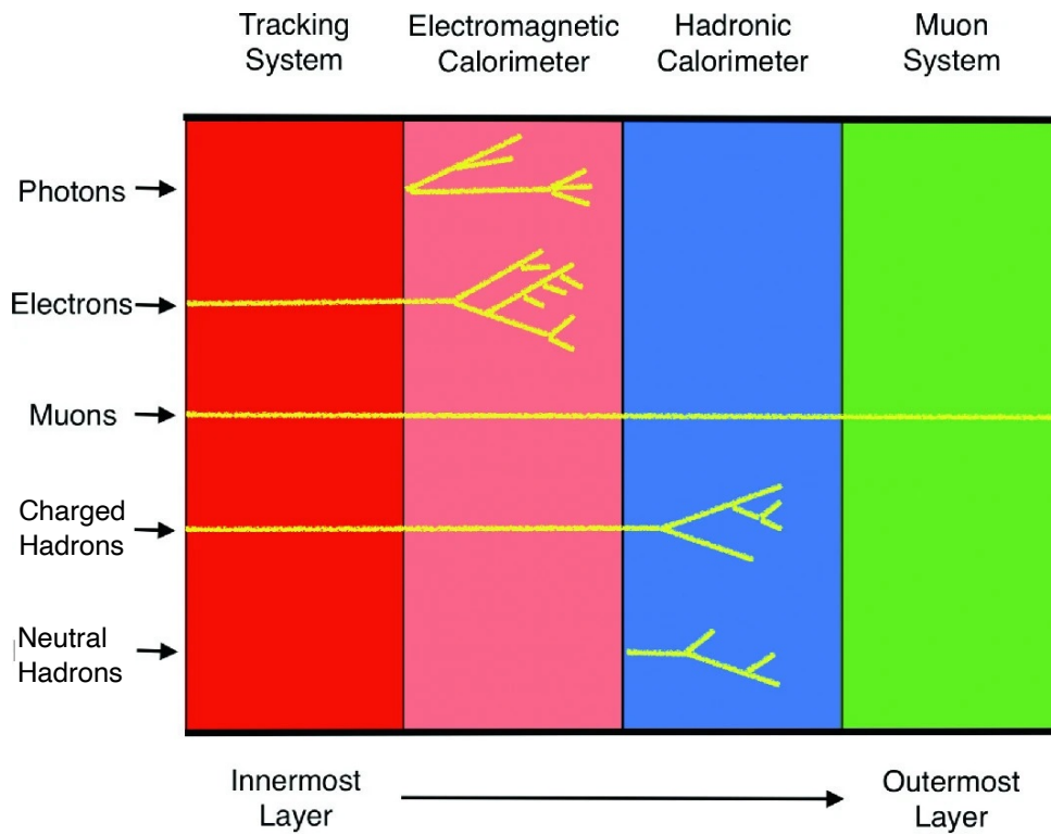
Figure 6.3. Layers in a typical general-purpose detector in particle physics and an illustration of the interactions of different particles.
