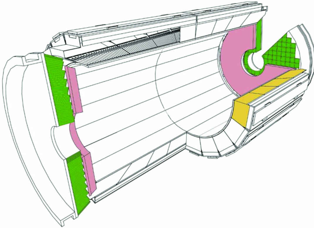
Figure 6.9. Layout of the CMS ECAL, reproduced from Ref. [44], with one of the 36 barrel regions highlighted in yellow, the preshower in pink, and the endcap regions in green.
