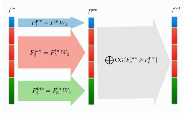
Figure 7.10. Schematic of a Lorentz group-equivariant network layer, reproduced from Ref. [54].
