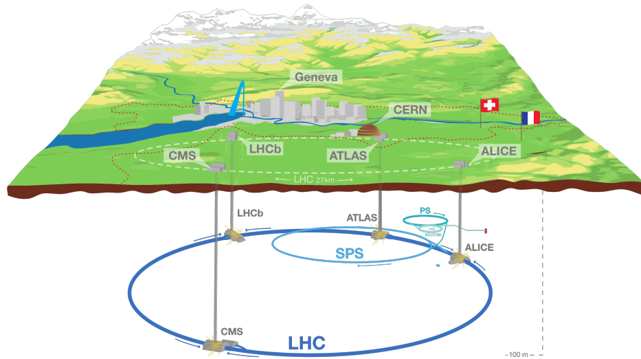
Figure 5.2. Diagram of the LHC accelerator complex adapted from Ref. [33], depicting the initial proton source (in red), LINAC, proton synchrotron booster, PS, SPS, LHC, and the four main experiments: CMS, ATLAS, ALICE, and LHCb.
