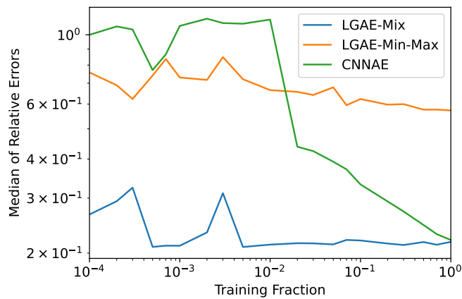
Figure 16.7. Median magnitude of relative errors of jet mass reconstruction by LGAE and CNNAE models at trained on different fractions of the training data.
