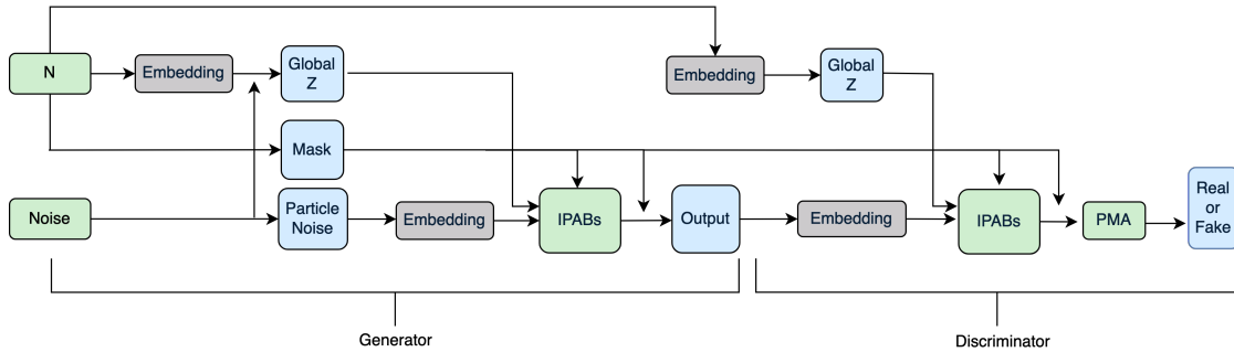
Figure 10.8. Diagram of the iGAPT generator and discriminator networks.
