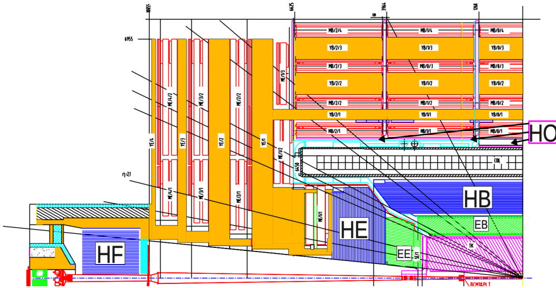
Figure 6.11. Layout of the CMS detector in the r - z plane with the four HCAL sections labeled, reproduced from Ref. [45].
