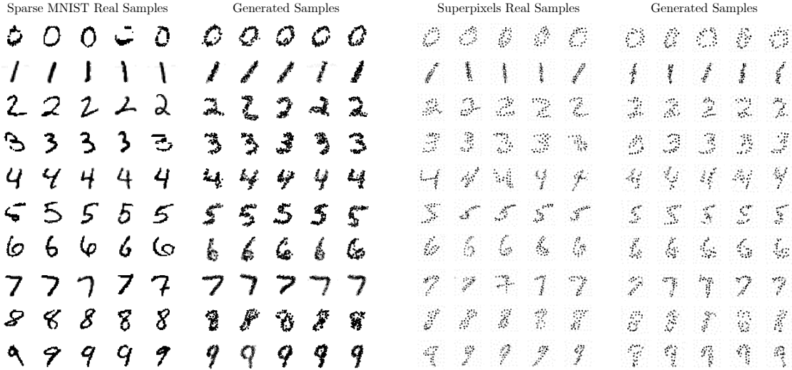
Figure 10.2. Samples from our sparse MNIST dataset (far left) compared to samples from MPGAN (center left). Samples from the MNIST superpixels dataset (center right) compared to samples from MPGAN (far right).
