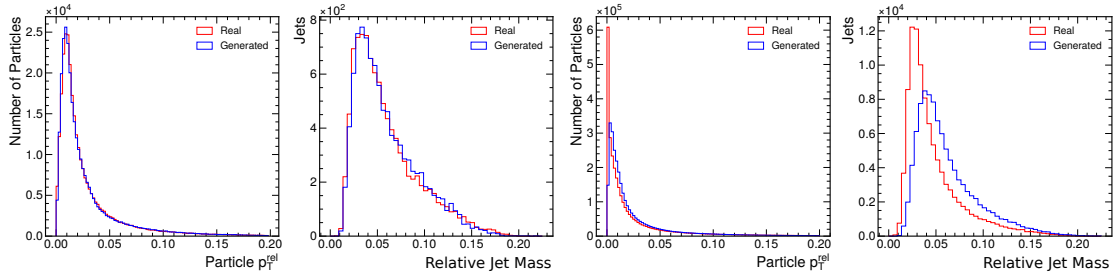
Figure C.2. Particle p_T^{\text{rel}} and relative jet mass distributions of real jets and those generated by MPGAN without our masking strategy. Left: gluon, right: light quark jets. We see that while for gluon jets the generator learns distributions correctly, it struggles to learn the discontinuous spike, due to the zero-padded particles, in the light quark p_T^{\text{rel}} distribution. This also leads to a distorted mass distribution.
