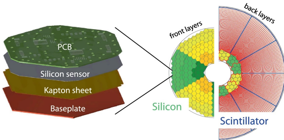
Figure 6.16. (Left) layers of the individual HGAL modules and (right) their layout in the all-silicon and mixed layers, reproduced from Ref. [49].
