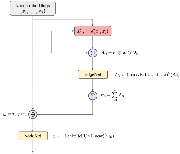
Figure E.1. An MPNN layer in the GNNAE. Here, EdgeNet and NodeNet are feed-forward neural networks.
