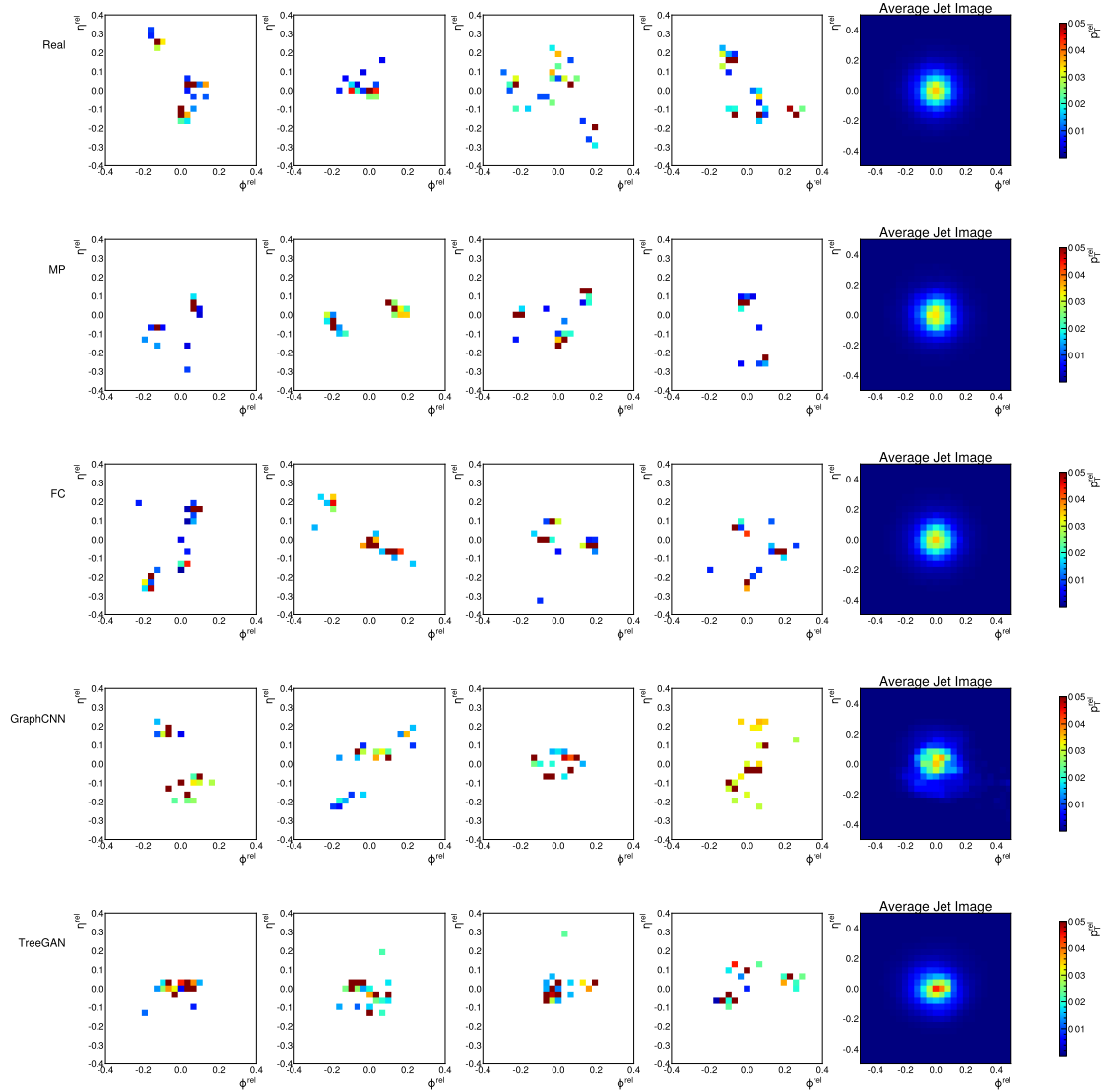
Figure 10.6. Random samples of discretized images in the \eta^{\text{rel}} - \phi^{\text{rel}} plane, with pixel intensities equal to particle p_{\text{T}}^{\text{rel}} , of real and generated top quark jets (left), and an average over 10,000 such sample images (right).
