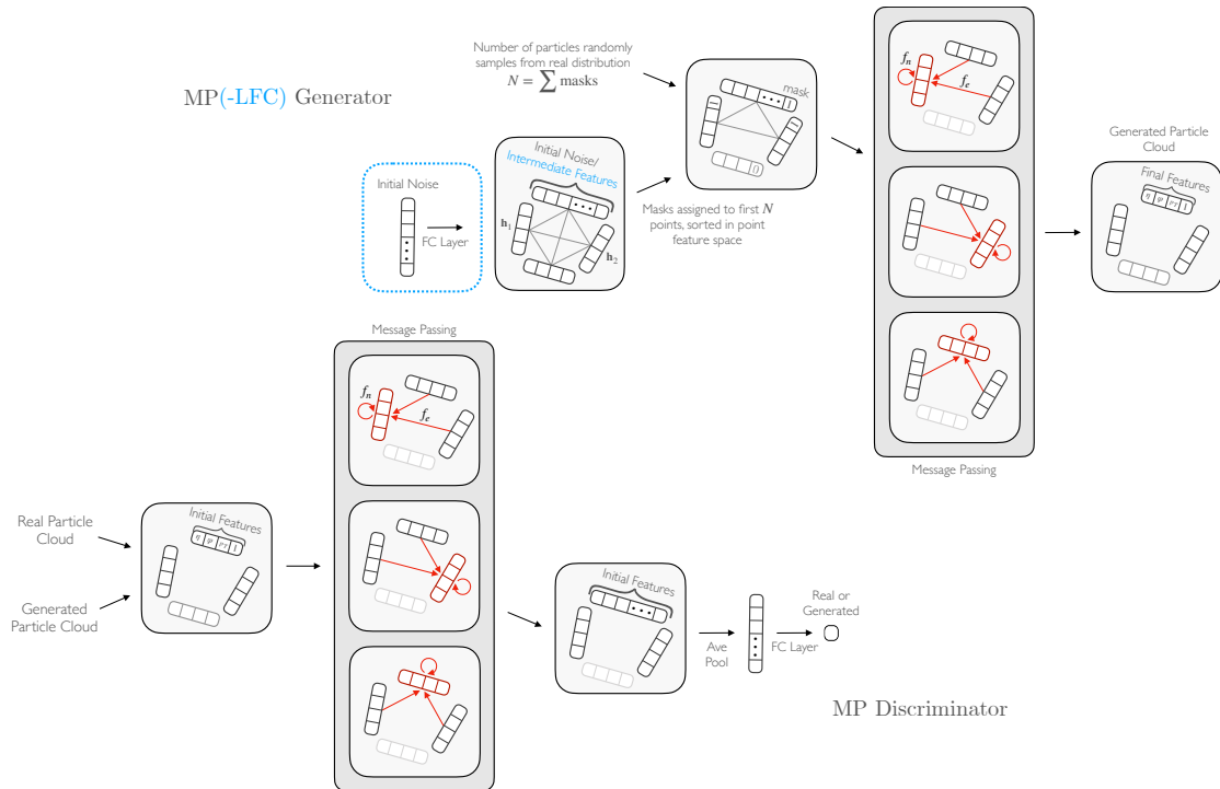
Figure 10.1. Top: The MP generator uses message passing to generate a particle cloud. In blue is the initial latent vector and FC layer part of the MP-LFC variant. Bottom: The MP discriminator uses message passing to classify an input particle cloud as real or generated.
