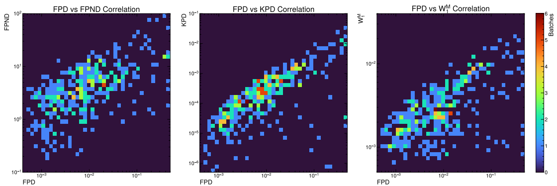
Figure 11.4. Correlations between FPD and FPND, KPD, and W_1^M on 400 separate batches of 50,000 GAPT-generated jets.
