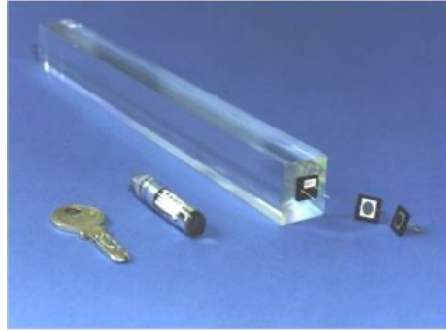
Figure 6.10. \text{PbWO}_4 crystals and photodiodes used in the CMS ECAL.
