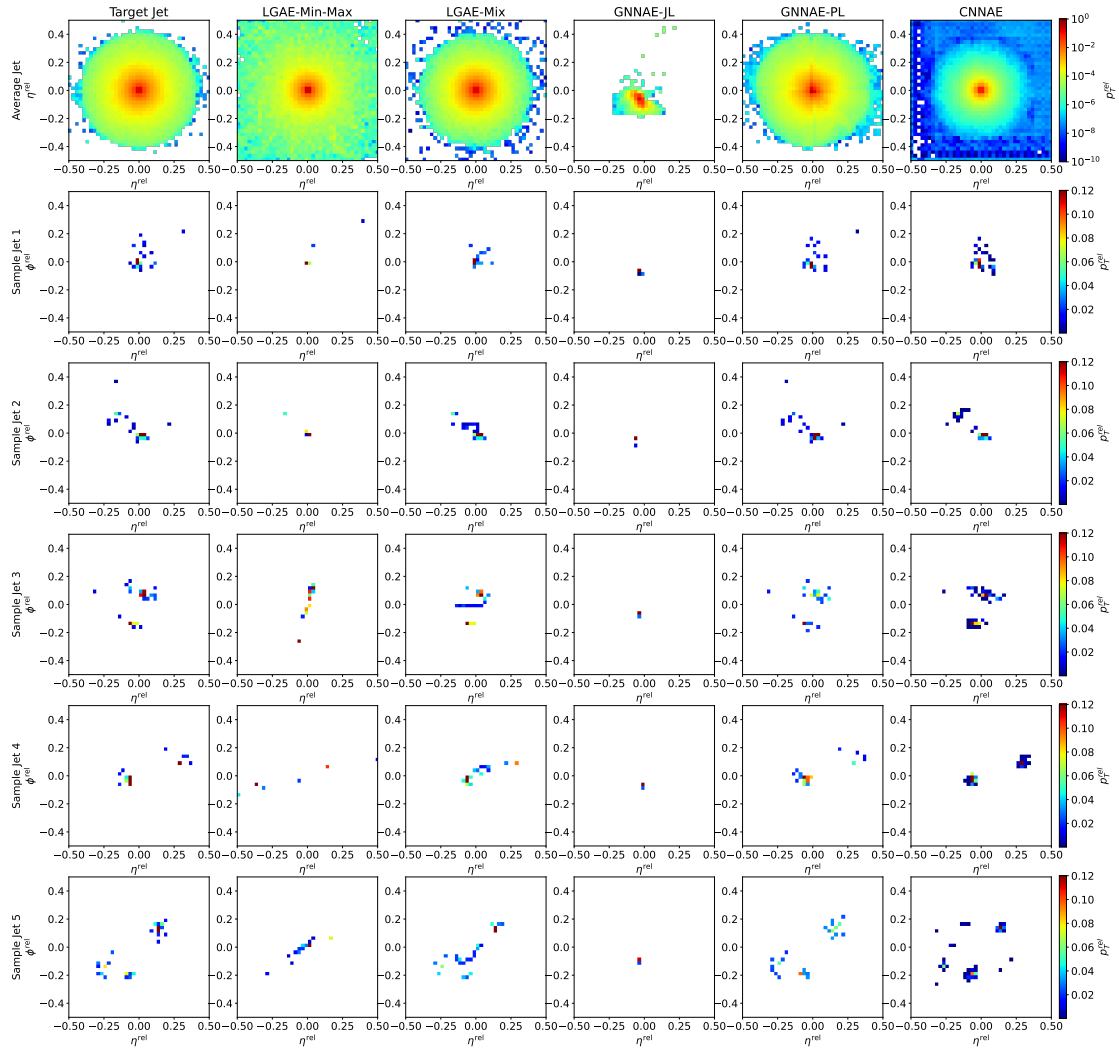
Figure 16.2. Jet image reconstructions by LGAE-Min-Max ( \tau_{(1/2,1/2)} = 4 , 56.67% compression), LGAE-Mix ( \tau_{(1/2,1/2)} = 9 , 61.67% compression), GNNAE-JL ( \dim(L) = 55 , 61.11% compression), GNNAE-PL ( \dim(L) = 2 \times 30 , 66.67% compression), and CNNAE ( \dim(L) = 55 , 61.11% compression).
