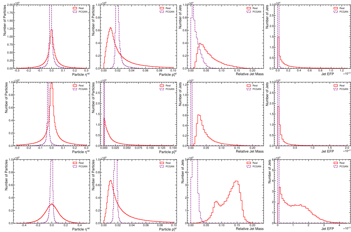
Figure C.1. Comparison of real and PCGAN-generated distributions for a subset of jet and particle features. Top: gluon jet features, Middle: light quark jets, Bottom: top quark jets.
