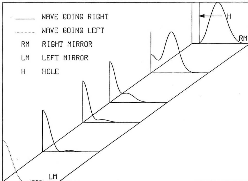
Figure 7. Intensity profile of the dominant azimuthally symmetric mode for an empty confocal resonator with 16 mm mirror radius.
