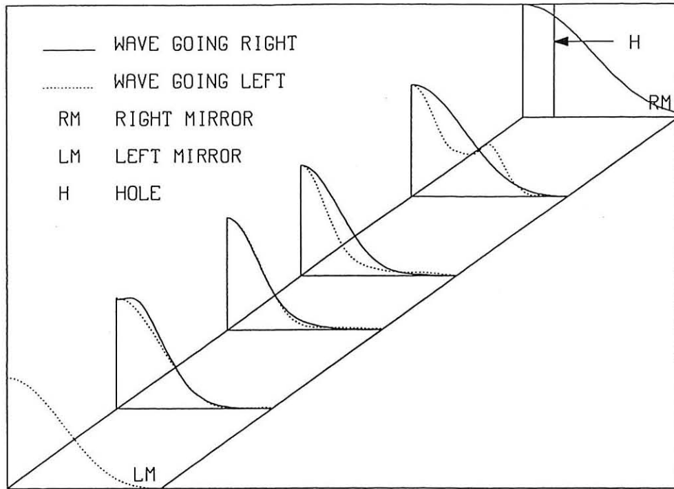
Figure 8. Same as for Fig.(7), except the mirror radii are reduced to 10 mm.
