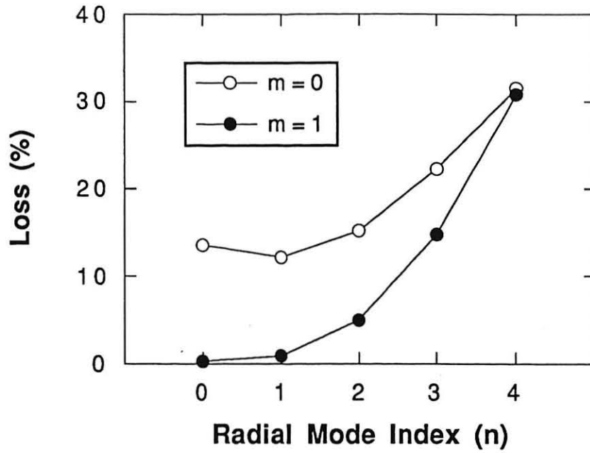
Figure 2. Total losses of five radial modes for m=0 and m=1 in an empty cavity.
