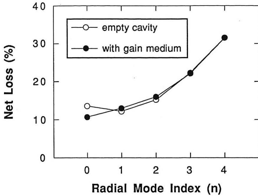
Figure 4. Net losses of five radial modes for m=0 in a cavity with and without FEL gain.
