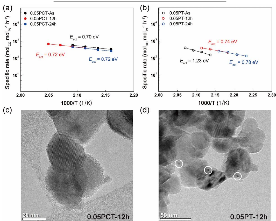
Fig. 4 Long-term CO oxidation test results. The E_{act} of (a) 0.05PCT and (b) 0.05PT catalysts measured before and after the long-term high temperature reaction tests (1 vol.% CO + 4 vol.% O 2 + 95 vol.% Ar at 300 °C). STEM images of (c) 0.05PCT and (d) 0.05PT catalysts after 12 hours of CO oxidation. White circles in (d) represent Pt NPs (diameter ≈ 3 nm). Refer to Fig. S7 in the ESI† and discussion therein for detailed experimental procedure and additional STEM images.
