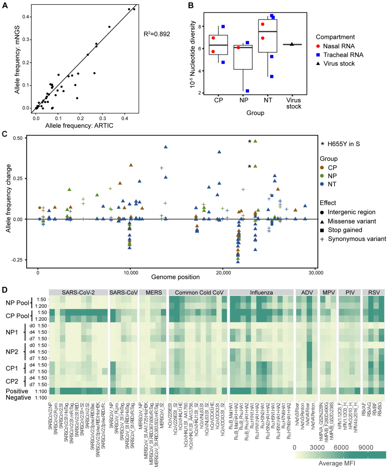
FIG 4 Impact of CP treatment on viral replication and evolution. (A) Comparison of allele frequencies determined using amplicon (ARTIC) and metagenomic sequencing (mNGS) methods. The square of the Pearson correlation coefficient values are shown. (B) Impact of treatment on viral sequence nucleotide diversity in nasal lavages and tracheal aspirates was assessed by ARTIC for comparison with the virus stock used for inoculation. A box plot of pairwise nucleotide diversity shows the median and the 1st and 3rd quartiles. (C) Impact of treatment on viral allele frequencies was assessed in comparison to the virus stock. Asterisks indicate expansion of a H655Y substitution in the viral spike protein. (D) Heat map showing antibody cross-reactivity to other related viruses in the human plasma pools and in plasma samples from study animals treated with NP and CP.
