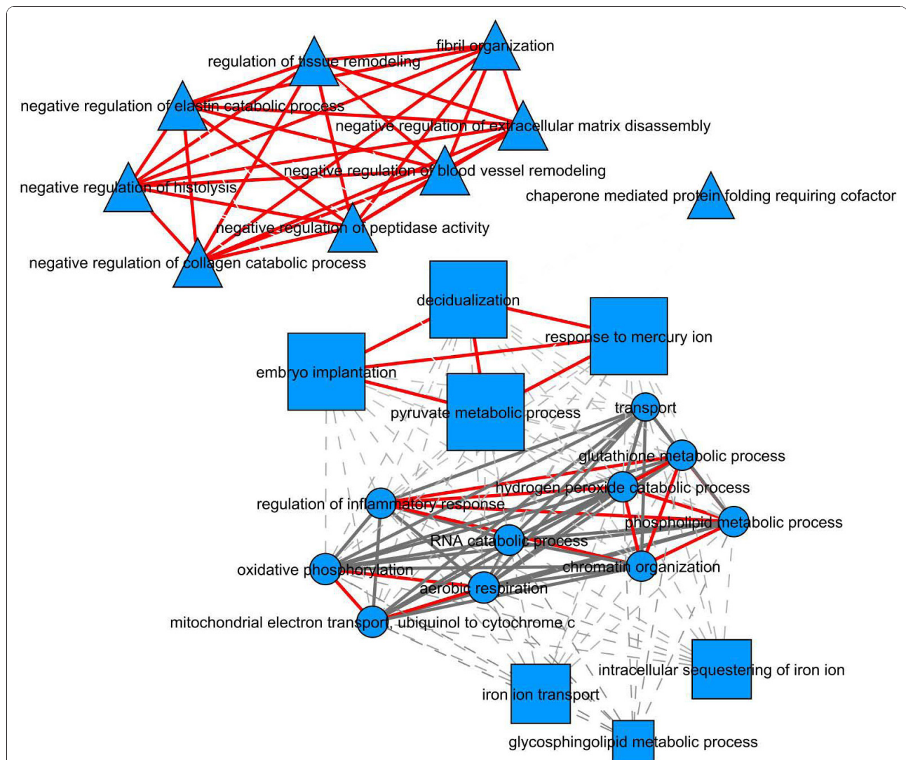
Figure 2 Functional and network analysis of the most highly-expressed genes. Analysis of the genes displaying expression levels above 13 clustered in particular functional networks. Different shapes represent different modules of biological functions. Dashed lines are relationships between nodes in different modules and solid lines are relationships between nodes in the same module. Dashed lines depict medium strong interactions (i.e. in between the median of the distribution and its upper quartile) and solid lines indicate the strongest interactions (i.e. superior to the upper quartile of their distribution). The interactional centrality of GO themes is illustrated by the size of the corresponding nodes. A red line denotes that the same gene is linked between all the biological process and gray lines denote different genes in each node.
