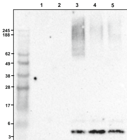
Fig. 5 A \beta peptides are oligomerized during incubation with cells and reduced by co-incubation with Hsp70. Cells (N2A) were incubated in DMEM medium containing 1% FBS at 37 ^{\circ} C for 48 h in the absence (lane 1) or presence of Hsp70 (0.32 \mu g) (lane 2). Cells were also incubated with monomerized A \beta_{1-42} peptides (10 \mu M) (lane 3) or co-incubated with Hsp70 (0.32 \mu g) added on day 1 or added on days 1 (lane 4) and 2 (lane 5). At the end of the incubation period, the extracellular medium was collected, depleted of any floating cells by centrifugation and electrophoresed, transferred onto nitrocellulose membranes, and analyzed by Western blotting using Clone 4G8 antibody followed by an HRP-conjugated secondary antibody
