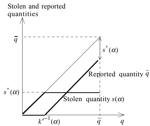
Figure 2. Optimal stealing as a function of output realization for given \alpha
