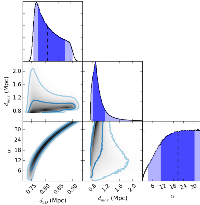
Figure B3. One-dimensional marginalized PDFs (panels on the diagonal) and two-dimensional marginalized PDFs of variables denoting characteristic distances and projection angle of the mergers.
