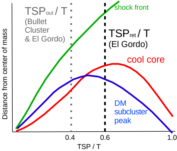
Figure 9. Schematic evolution of cool core gas and DM displacements relative to the merger center of mass as a function of the phase ( TSP/T ), based on simulations of a bimodal cluster merger by Mathis et al. (2005) . During and shortly after core passage, ram pressure ( =\rho v^2 ) exerts substantial force on the cool core, which then lags the DM. (This corresponds to the outgoing scenario of TSP_{out}/T indicated by the grey dotted line). Ram pressure then declines dramatically as the cool core enters regions of lower density. The cool core can then fall into (and past the center of) the gravitational potential of the corresponding DM subcluster as what is described as the slingshot effect ( Markevitch & Vikhlinin 2007 ). The Bullet Cluster is seen at a phase of TSP_{out}/T \approx 0.4 Gyr/ 1.6 Gyr after core passage according to (D13) and indeed the cool core is closest to the center of mass. We found that El Gordo is more likely to be seen at a later stage (as indicated by TSP_{ret}/T rather than TSP_{out}/T ), explaining why the DM of El Gordo is closer to the center of mass than the cool core.
