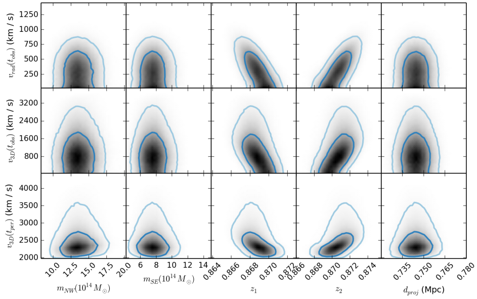
Figure B11. Marginalized PDFs of relative velocities characteristic timescales of the simulation and the inputs.
