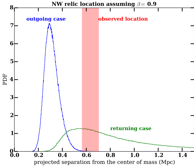
Figure 7. Comparison of the PDFs of the observed position of the NW relic (red bar includes the 95% confidence interval of location of the NW radio relic in the center of mass frame) with the predicted position from the two simulated merger scenarios (blue for outgoing and green for the returning scenario). We made use of the polarization weight for producing this figure. The rationale of picking \beta = 0.9 can be found in the last paragraph of section 3.4.
