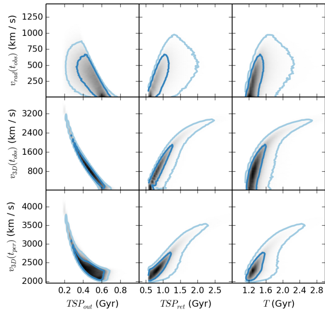
Figure B9. Marginalized PDFs velocities and the characteristic timescales of the simulation against the inputs.
