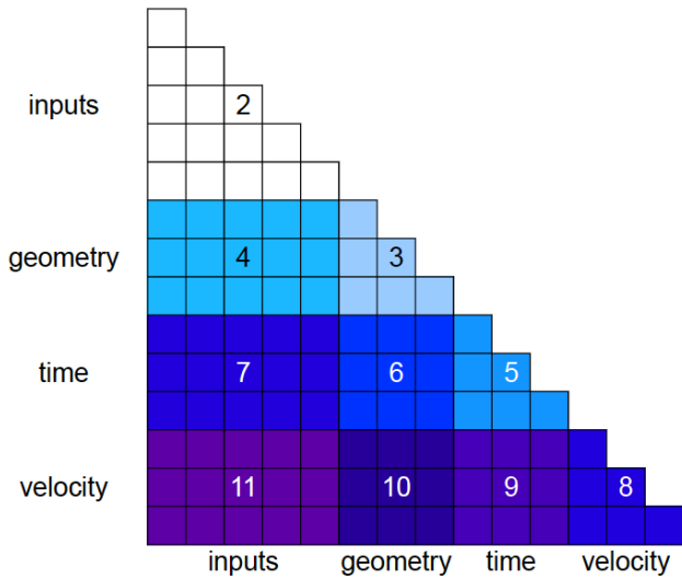
Figure B1. Matrix of variables used in the simulations. We present them in 4 categories, including, inputs, geometry, time and velocity. Regions of the same color represent one plot and the number indicates the corresponding figure number in this appendix.
