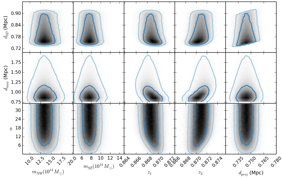
Figure B4. Marginalized PDFs of characteristic distances and projection angle of the merger and the inputs of the simulation.
