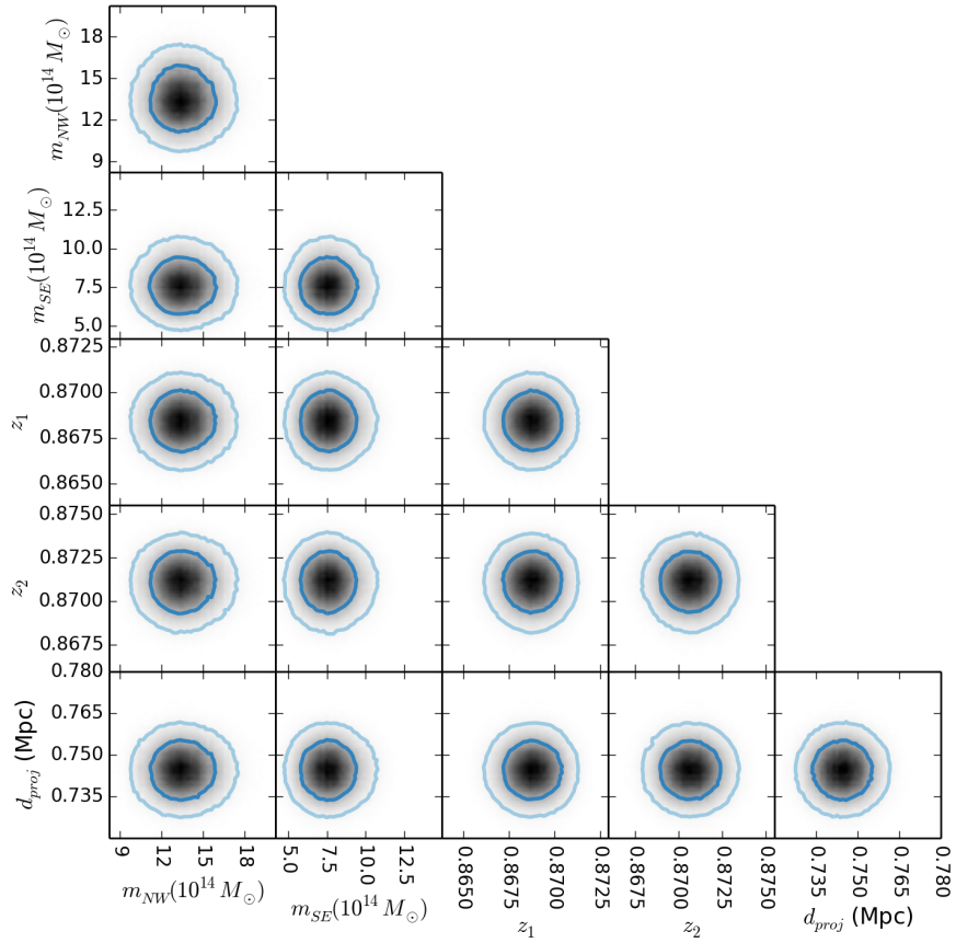
Figure B2. Marginalized 2-dimensional PDFs of original inputs (vertical axis) and the inputs after applying polarization weight and default weights (horizontal axis). The inner and outer contour denote the central 68% and 95% confidence regions respectively. The circular contours show that the application of weights did not introduce uneven sampling of inputs.
