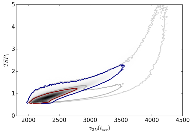
Figure 6. The marginalized output PDF of the returning time-since-pericenter ( TSP_{\text{ret}} ) vs. the 3D velocity at the time of pericenter for El Gordo. The grey set of contours show the confidence regions before applying the polarization weight and the colored contours correspond to the confidence regions after applying the weights. The contours represent the 95% and 68% confidence regions respectively.
