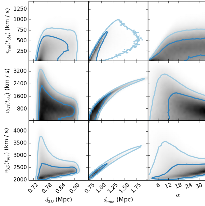
Figure B10. Marginalized PDFs of the velocities at characteristic timescales and the characteristic distances and the projection angle of the merger.
