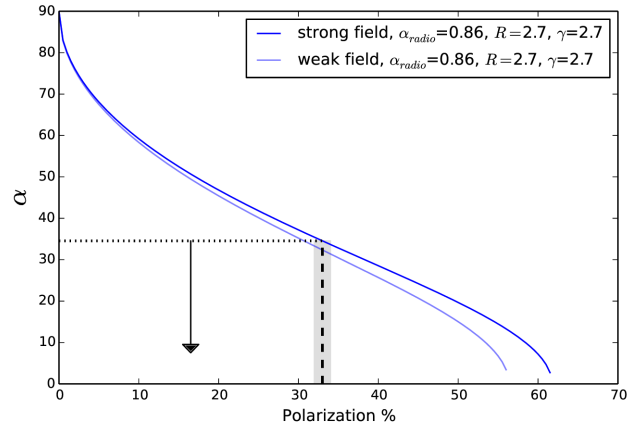
Figure 5. Predictions of polarization percentage of the radio relic at a given projection angle from different models, reproduced from ( Ensslin et al. 1998 ) or equation 5. Each model assumes electrons producing the radio emission to be accelerated inside uniform magnetic field of various strengths ( strong or weak ). The curves are plotted with spectral index of the radio emission ( \alpha_{\text{radio}} ), spectral index of the electrons ( \gamma ) and compression ratio of the magnetic field ( R ) corresponding to the estimated values from Lindner et al. (2014) . We highlight the observed polarization percentage of the main NW radio relic of El Gordo by the dotted vertical line with the greyed out region indicating the uncertainty ( Lindner et al. 2014 ).
