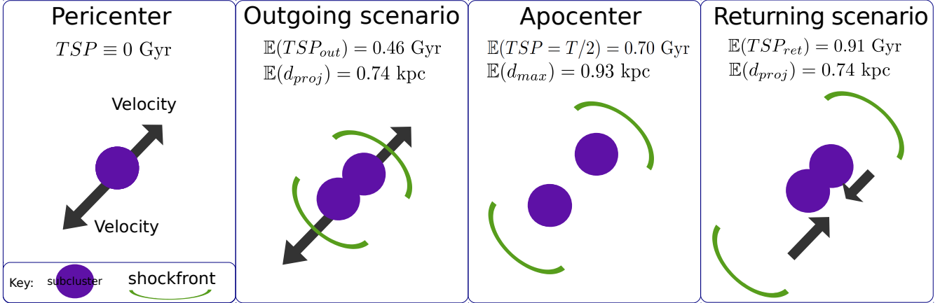
Figure 2. Illustration of the spatial location of different components of El Gordo at different stages of the merger. Earlier stages (with a smaller TSP) are on the left side of later stages. The rightmost returning scenario is preferred from our simulation.
