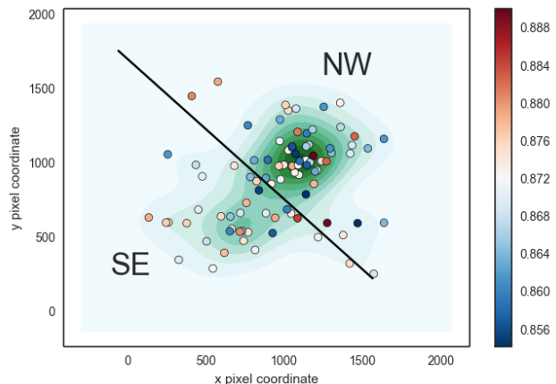
Figure 3. Points showing the locations of the member galaxies and the division of the member galaxies among the two subclusters of El Gordo by a spatial cut (black line). The color of the points shows the corresponding spectroscopic redshift of the member galaxies (see color bar for matching of spectroscopic values), with the redder end indicating higher redshift. The galaxy number density contours in the background in green indicate a bimodal distribution.
