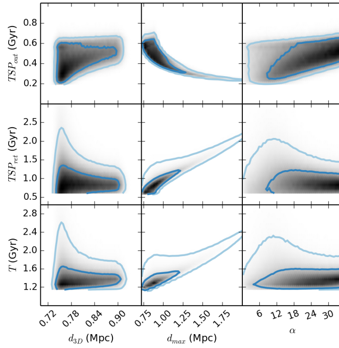
Figure B6. Marginalized PDFs of characteristic timescales of the simulation and the characteristic distances and the projection angle of the merger.
