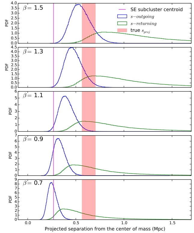
Figure C3. Comparison of the PDFs of the observed position of the NW relic (red bar includes 95% confidence interval of location of relic in the center of mass frame) with the predicted position from the two simulated merger scenarios (blue for outgoing and green for the returning scenario). For the plausible values of \beta < 1.1 , the returning model is preferred. For comparison purpose, we also show that \beta > 1.3 (top panel) for the outgoing scenario to be favored. Note that we made use of the polarization weight for producing this figure.
