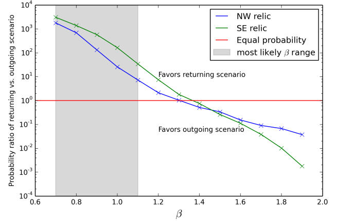
Figure C1. Probability ratio between the returning model (numerator) and the outgoing model at given \beta . We remind readers \beta is a factor relating the time-averaged shock velocity and the centric velocity of the corresponding subcluster.
