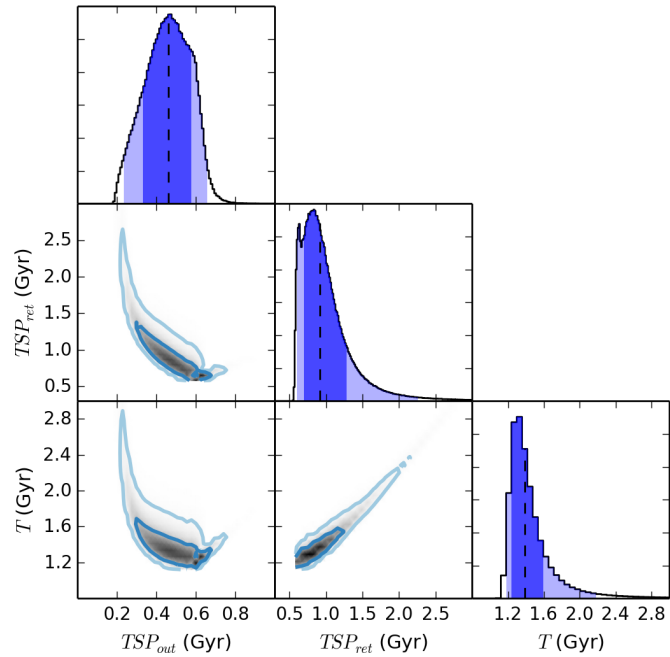
Figure B5. One-dimensional PDFs of characteristic timescales of the simulation (panels on the diagonal) and the marginalized PDFs of different timescales. Note that there is a default weight for constraining TSP_{out} but not for TSP_{ret} and T , so TSP_{out} spans a smaller range.
