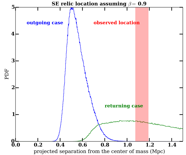
Figure 8. Comparison of the PDFs of the observed position of the SE relic (red bar includes the 95% confidence interval of location of the radio relic in the center of mass frame). We made use of the polarization weight for producing this figure. The rationale of picking \beta = 0.9 can be found in the last paragraph of section 3.4.
