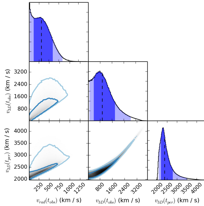
Figure B8. One-dimensional marginalized PDFs of velocities at characteristic times (panels on the diagonal) and marginalized PDFs of different velocities.
