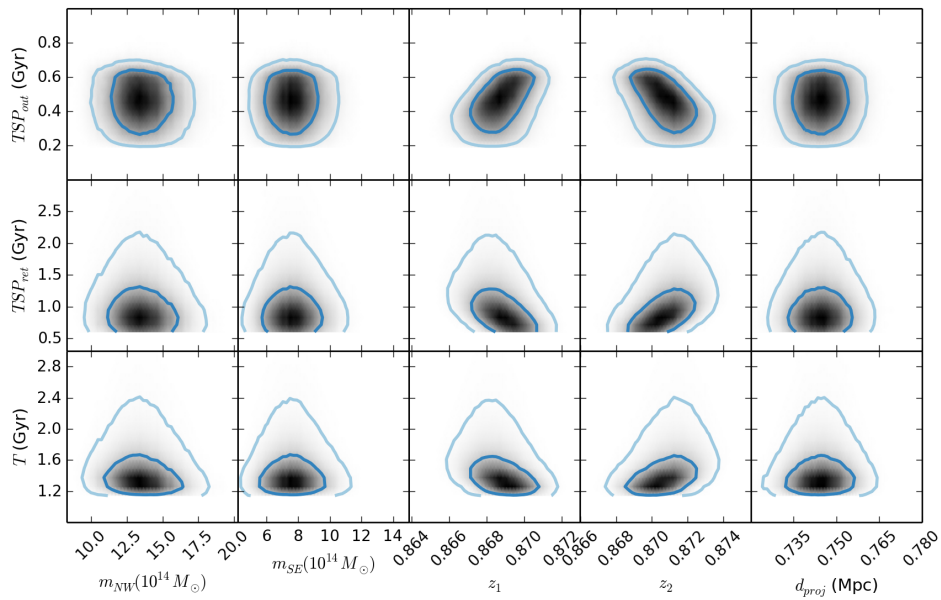
Figure B7. Marginalized PDFs of characteristic timescales of the simulation and the inputs.
