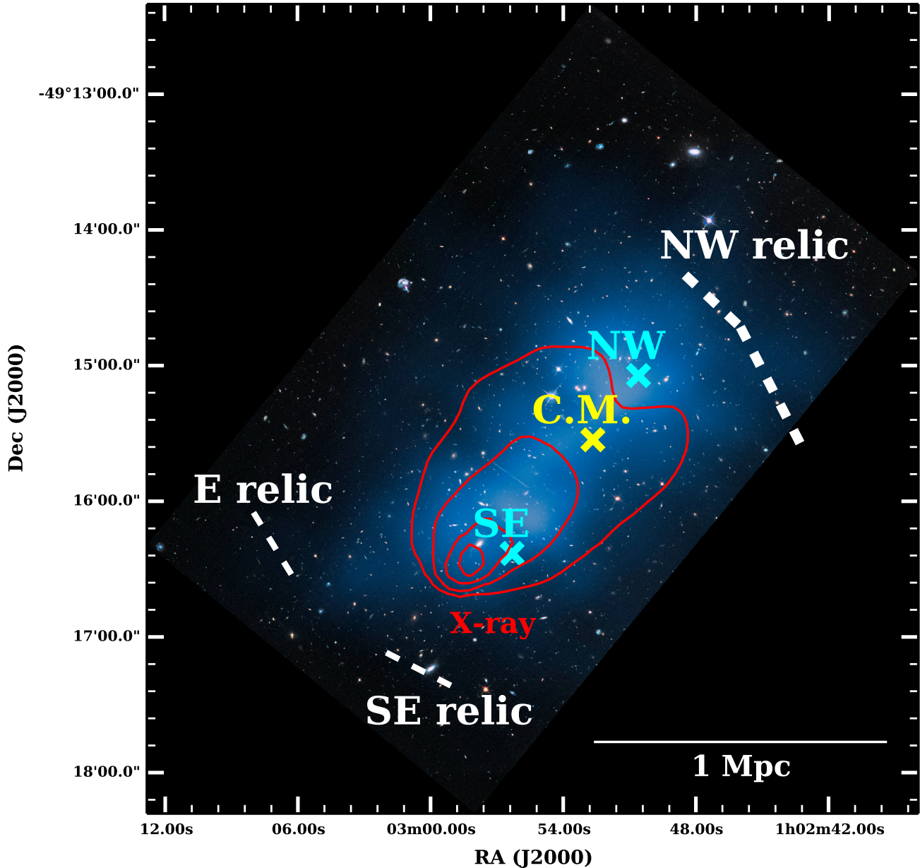
Figure 1. Configuration of El Gordo showing overlay of dark matter distribution in blue, and X-ray emission in red. (Image credit: NASA, ESA and Jee et al. 2014 ). The cross markers show the positions of the northwest (NW) and southeast (SE) dark matter density peaks, and the center of mass (CM) locations respectively. Note that the mass ratio of the NW subcluster to the SE subcluster is \sim 2 : 1 ( Jee et al. 2014 ). The dashed white lines indicate the approximate location and extent of the northwest radio relic (NW relic), the east radio relic (E relic) and the southeast radio relic (SE relic) ( Lindner et al. 2014 ).
