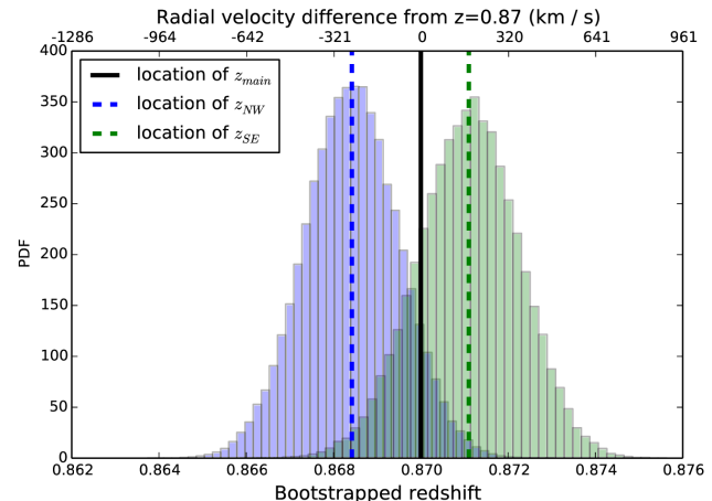
Figure 4. Bootstrapped location of the redshift estimates and v_{rad} estimates for each subcluster using the selected spectroscopic members. The shaded histograms represent the bootstrapped samples.
