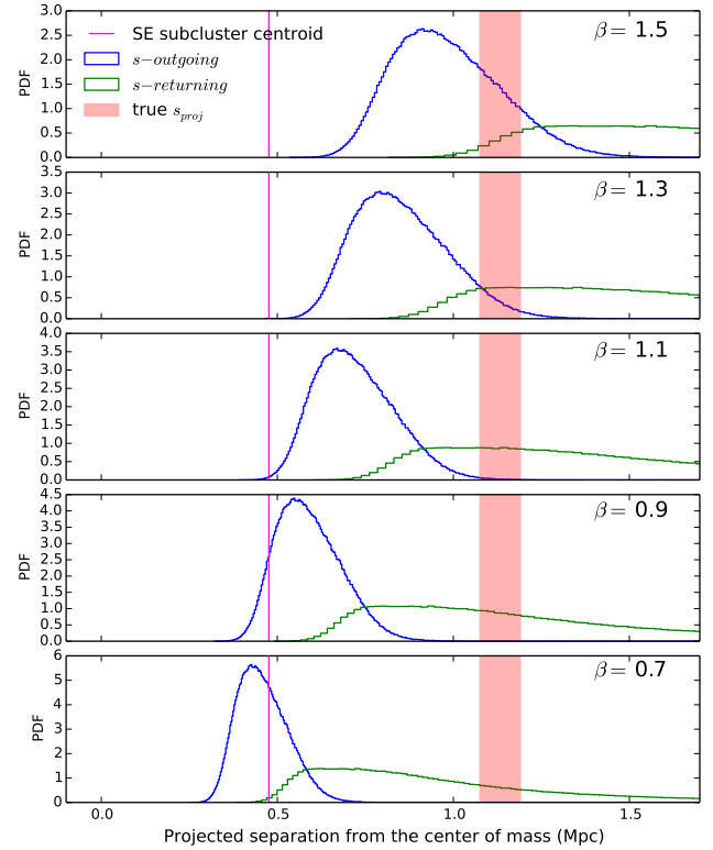
Figure C2. Comparison of the PDFs of the observed position of the SE relic (red bar includes 95% confidence interval of location of relic in the center of mass frame) with the predicted position from the two simulated merger scenarios (blue for outgoing and green for the returning scenario). For the plausible values of \beta < 1.1 , the returning scenario is preferred. We obtained similar conclusion about the merger scenario as for the NW relic calculation.
